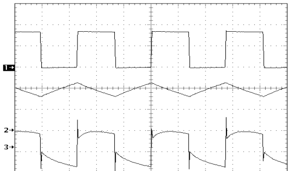
Figure 52. NCP1450ASN19T1 Operating Waveforms (Heavy Load)
