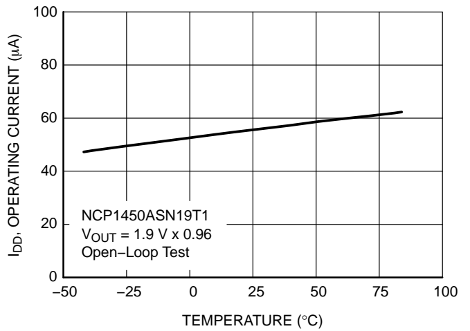
Figure 12. NCP1450ASN19T1 Operating Current vs. Temperature
