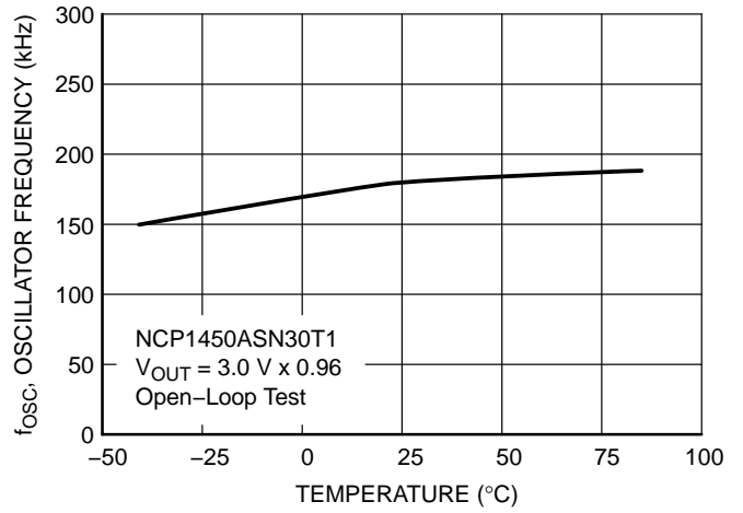
Figure 22. NCP1450ASN30T1 Oscillator Frequency vs. Temperature
