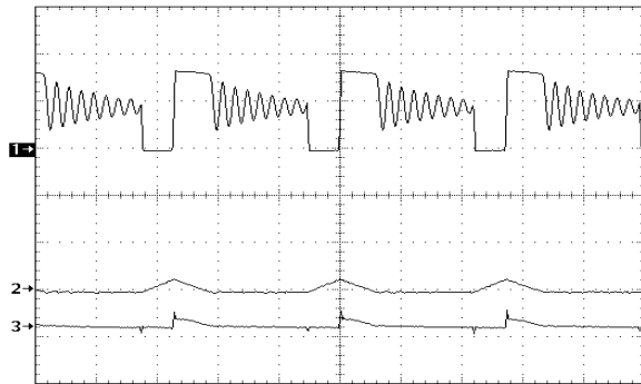
Figure 51. NCP1450ASN19T1 Operating Waveforms (Medium Load)
