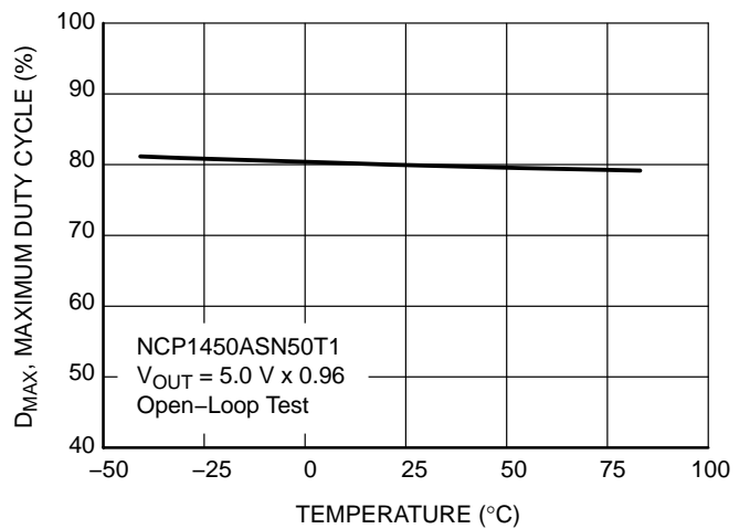
Figure 26. NCP1450ASN50T1 Maximum Duty Cycle vs. Temperature
