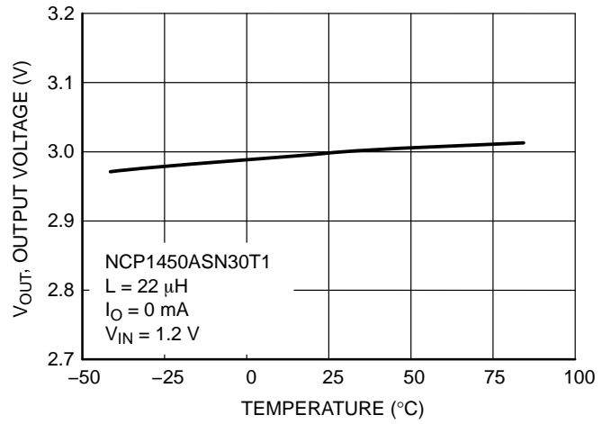
Figure 10. NCP1450ASN30T1 Output Voltage vs. Temperature
