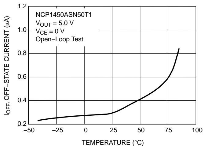
Figure 20. NCP1450ASN50T1 Off-State Current vs. Temperature
