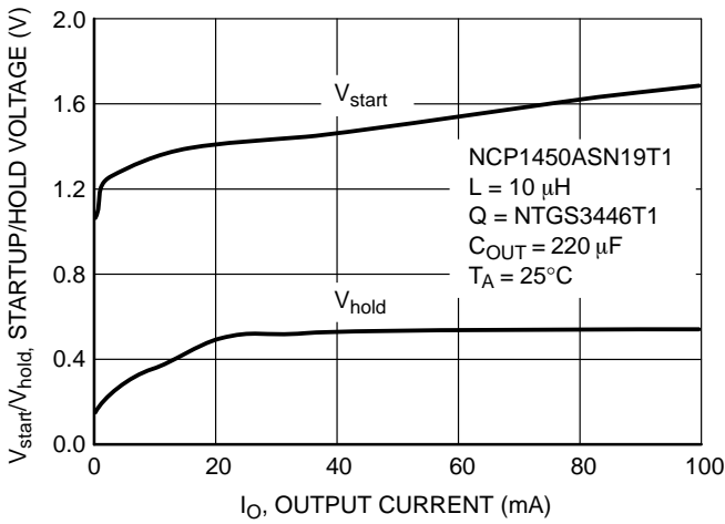
Figure 45. NCP1450ASN19T1 Startup/Hold Voltage vs. Output Current (Using MOSFET)
