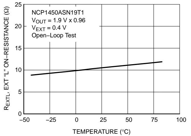
Figure 36. NCP1450ASN19T1 EXT "L" ON-Resistance vs. Temperature
