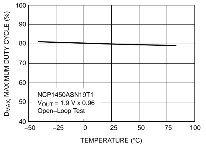
Figure 24. NCP1450ASN19T1 Maximum Duty Cycle vs. Temperature
