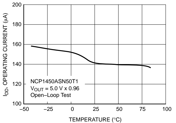
Figure 14. NCP1450ASN50T1 Operating Current vs. Temperature
