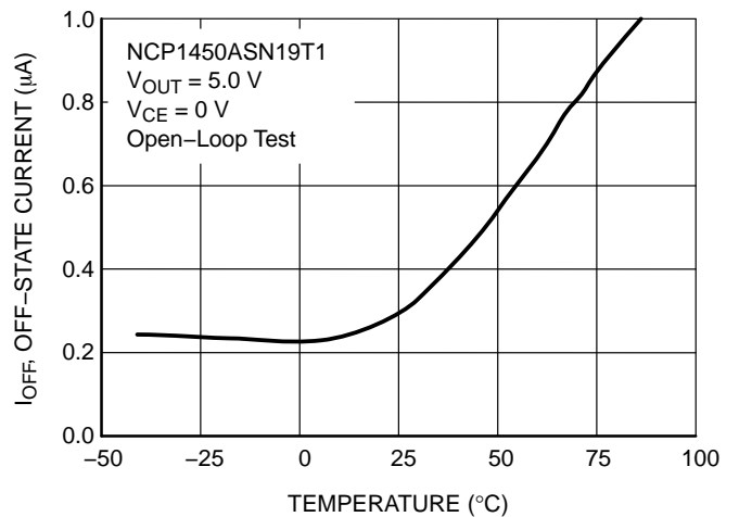
Figure 18. NCP1450ASN19T1 Off-State Current vs. Temperature
