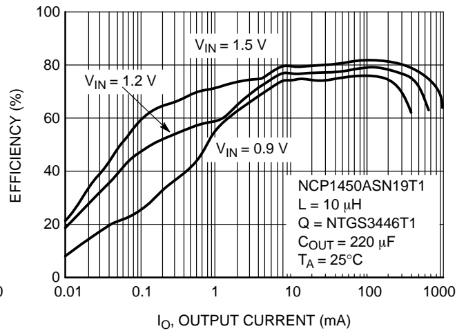
Figure 6. NCP1450ASN19T1 Efficiency vs. Output Current
