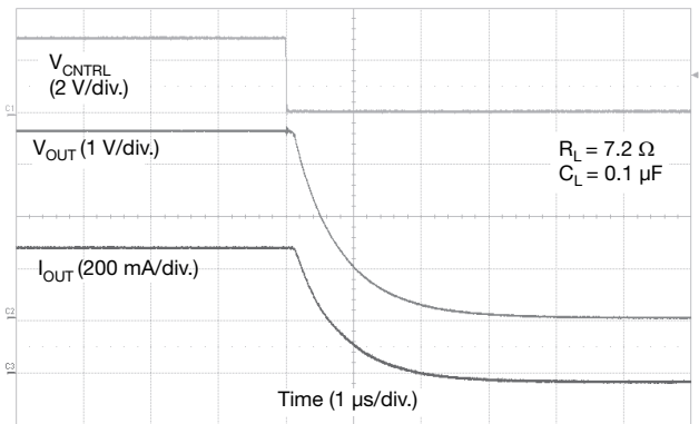
Figure 33 - SiP32416 Turn-Off ( V_{IN} = 3.6\text{ V} , R_L = 7.2\ \Omega )
