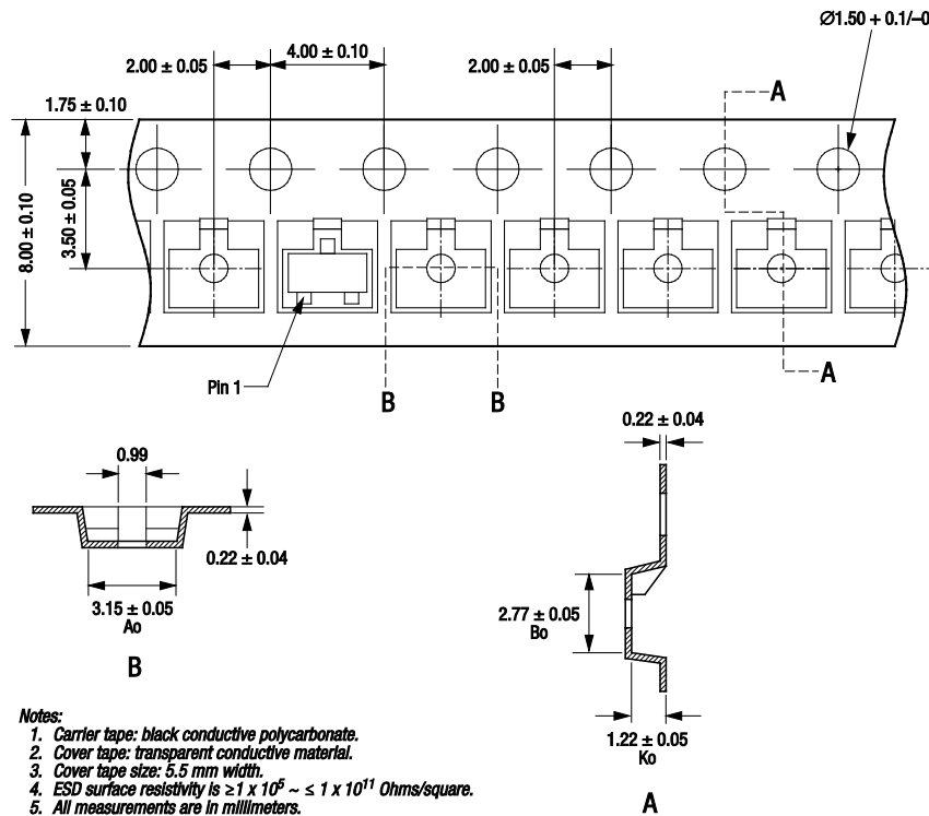
Figure 15. SOT-23 Tape and Reel Dimensions
