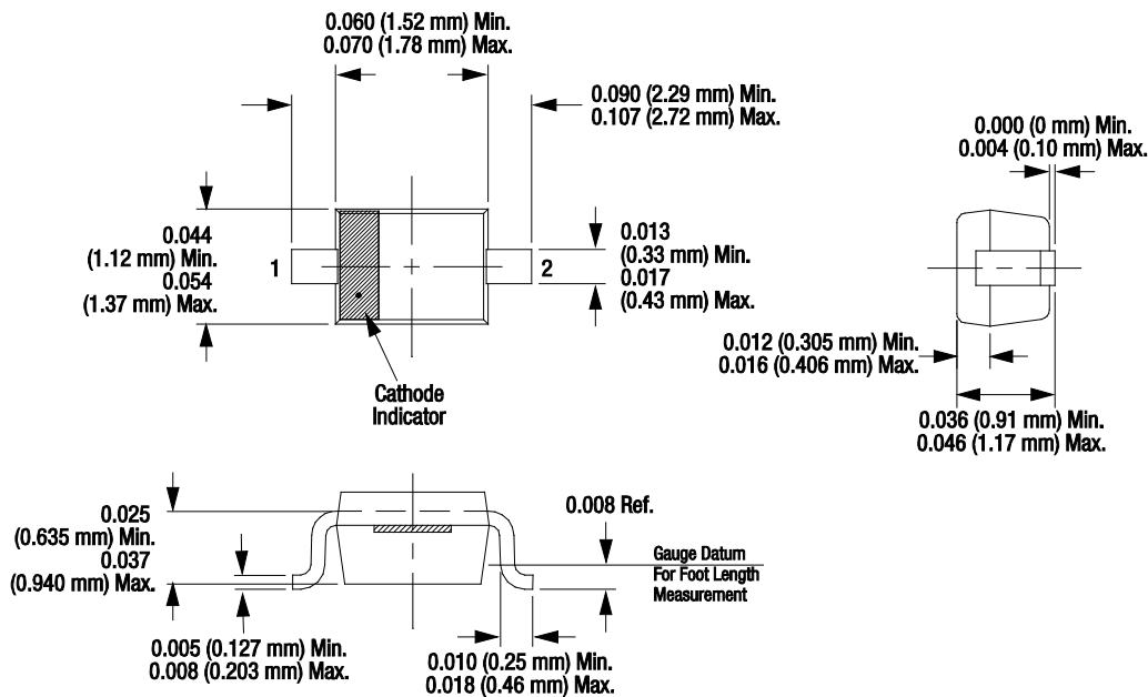
Figure 12. SOD-323 Package Dimension Drawing
