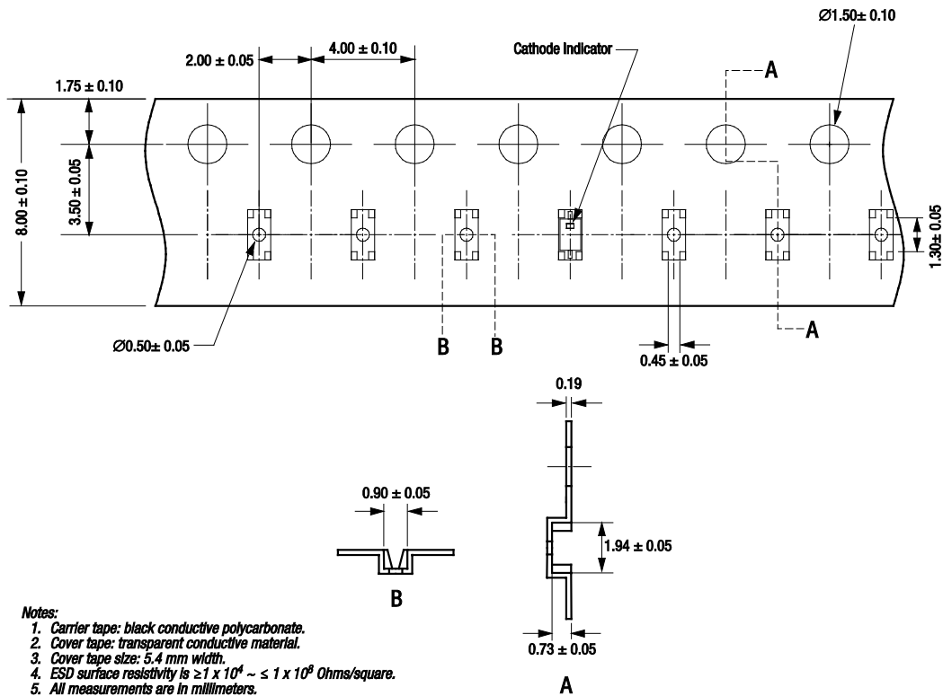
Figure 11. SC-79 Tape and Reel Dimensions
