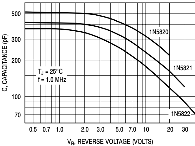
Figure 10. Typical Capacitance
