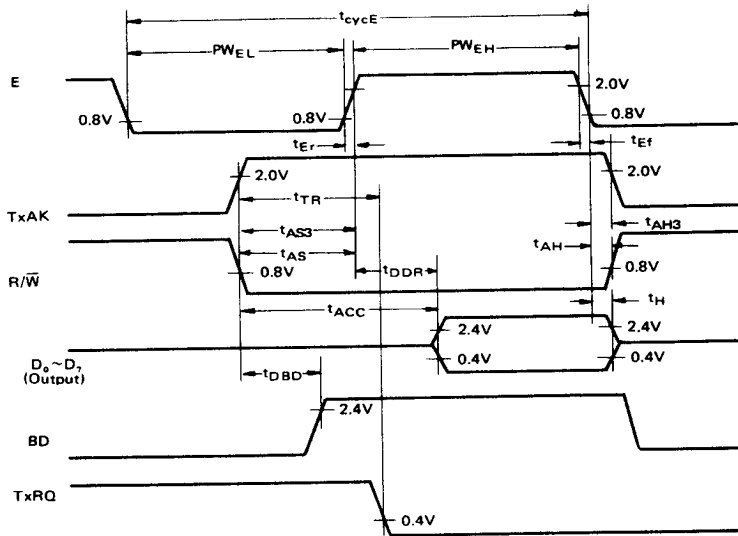
Figure 10 DMA Read Timing
