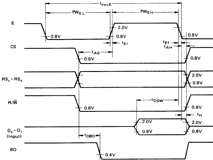
Figure 9 Write Timing
