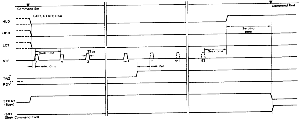
Figure 23 Timing Sequence of STZ Command
