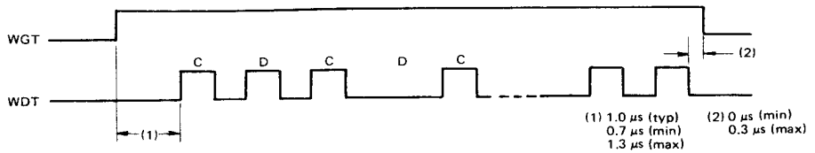
Figure 17 Write Data versus Write Gate Timing
