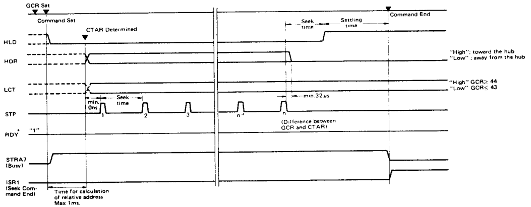
Figure 24 Timing Sequence of SEK Command
