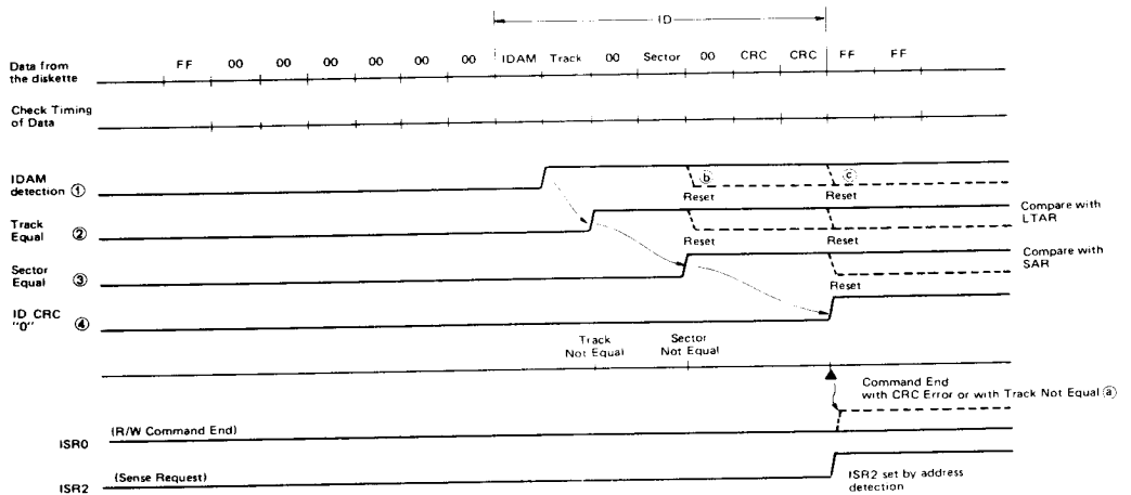
Figure 25 Timing Sequence of SSR, SSW, RCR, SWD, MSR, MSW Command (Relation with HLD and IDX)
