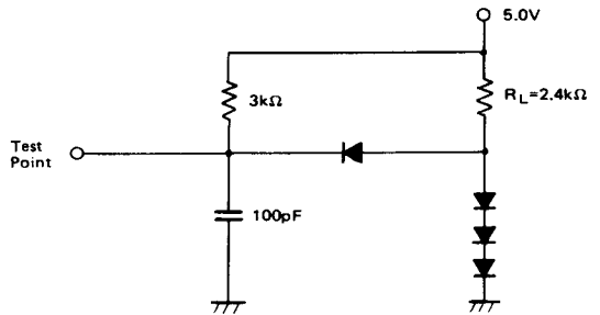
LOAD B ( \overline{IRQ} )
