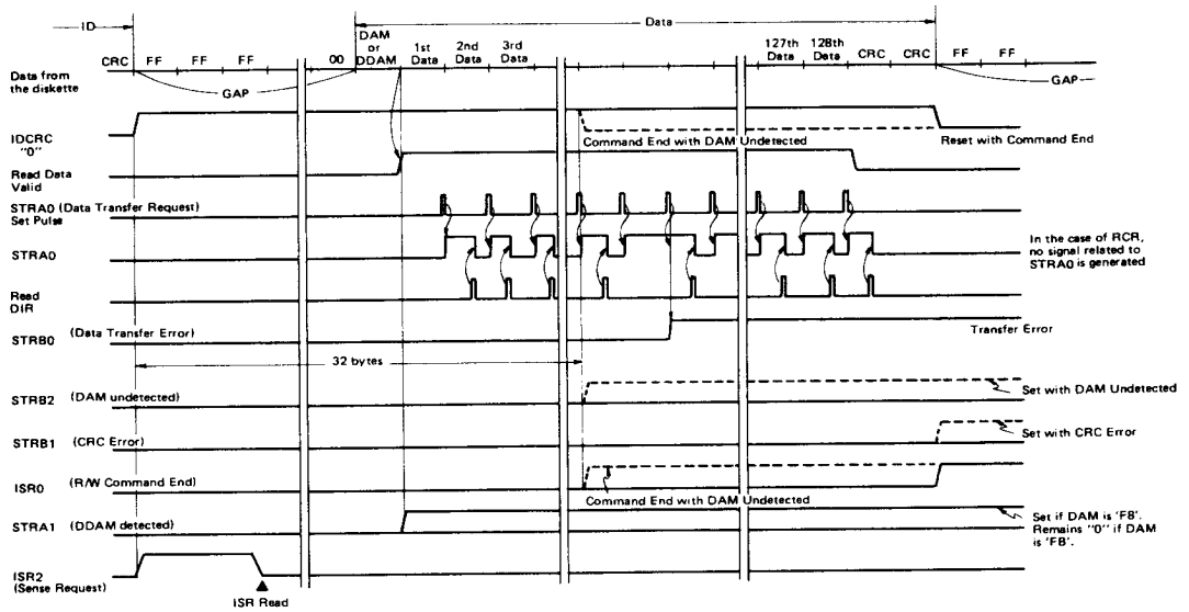
Figure 27 Data Transfer Timing of SSR, RCR Command
