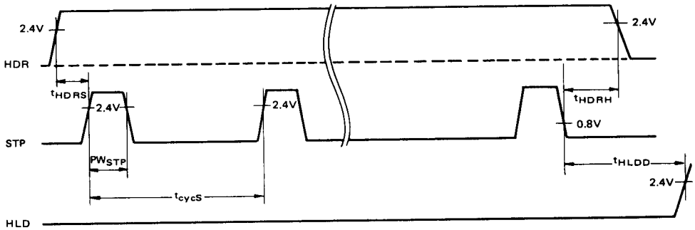
Figure 5 Seek Operation Sequence
