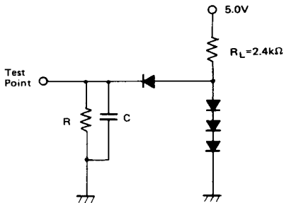
LOAD A (Except \overline{IRQ} )
