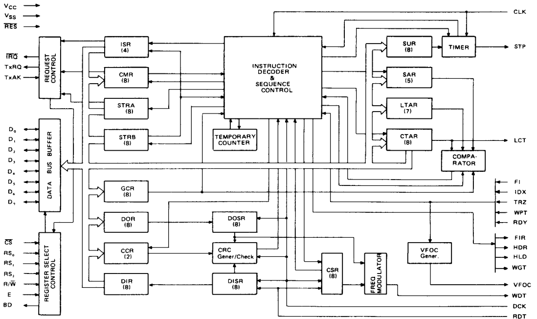
Figure 13 Block Diagram of the FDC
