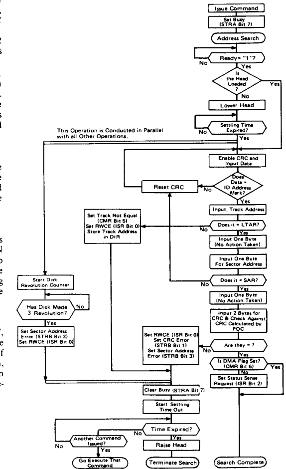
Figure 20 Operational Flow of the Address Search Sequence
