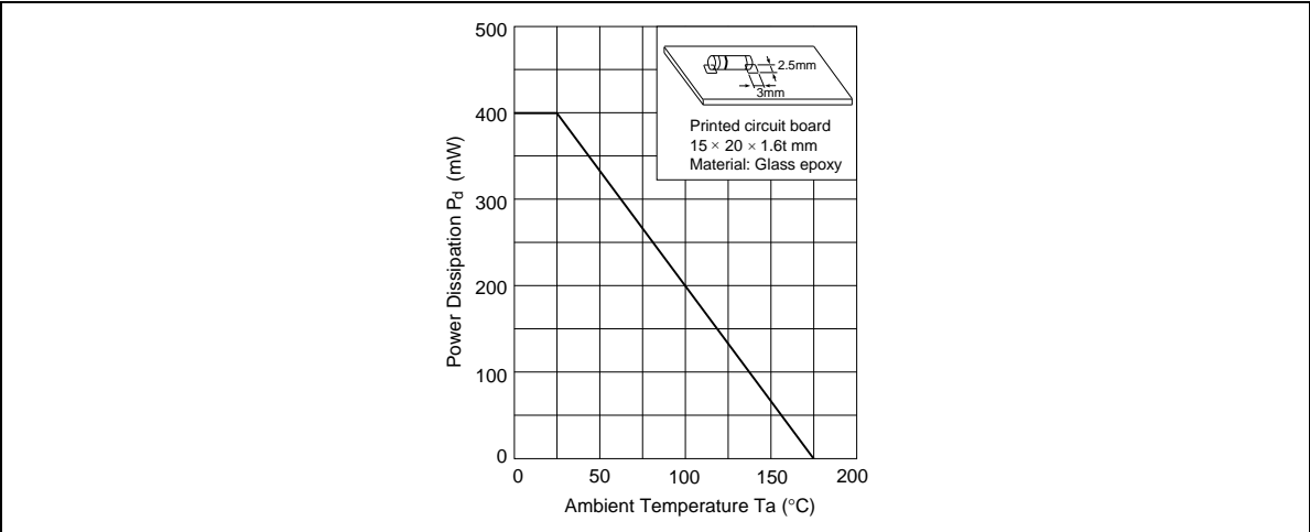
Fig.3 Power Dissipation Vs. Ambient Temperature
