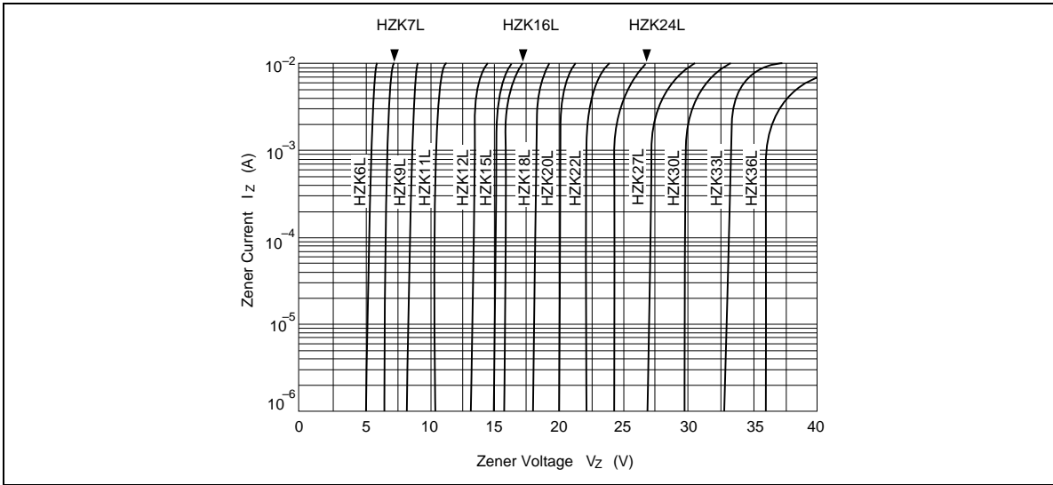
Fig.1 Zener current Vs. Zener voltage
