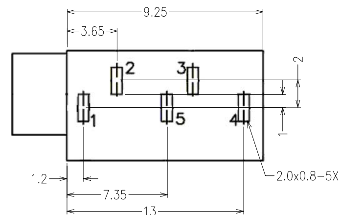
DIMENSIONS OF PCB BOARD HOLES TOLERANCE ±0.1 (TOP VIEW)
