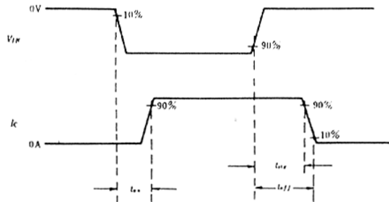
RESPONSE WAVEFORM
