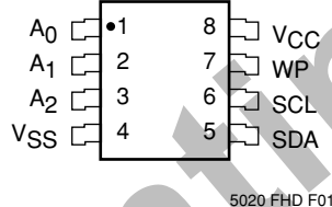
SOIC Package (J, W)
