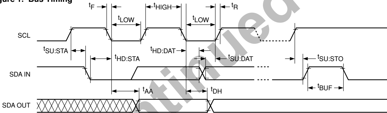
Figure 1. Bus Timing
