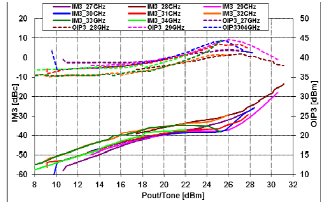
@Vds=5V, Idsq=3A
