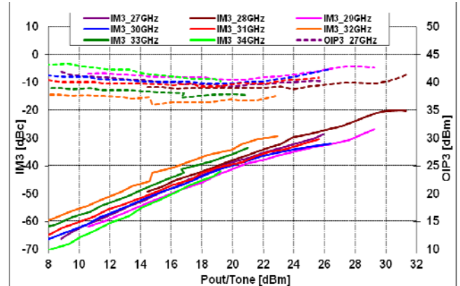
@Vds=6V, Idsq=2.5A
