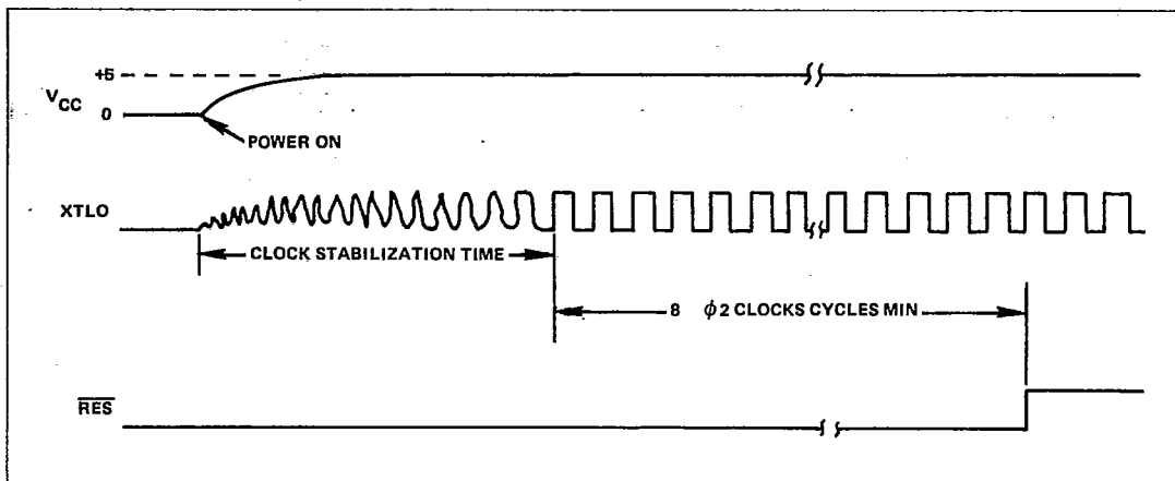
Figure 4-1. Power Turn-On Timing Detail
