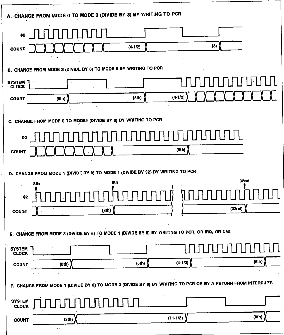
Figure 3-7. Prescaler Waveform Examples
