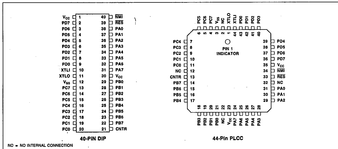
Figure 2-2. R65C10 Pin Assignments
