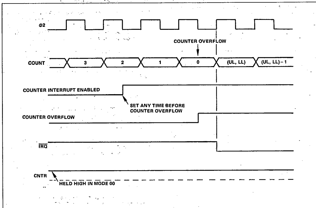
Figure 3-10. Interval Timer (Mode 0) Timing Waveforms
