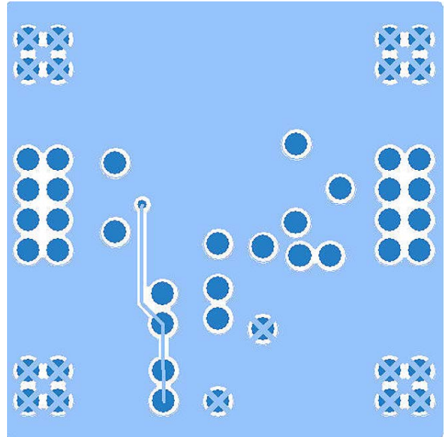
Figure 48. Typical Board Layout, Bottom Side
