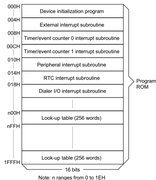
Program memory
