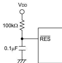
Reset circuit
