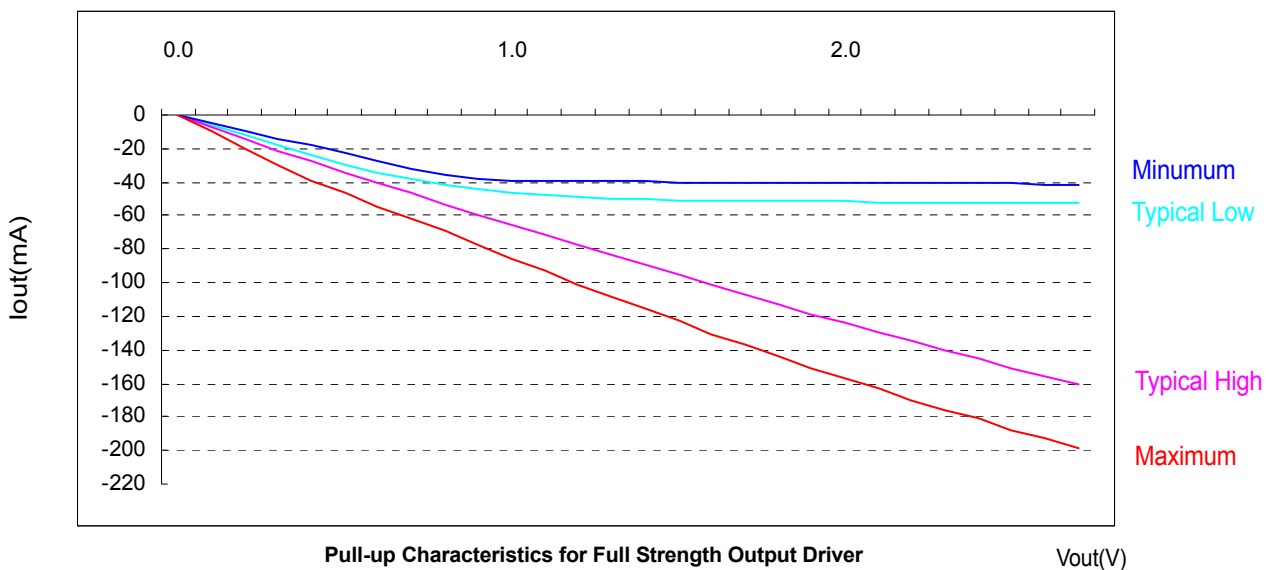
Figure 8. I/V characteristics for input/output buffers : Pull-down(above) and Pull-up(below)
