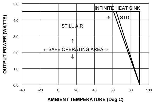
5 WATT DUAL SERIES POWER DERATING
