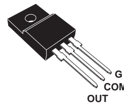
TO-220FPAB ACST4-7SFP/CFP
