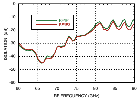
RF/IF Isolation
