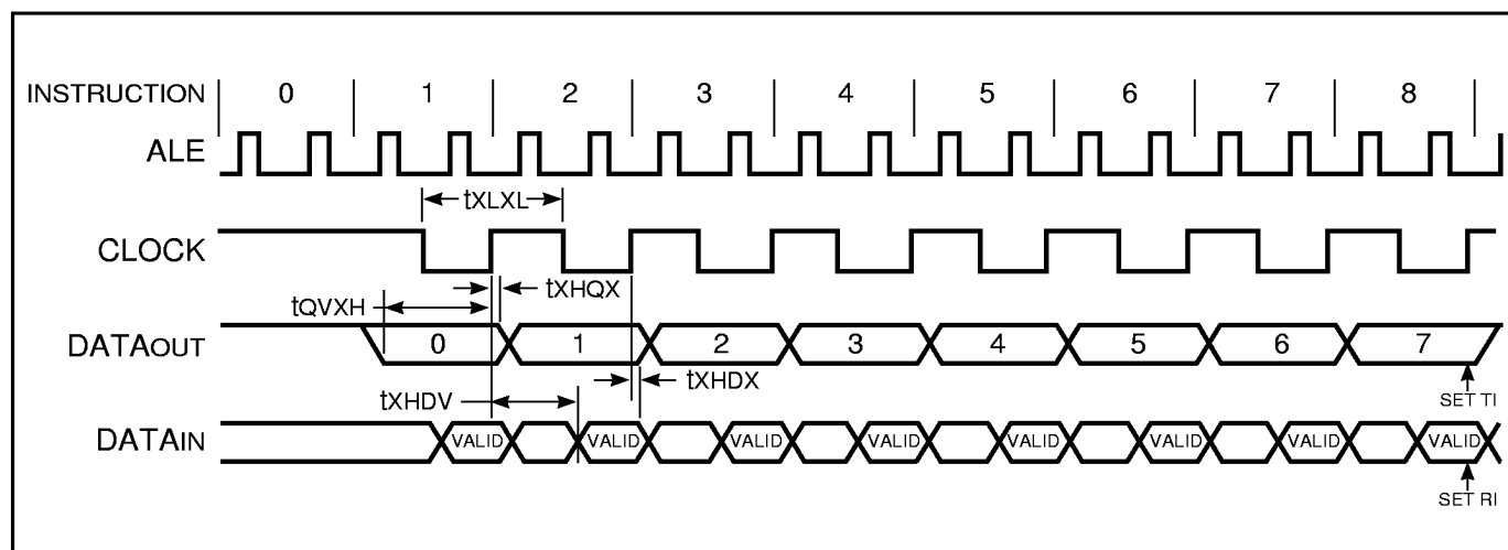
Figure 35. Shift Register Mode Timing Waveform
