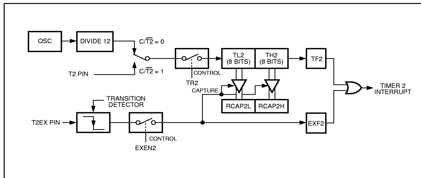
Figure 12. Timer 2 In Capture Mode
