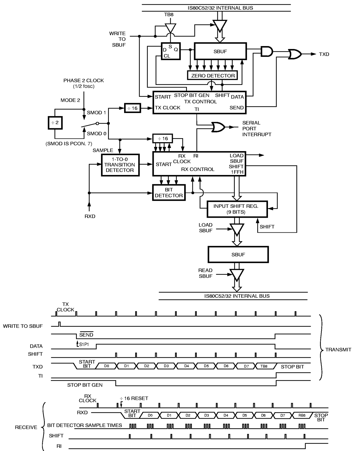
Figure 17. Serial Port Mode 2
