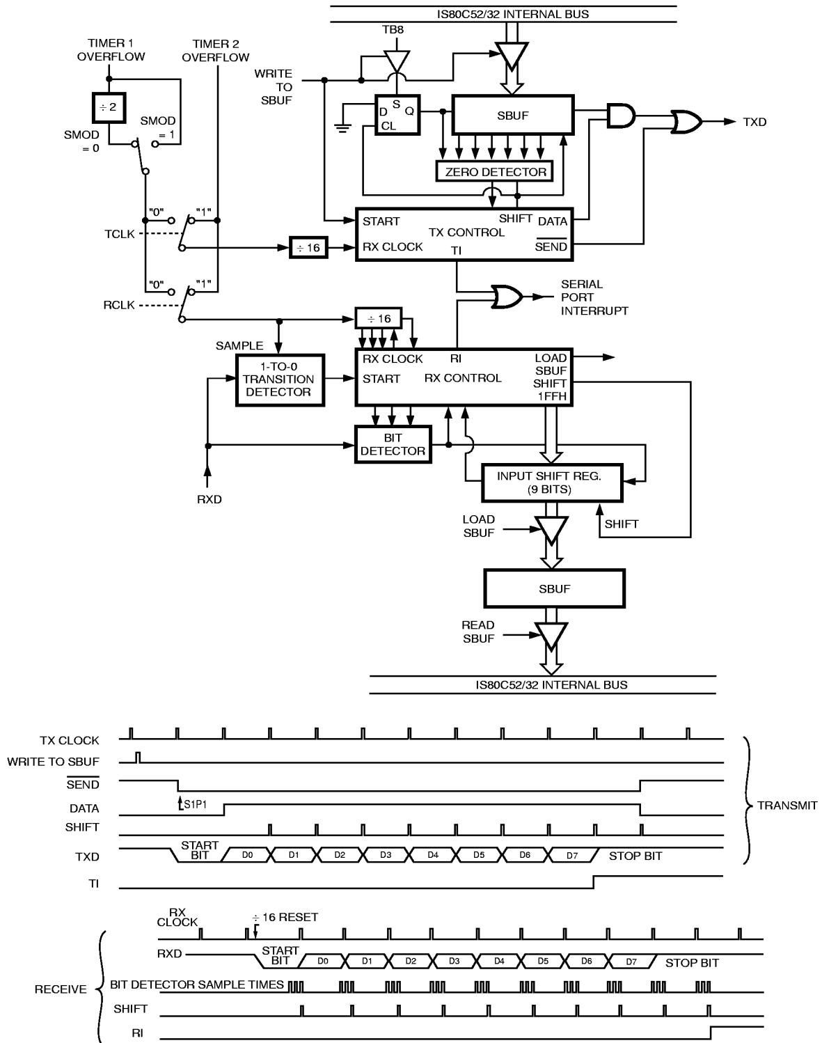
Figure 16. Serial Port Mode 1
