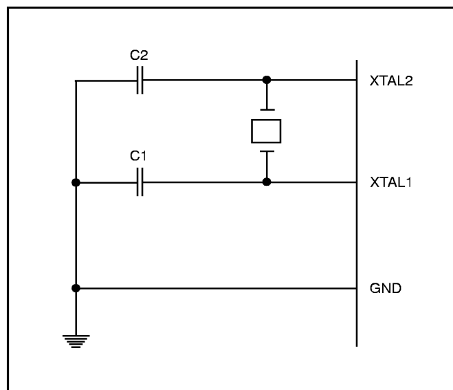
Figure 24. Oscillator Connections
