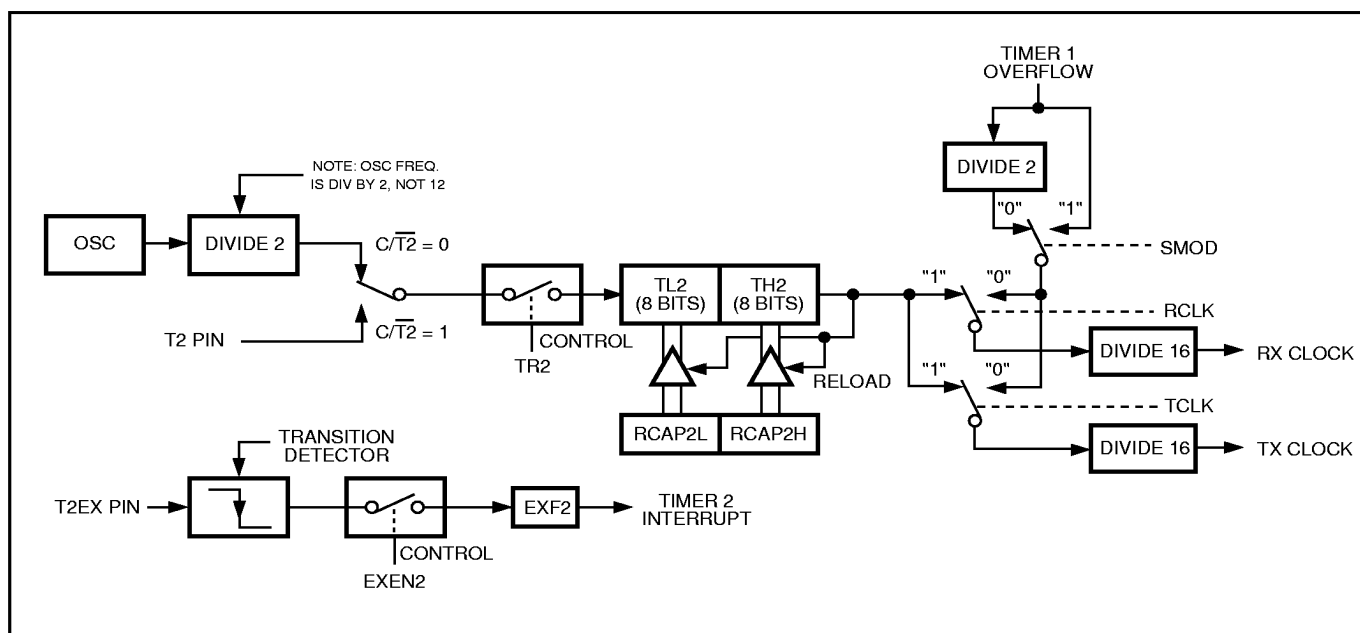
Figure 14. Timer 2 in Baud Rate Generator Mode
