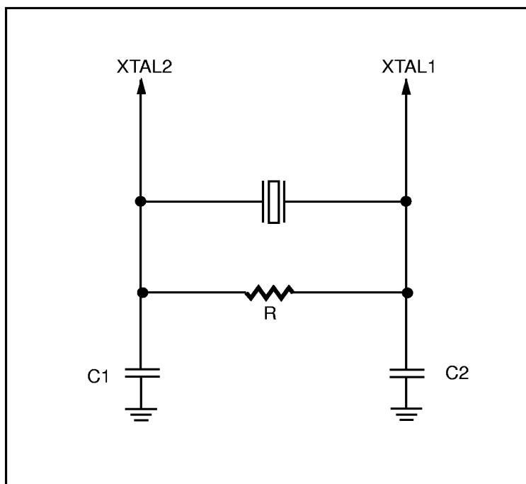
Figure 26. For High Speed (> 24 MHz)
