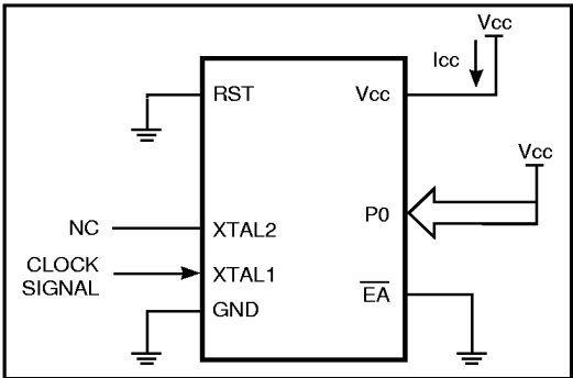
Figure 29. Idle Mode
