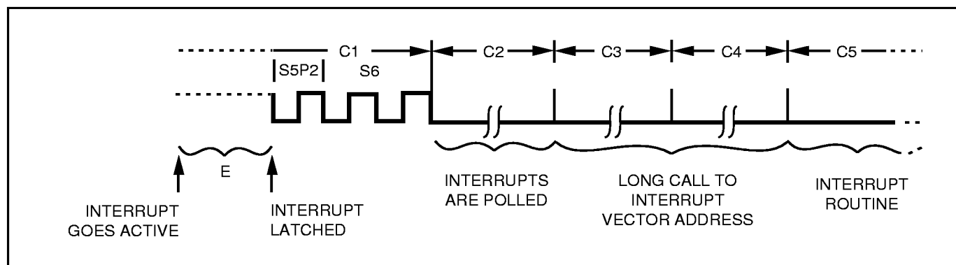
Figure 20. Interrupt Response Timing Diagram
