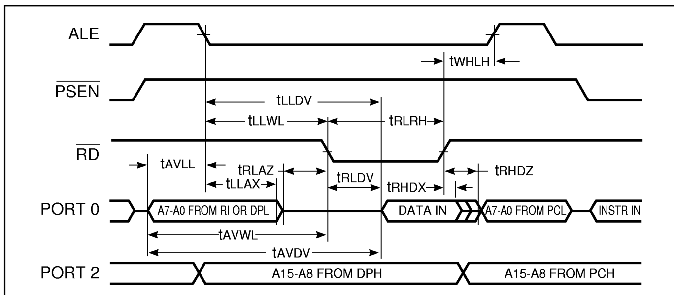
Figure 33. External Data Memory Read Cycle
