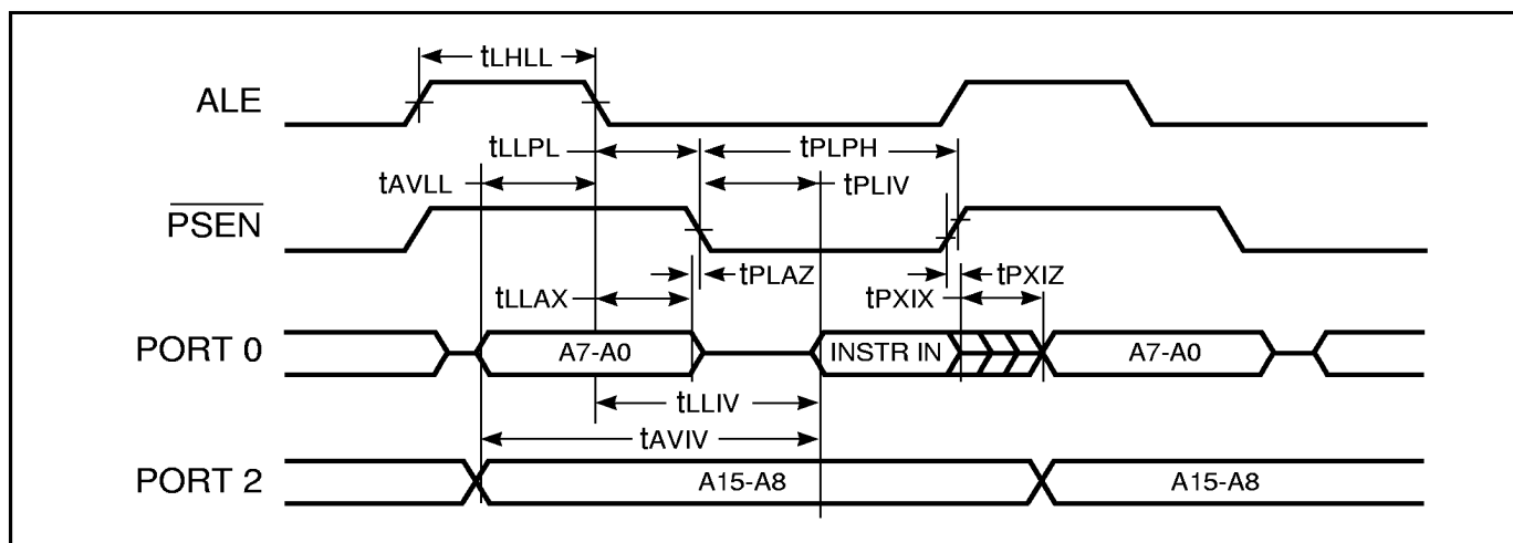
Figure 32. External Program Memory Read Cycle
