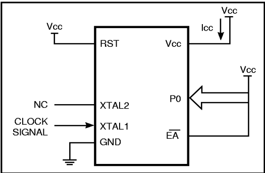
Figure 28. Active Mode
