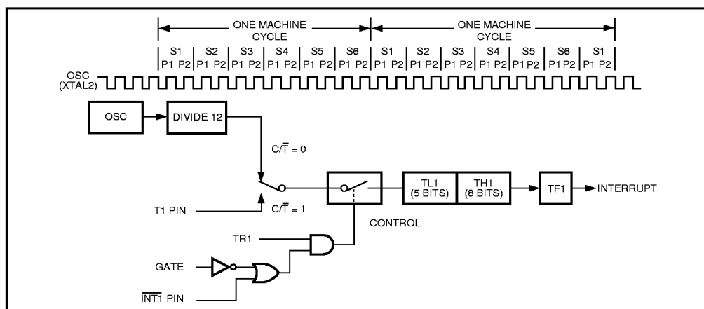
Figure 8. Timer/Counter 1 Mode 0: 13-Bit Counter
