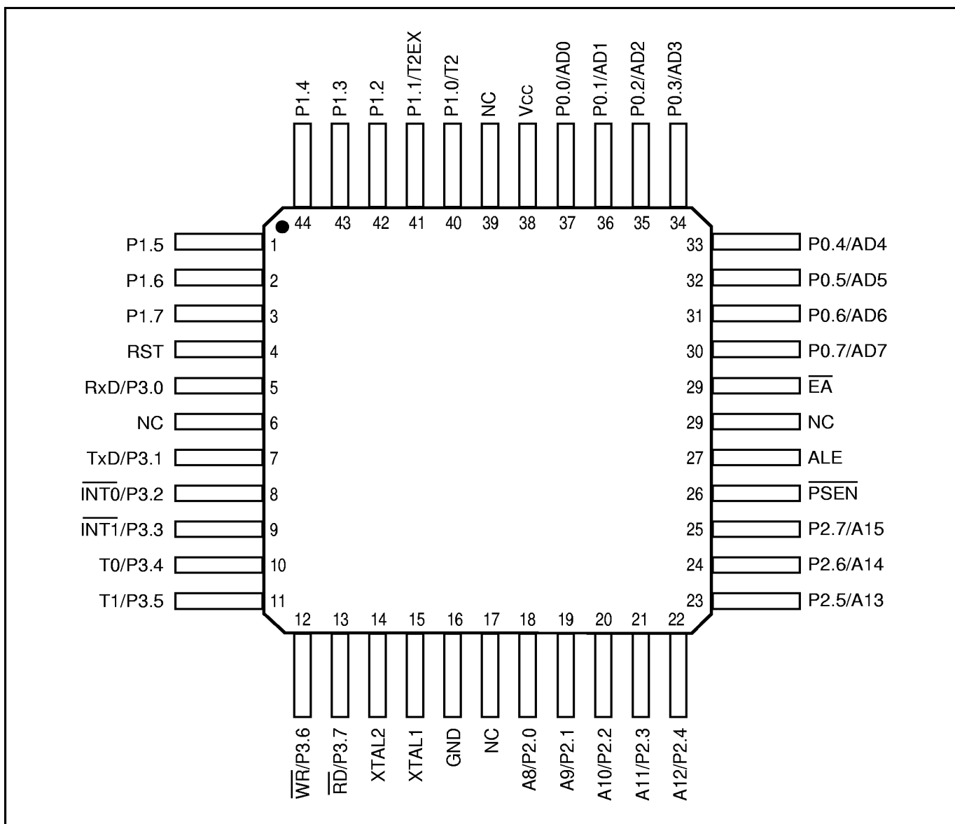
Figure 3. IS80C52/32 Pin Configuration: 44-pin PQFP
