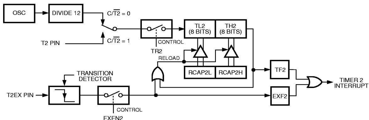
Figure 13. Timer 2 in Auto-Reload Mode
