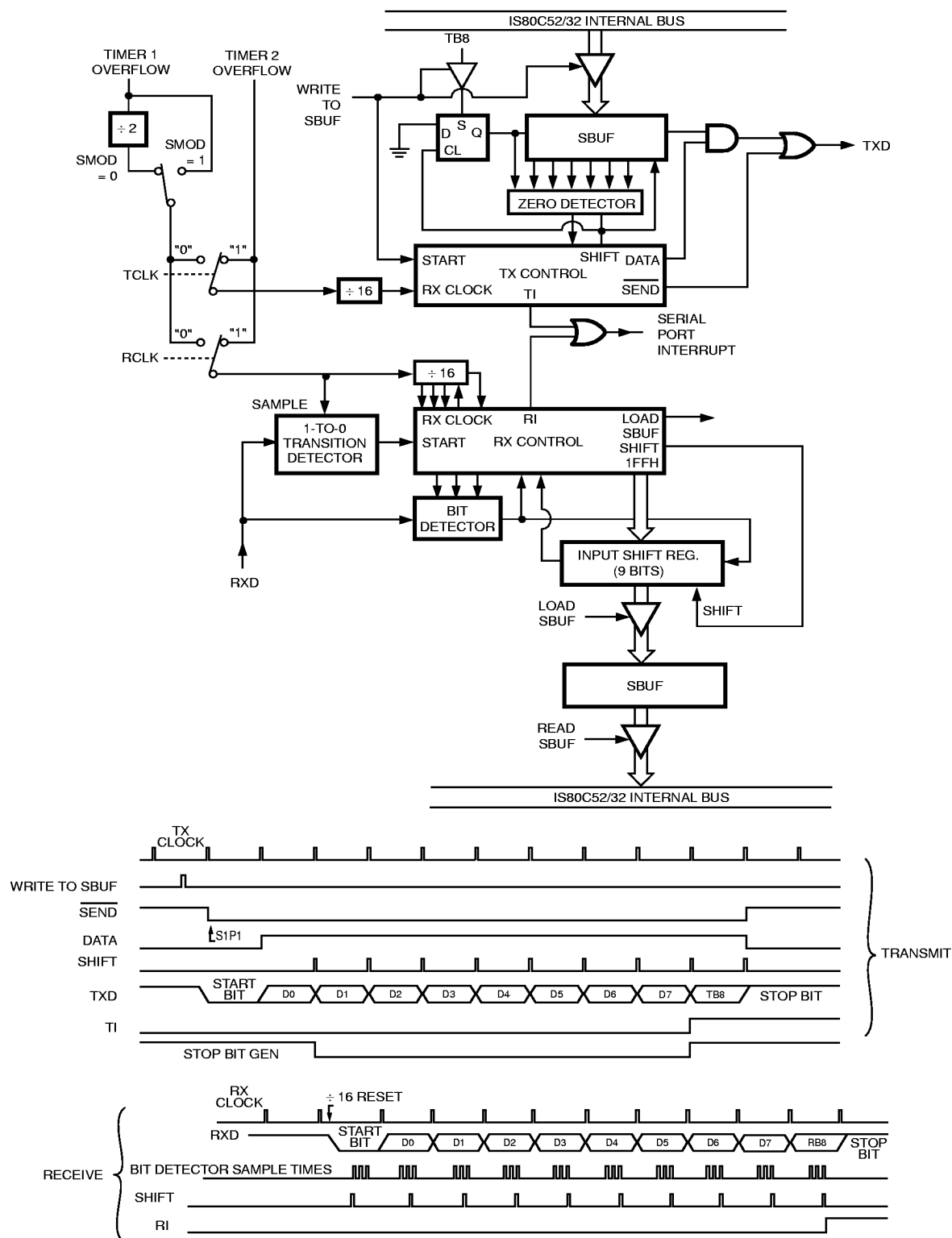
Figure 18. Serial Port Mode 3
