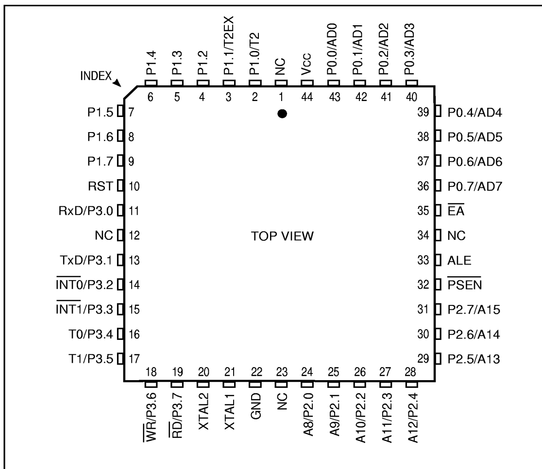
Figure 2. IS80C52/32 Pin Configuration: 44-pin PLCC
