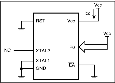
Figure 30. Power-down Mode
