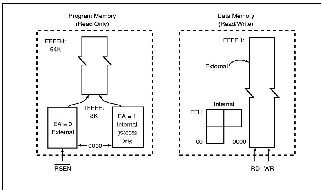
Figure 5. IS80C52/32 Program and Data Memory Structure
