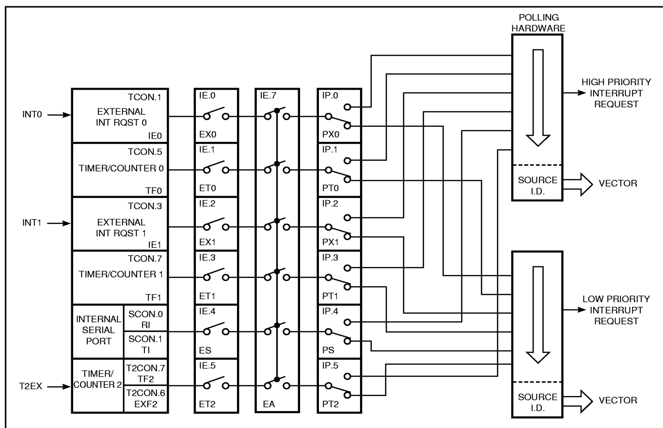
Figure 19. Interrupt System
