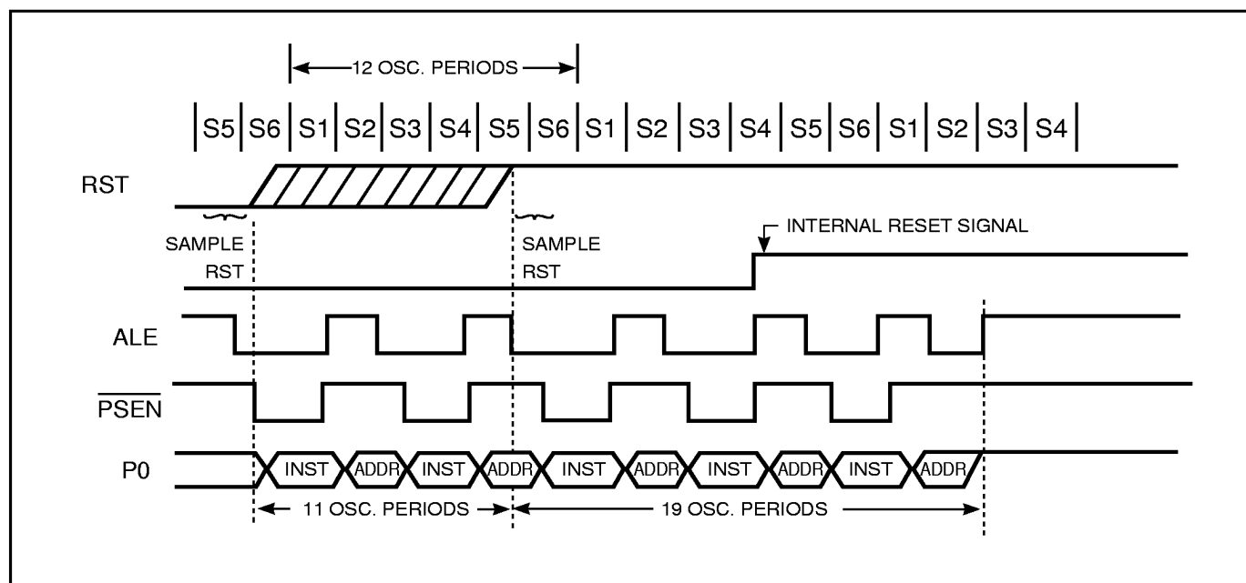
Figure 22. Reset Timing
