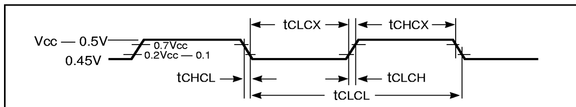
Figure 31. Icc Test Conditions
