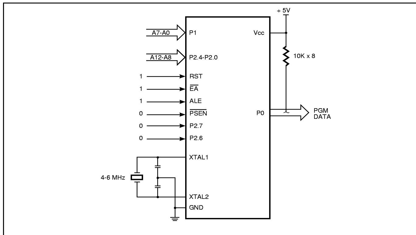
Figure 27. ROM Verification
