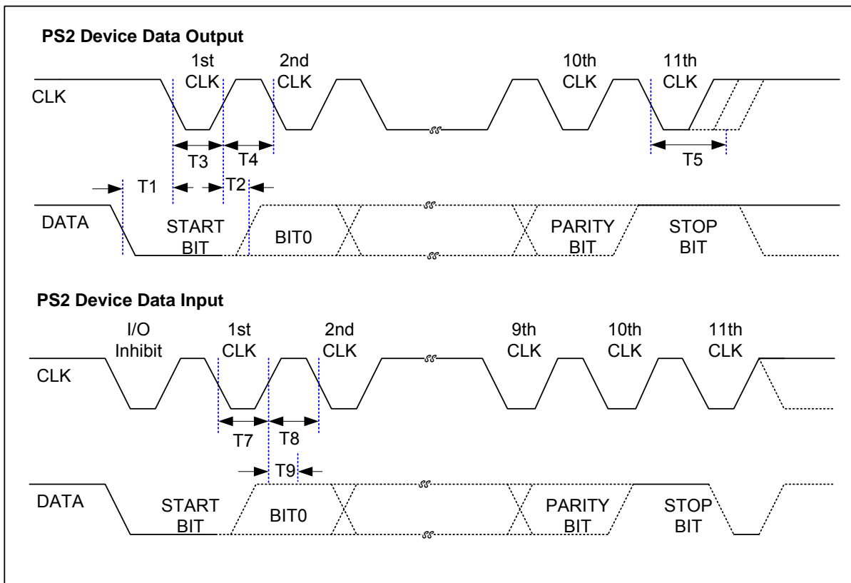
Figure 5-87 PS/2 Bus Timing
