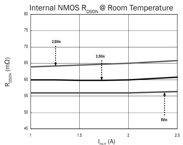
Figure 12. Low-Side N-MOSFET
