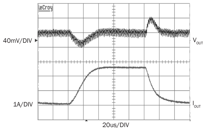
Figure 5. Transient Response @ 0 to 2.5A
