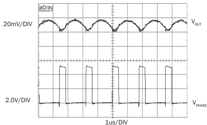
Figure 6. Ripple and Stability @ 2.5A
