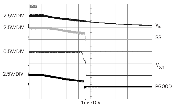
Figure 4. Shutdown by V IN @ 2.5A
