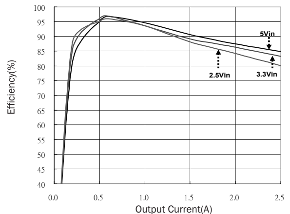
Figure 10. Efficiency( V_{IN} )
