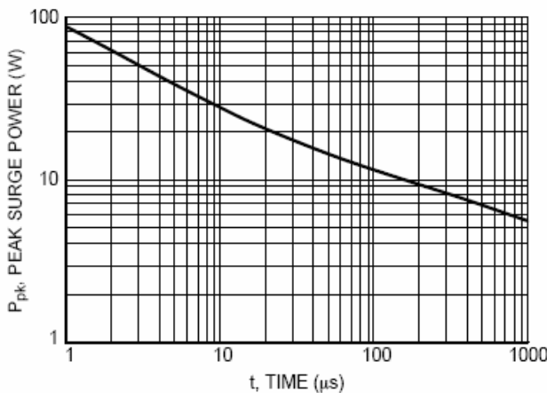
Figure 1 Pulse Width
