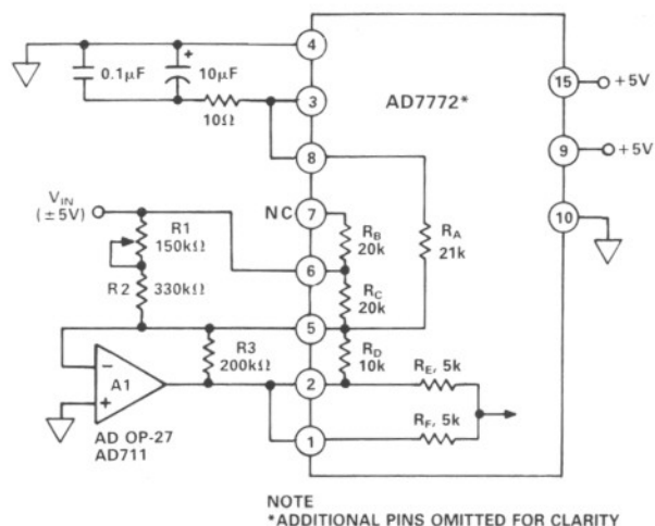
Figure 15. AD7772 Connected for \pm 5V Input Range with Full-Scale Error Adjust
