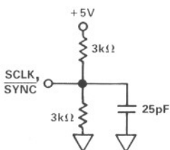
Figure 1. SCLK, SYNC Load Circuit
