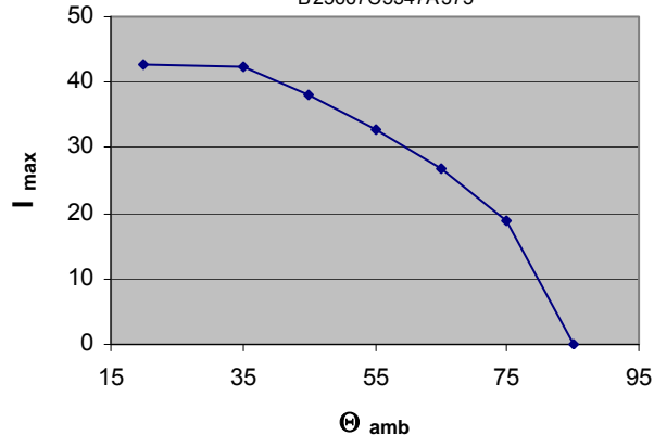
Max. allowable current (rms) at specific ambient Temp. B25667C5347A375
