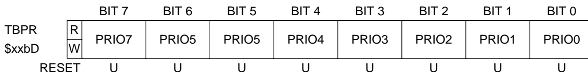
Figure 13. Transmit buffer priority register (TBPR)
