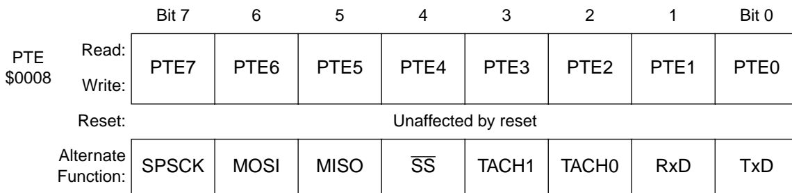
Figure 13. Port E data register (PTE)
