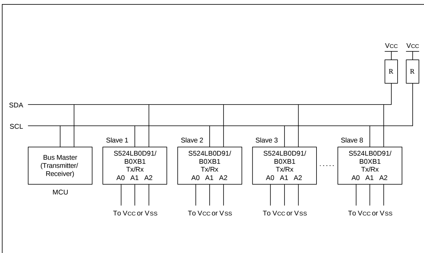
Figure 7-6. Typical Configuration
