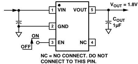
Figure 1. ADP150UJZ-RedyKit
