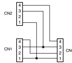
Wiring Diagram
