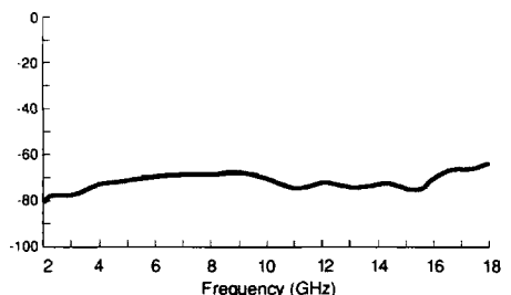
Isolation (dB)
