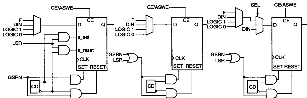
Figure 17. Latch/FF Set/Reset Configurations
