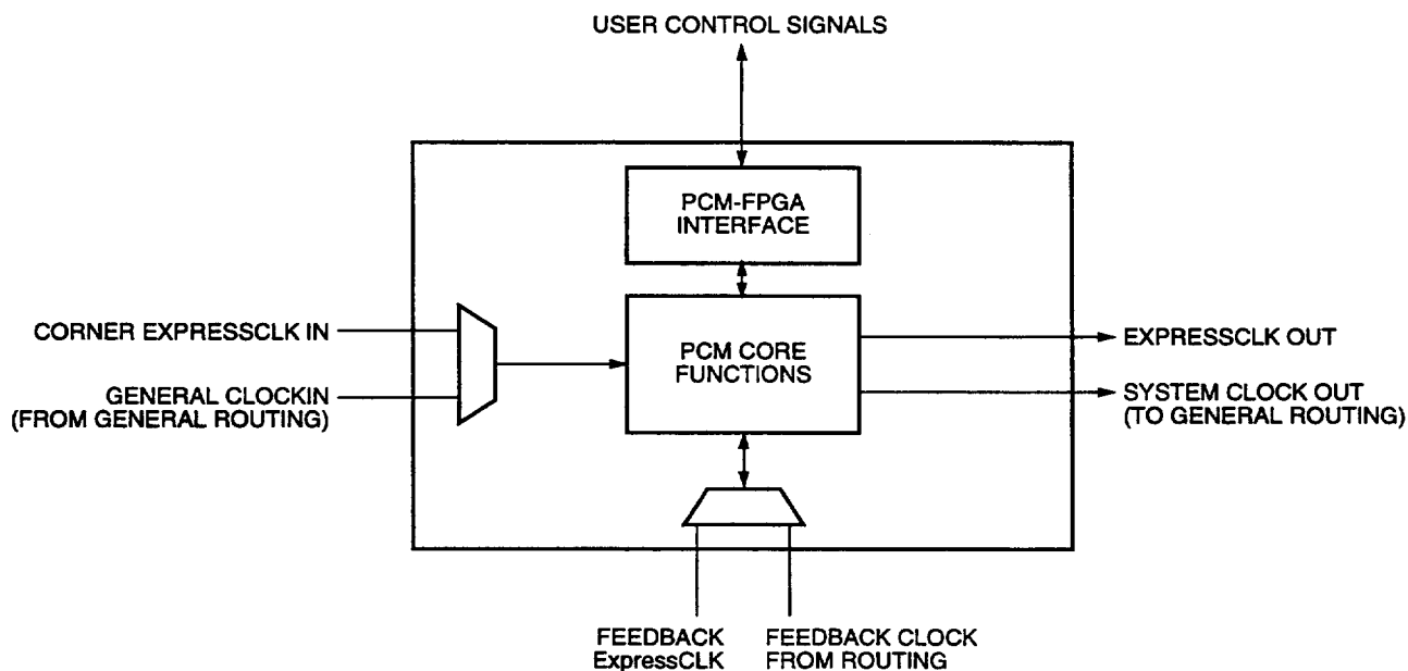
Figure 45. PCM Block Diagram
