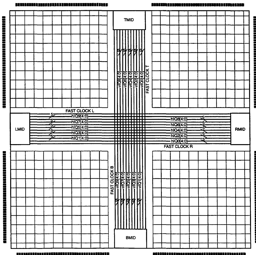
Figure 28. Interquad Routing
