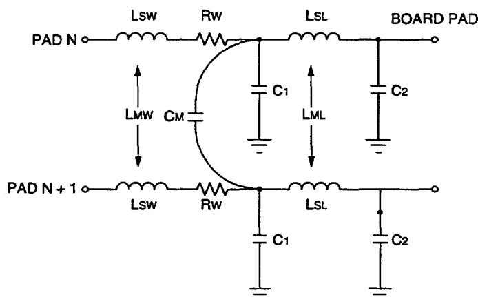
Figure 104. Package Parasitics
