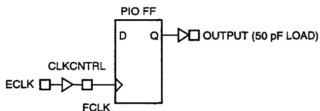
Figure 77. Fast Clock to Output Delay
