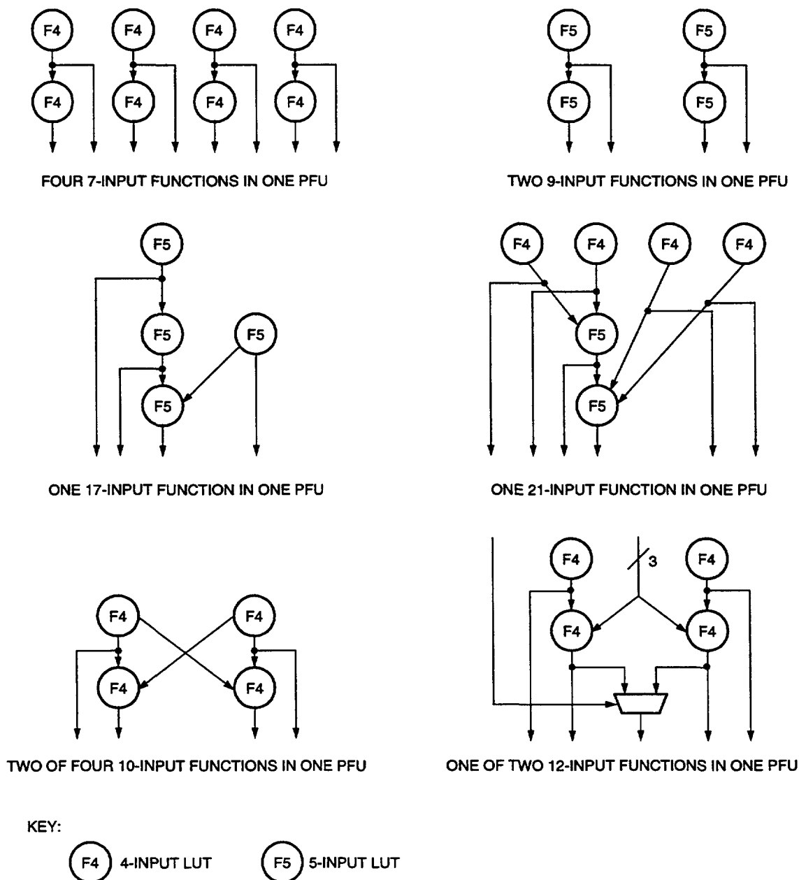
Figure 5. Softwired LUT Topology Examples
