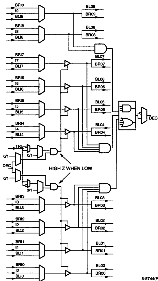
Figure 11. SLIC All Modes Diagram
