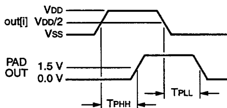
Figure 90. Output Buffer Delays
