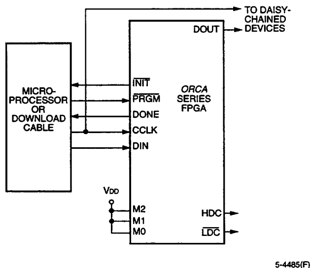
Figure 61. Slave Serial Configuration Schematic
