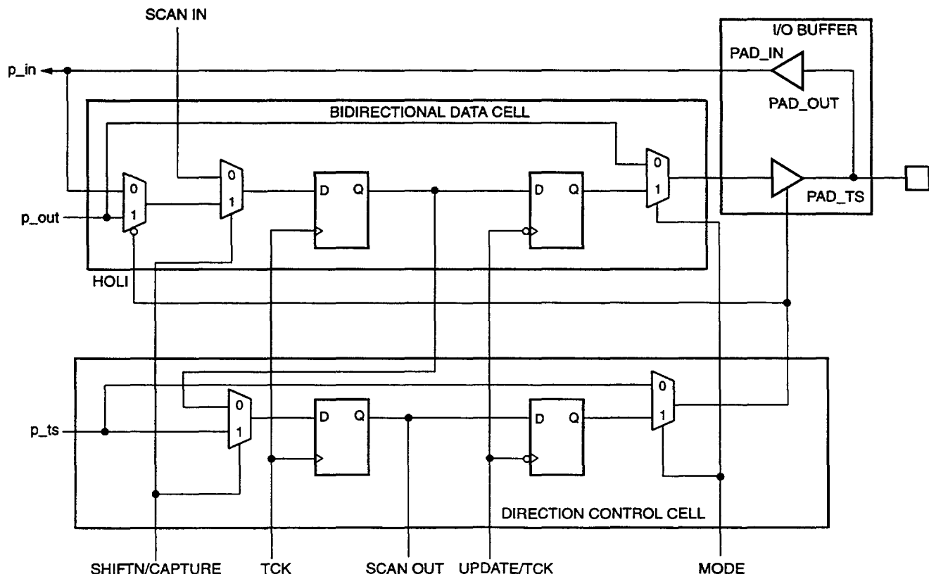
Figure 40. Boundary-Scan Cell
