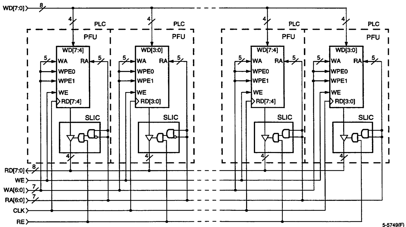
Figure 10. Memory Mode Expansion Example—128 x 8 RAM
