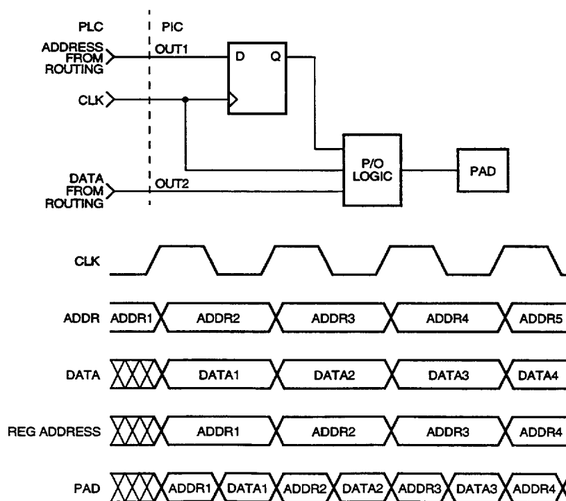
Figure 26. Output Multiplexing (OUT2OUTREG Mode)
