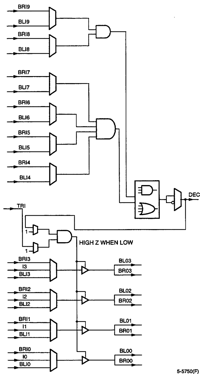
Figure 15. Buffer-Decoder-Decoder Mode
