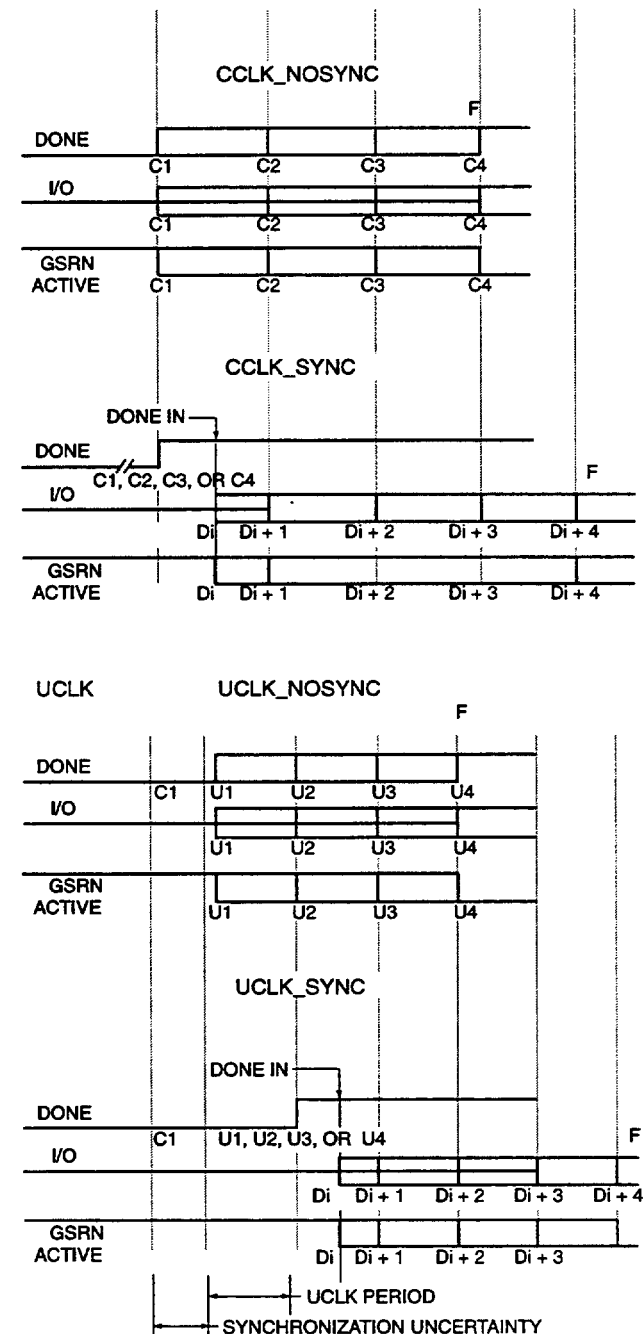
Figure 51. Start-Up Waveforms
