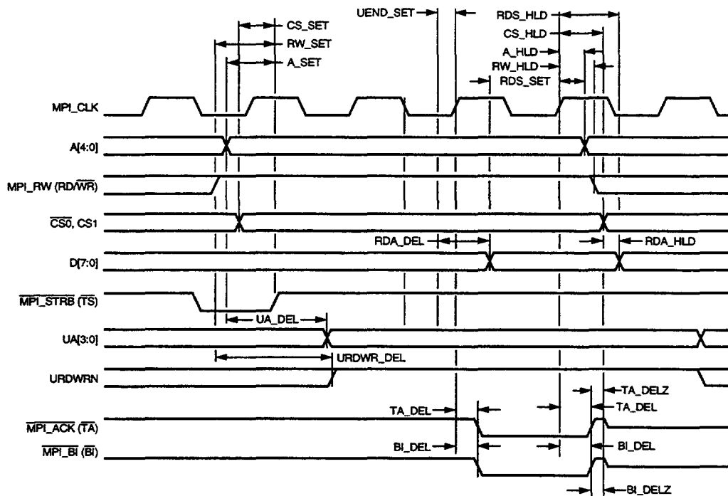
Figure 69. MPI PowerPC Internal Read Timing
