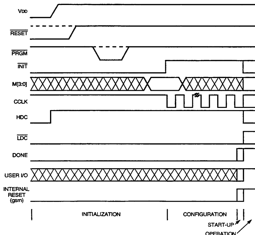
Figure 50. Initialization/Configuration/Start-Up Waveforms
