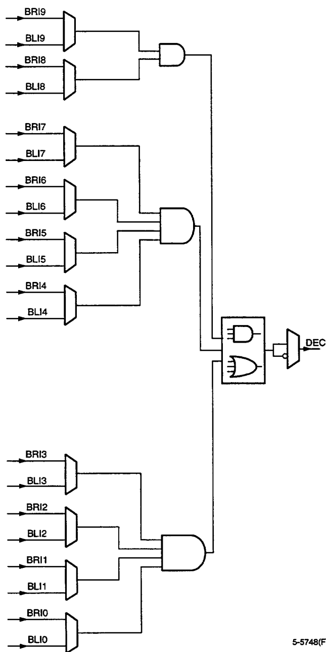
Figure 16. Decoder Mode
