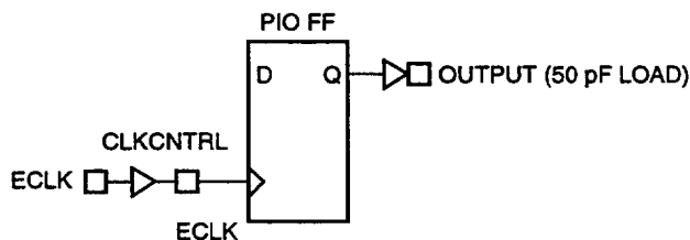
Figure 76. ExpressCLK to Output Delay
