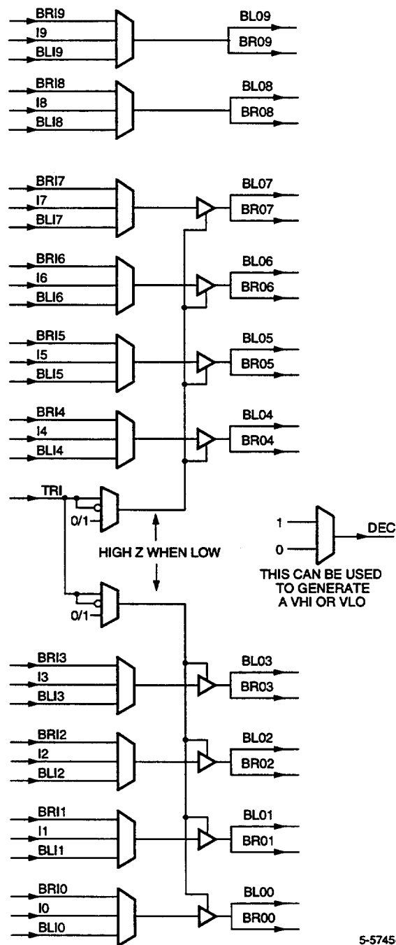
Figure 12. Buffer Mode
