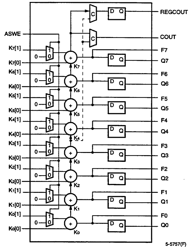
Figure 8. Multiplier Submode
