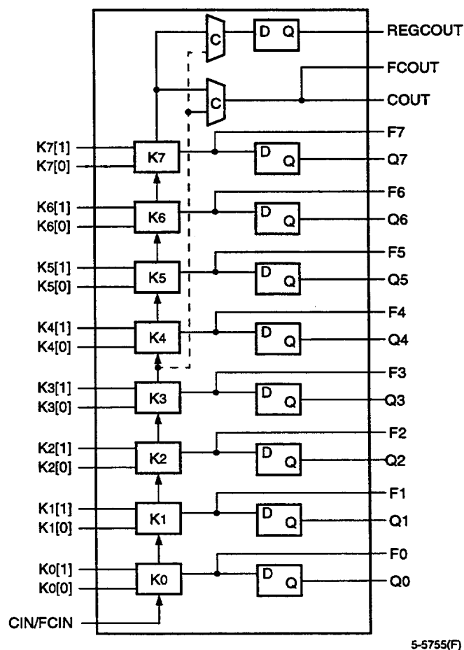
Figure 6. Ripple Mode
