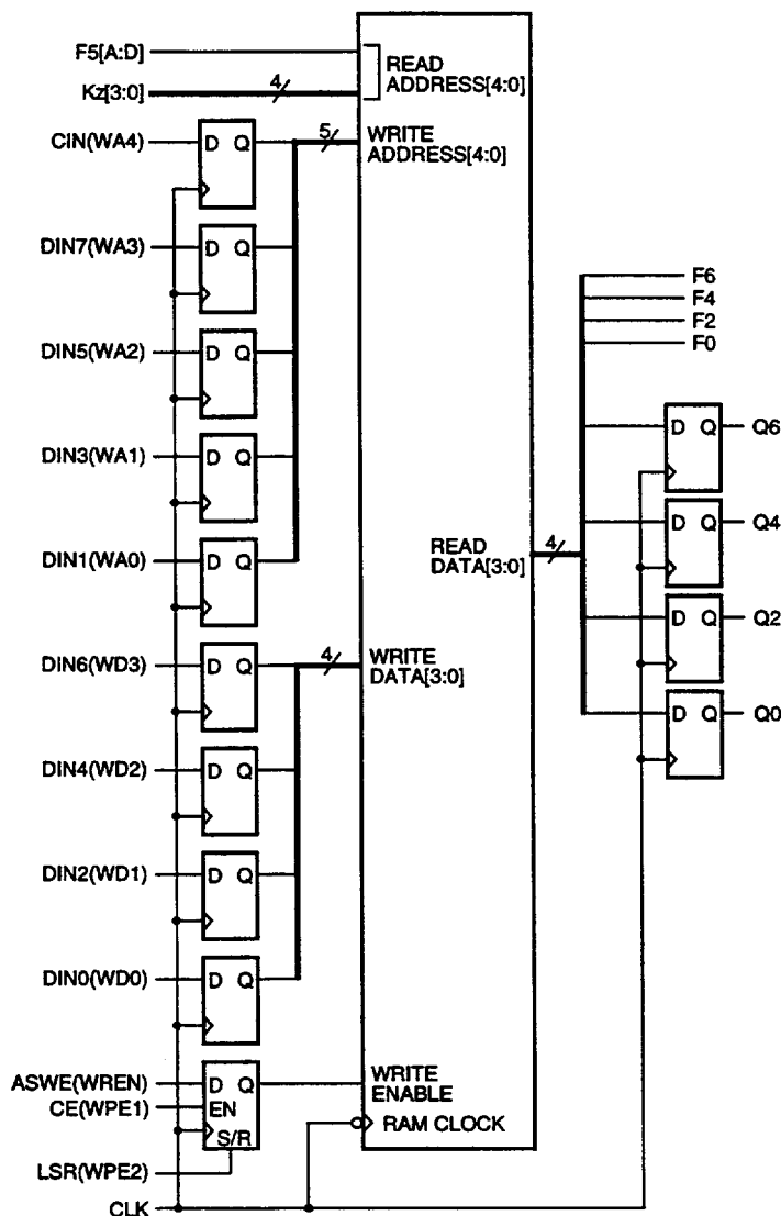
Figure 9. Memory Mode
