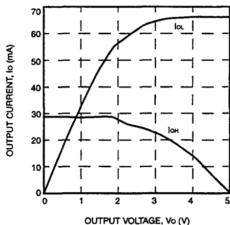
Figure 92. Sinklim ( T_J = 25^\circ\text{C} , V_{DD} = 5.0\text{ V} )
