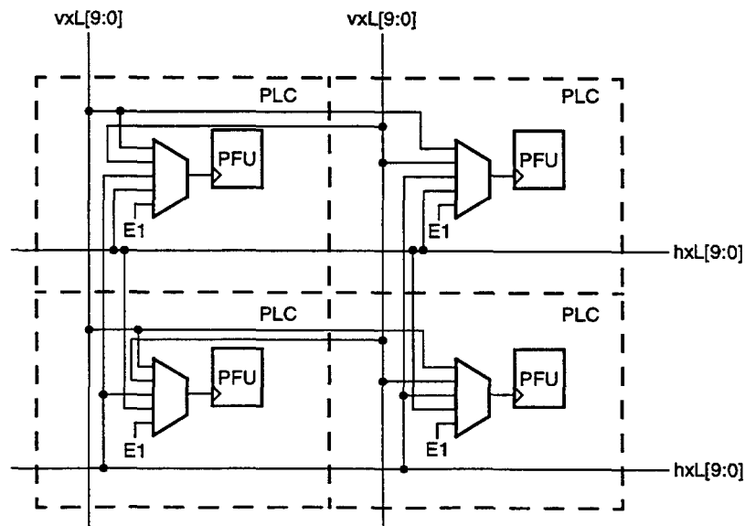
Figure 31. PFU Clock Sources
