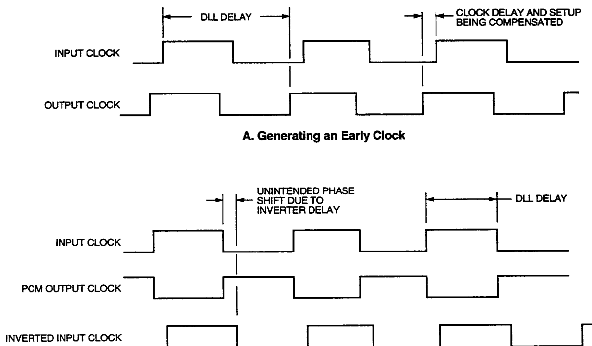
B. Multiphase Clock Generation Using the DLL
