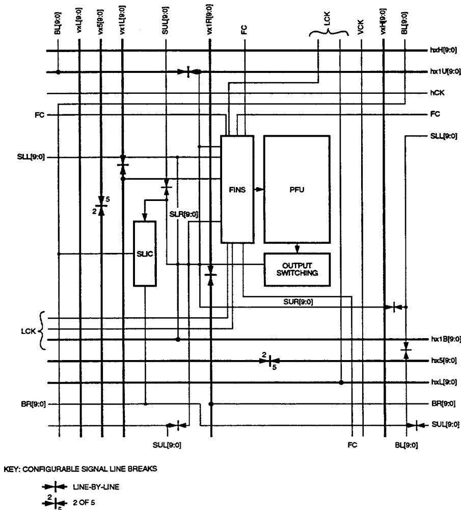
Figure 19. Single PLC View of Inter-PLC Route Segments
