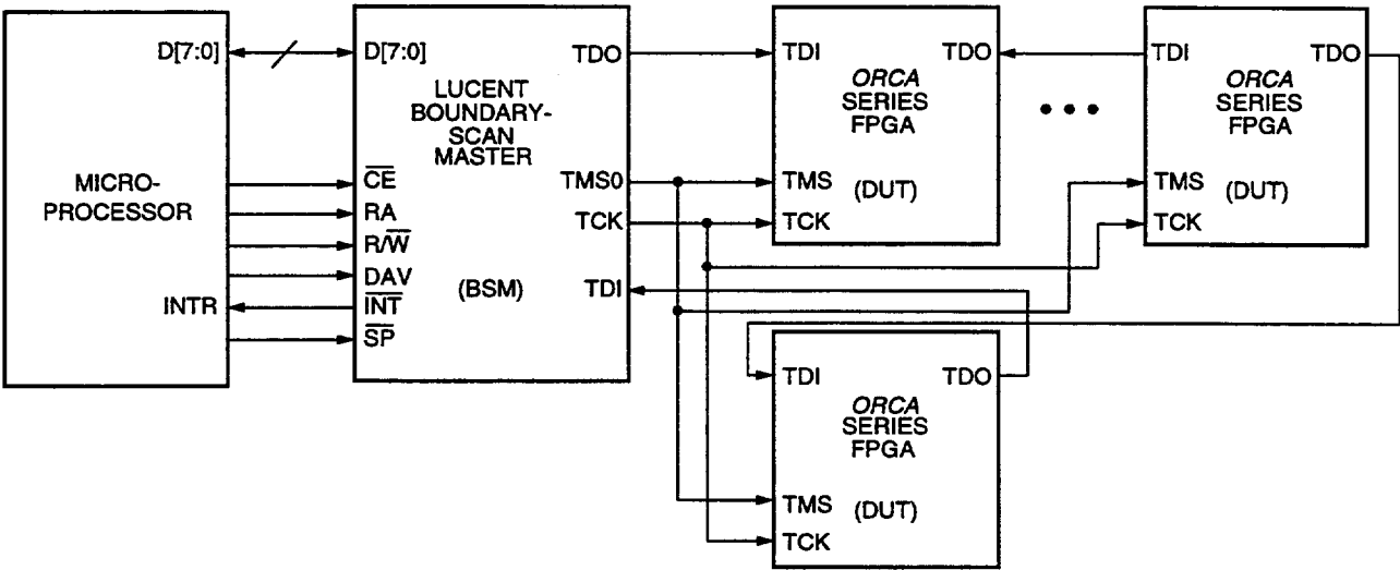
Figure 37. Boundary-Scan Interface
