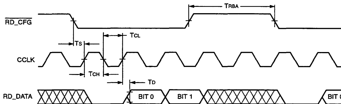
Figure 88. Readback Timing Diagram
