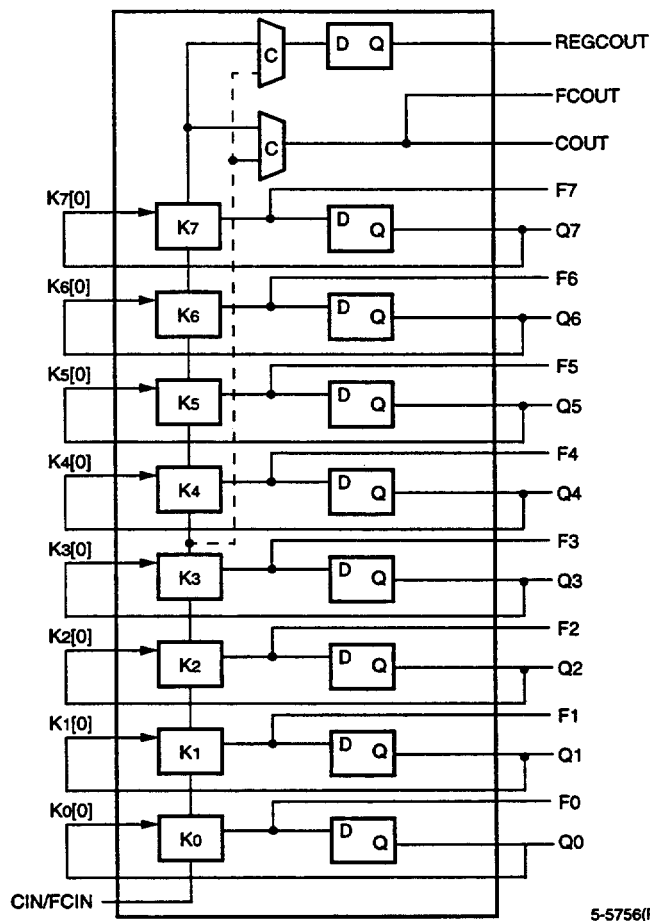
Figure 7. Counter Submode
