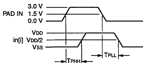
Figure 91. Input Buffer Delays
