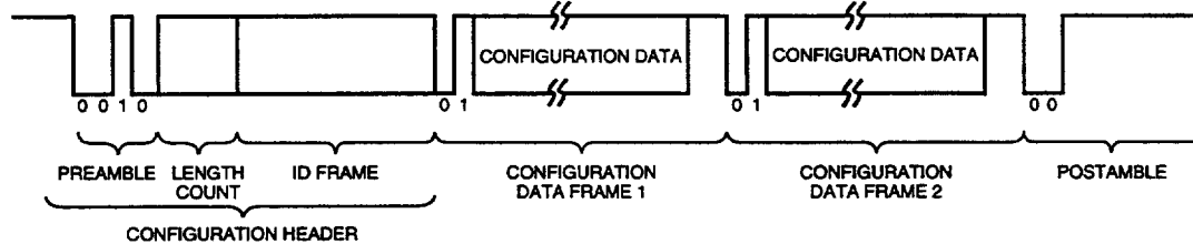
Figure 52. Serial Configuration Data Format—Autoincrement Mode
