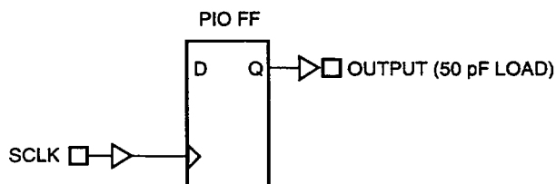
Figure 78. System Clock to Output Delay
