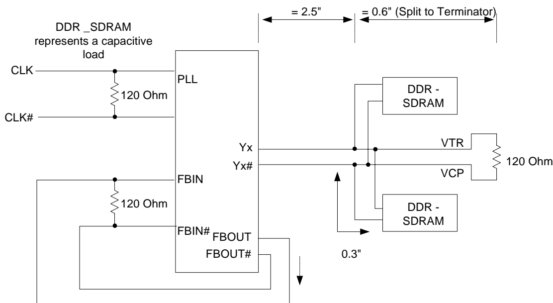
Figure 1. Clock Structure 1 [1]
