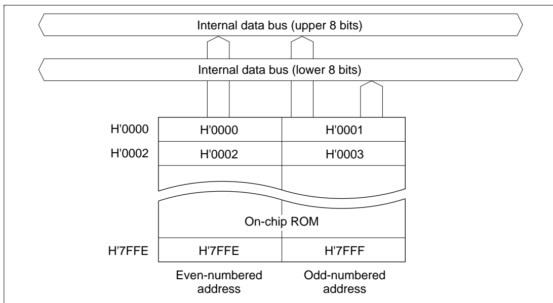
Figure 6.1 ROM Block Diagram (H8/3824R and H8/3824S)
