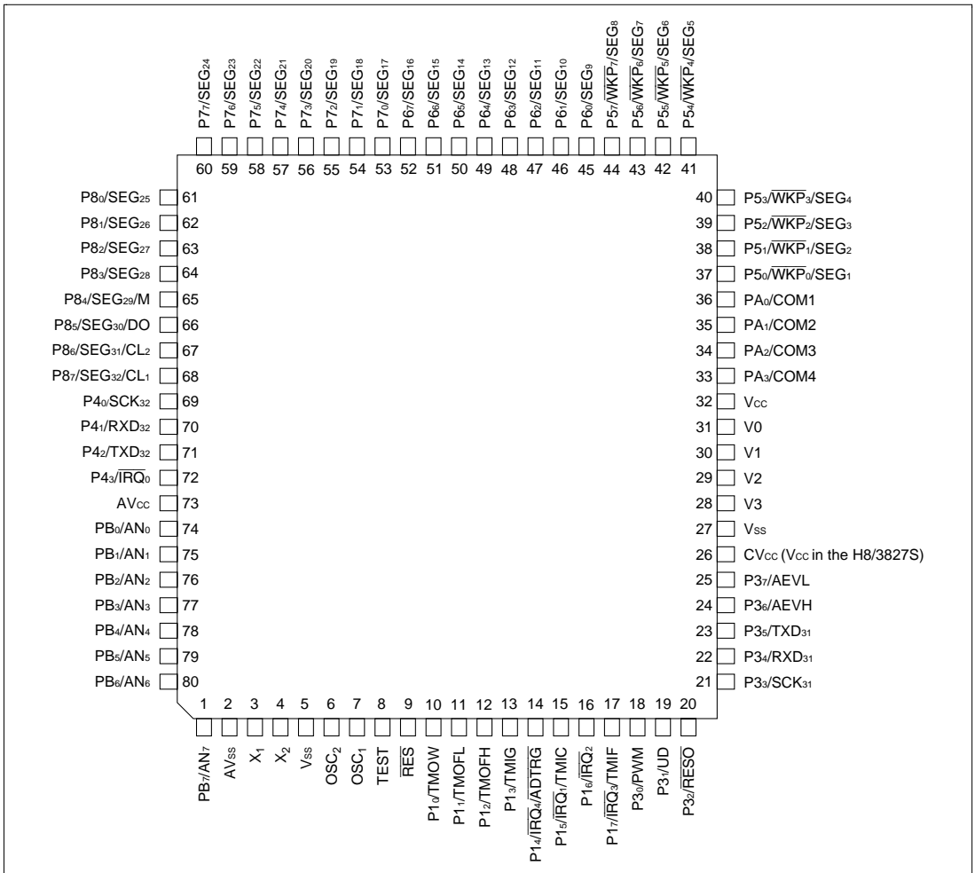
Figure 1.2 Pin Arrangement (FP-80A, TFP-80C: Top View)
