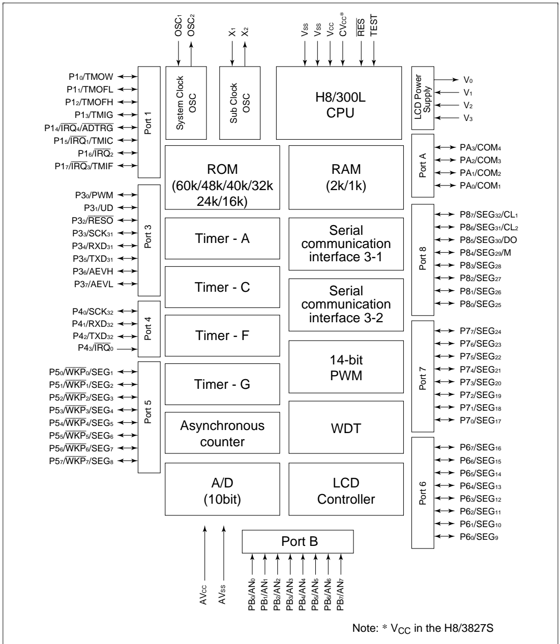
Figure 1.1 Block Diagram
