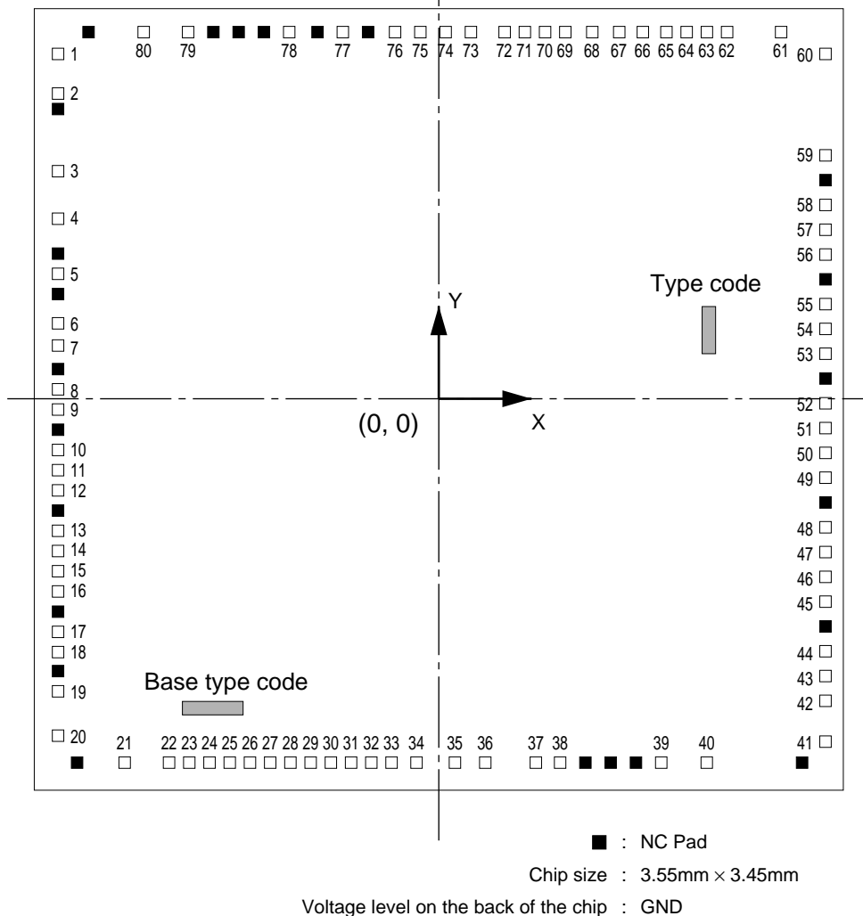
Figure 1.5 Bonding Pad Location Diagram of HCD6433827S, HCD6433826S, HCD6433825S, and HCD6433824S (Top View)
