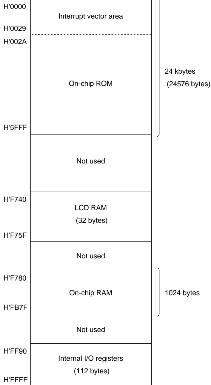
Figure 2.16 (2) H8/3823R Memory Map
