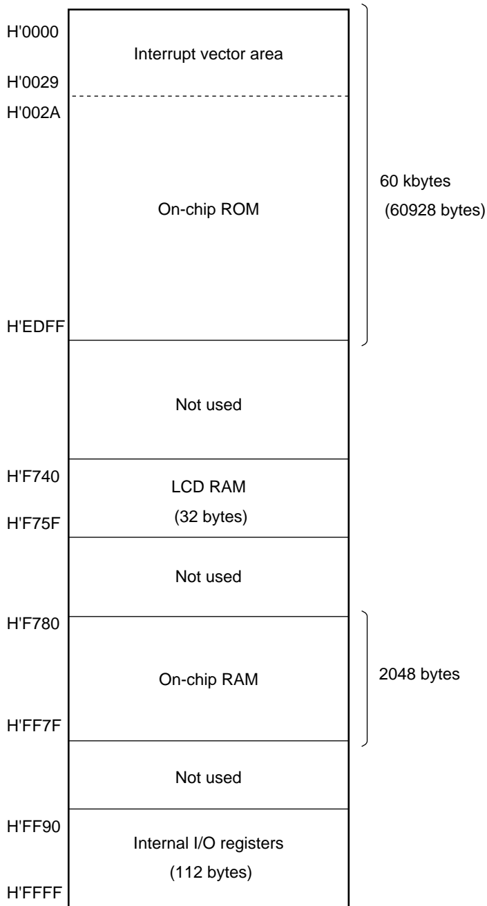
Figure 2.16 (6) H8/3827R and H8/3827S Memory Map
