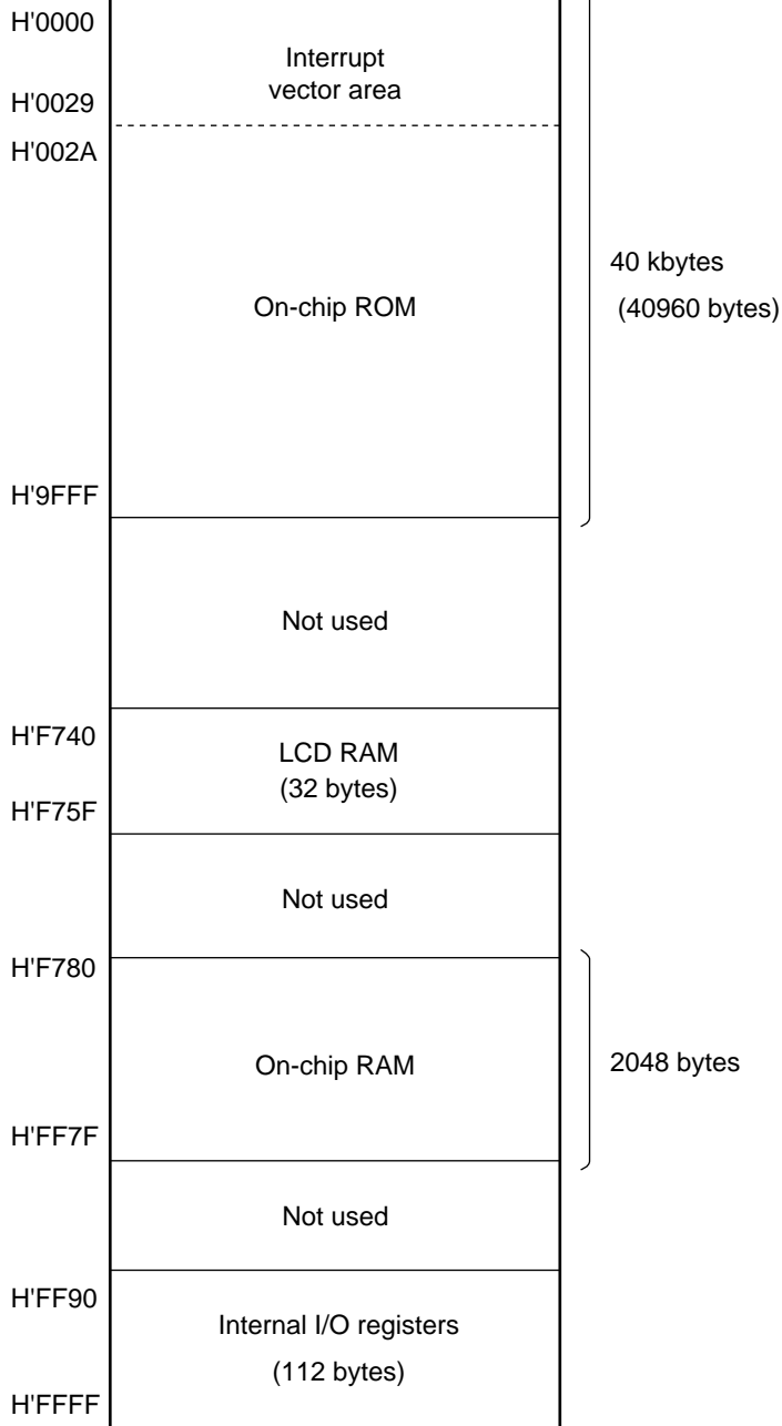
Figure 2.16 (4) H8/3825R and H8/3825S Memory Map
