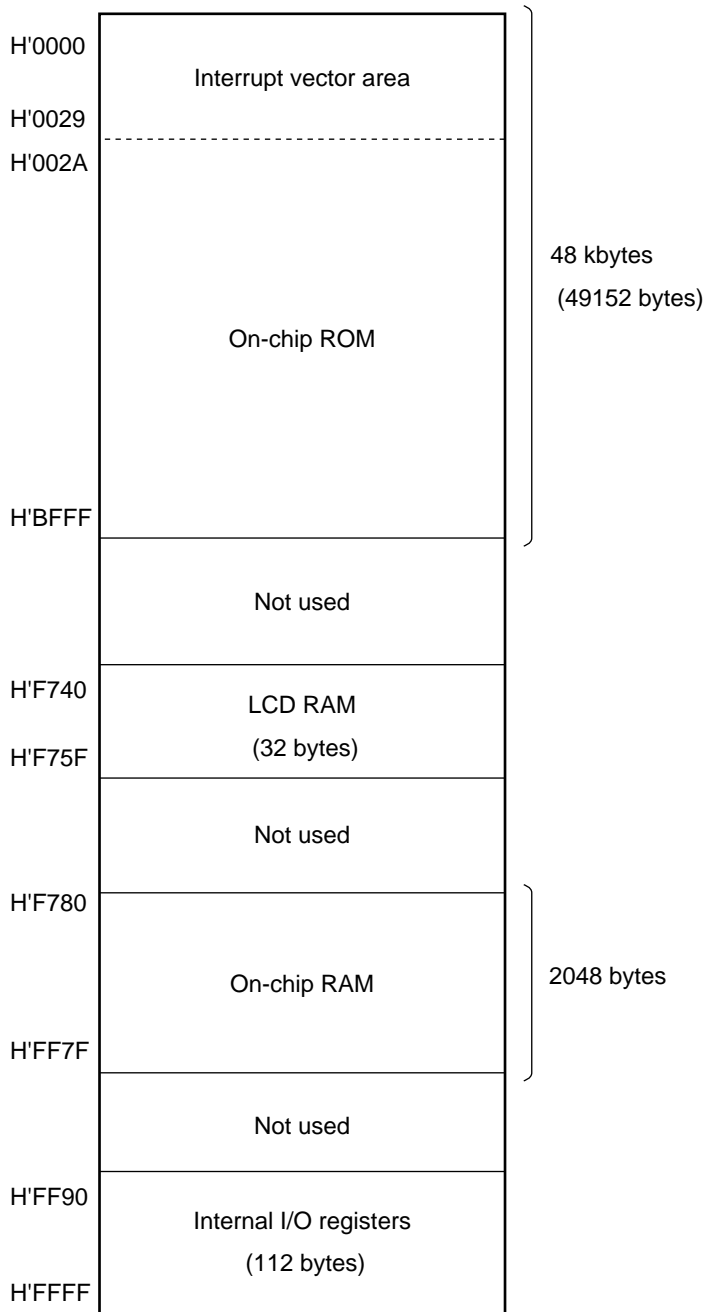
Figure 2.16 (5) H8/3846R and H8/3846S Memory Map
