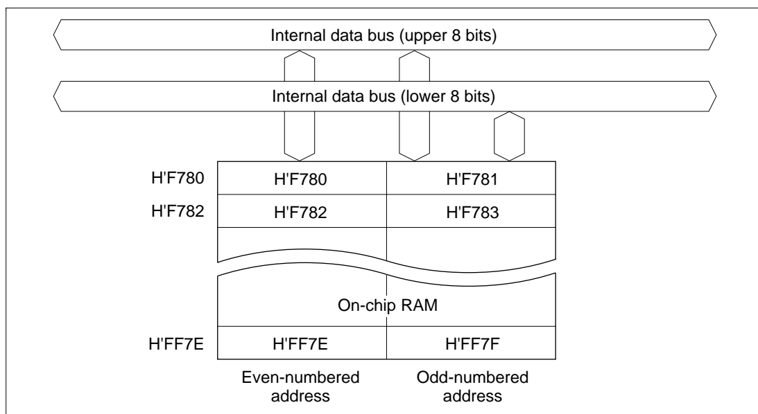
Figure 7.1 RAM Block Diagram (H8/3844R and H8/3844S)
