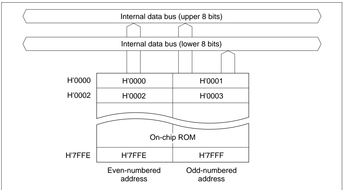
Figure 6.1 ROM Block Diagram (H8/3844R and H8/3844S)
