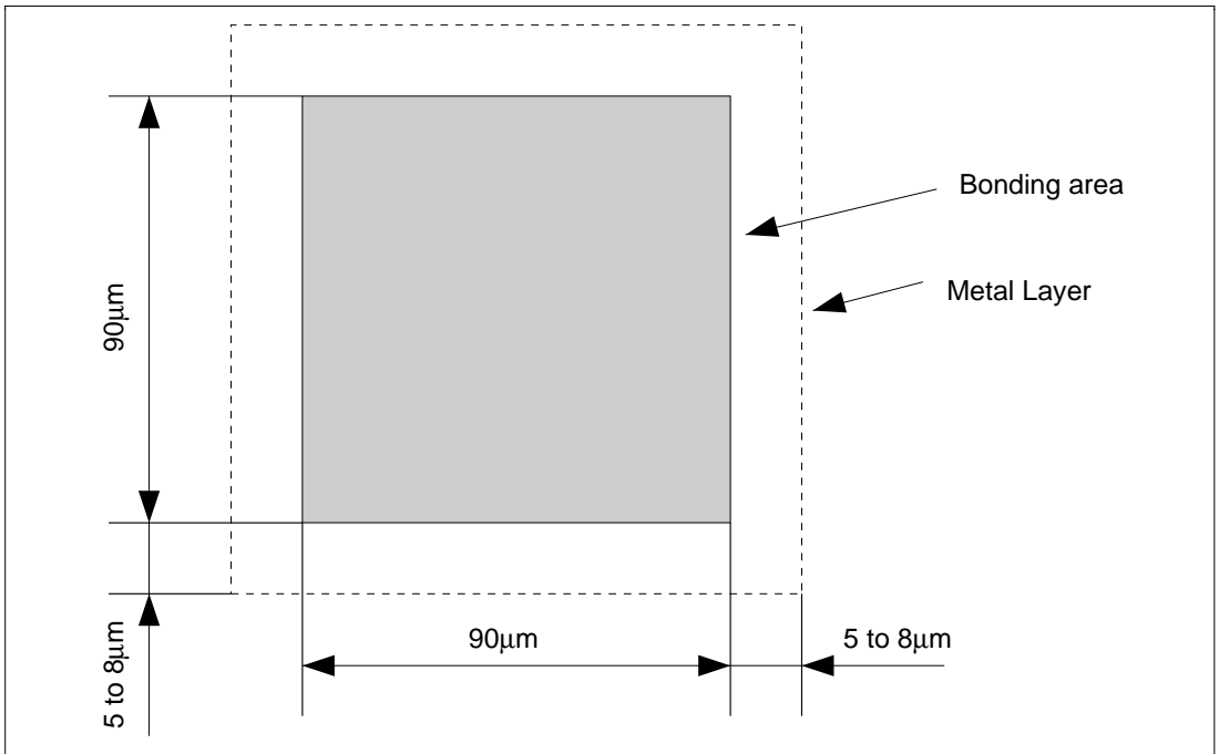
Figure H.1 Bonding Pad Form
