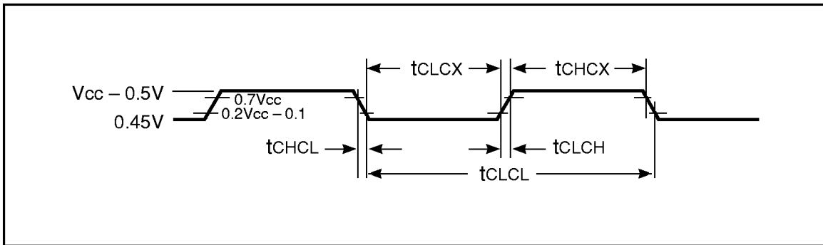
Figure 36. ROM Verification Waveforms
