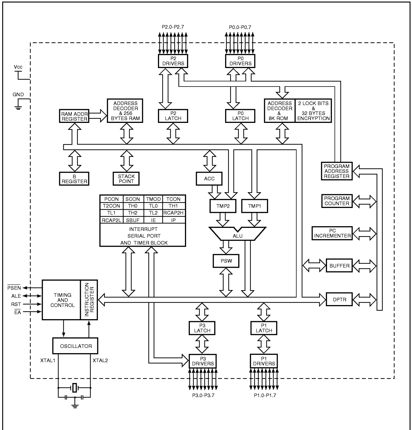
Figure 3. IS80C52/32 Block Diagram
