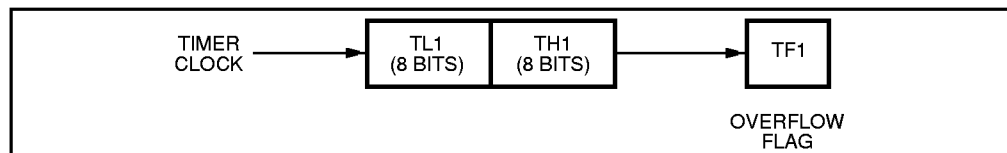
Figure 8. Timer/Counter 1 Mode 1: 16-Bit Counter
