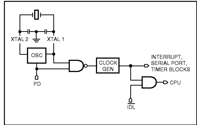
Figure 22. Idle and Power-Down Hardware
