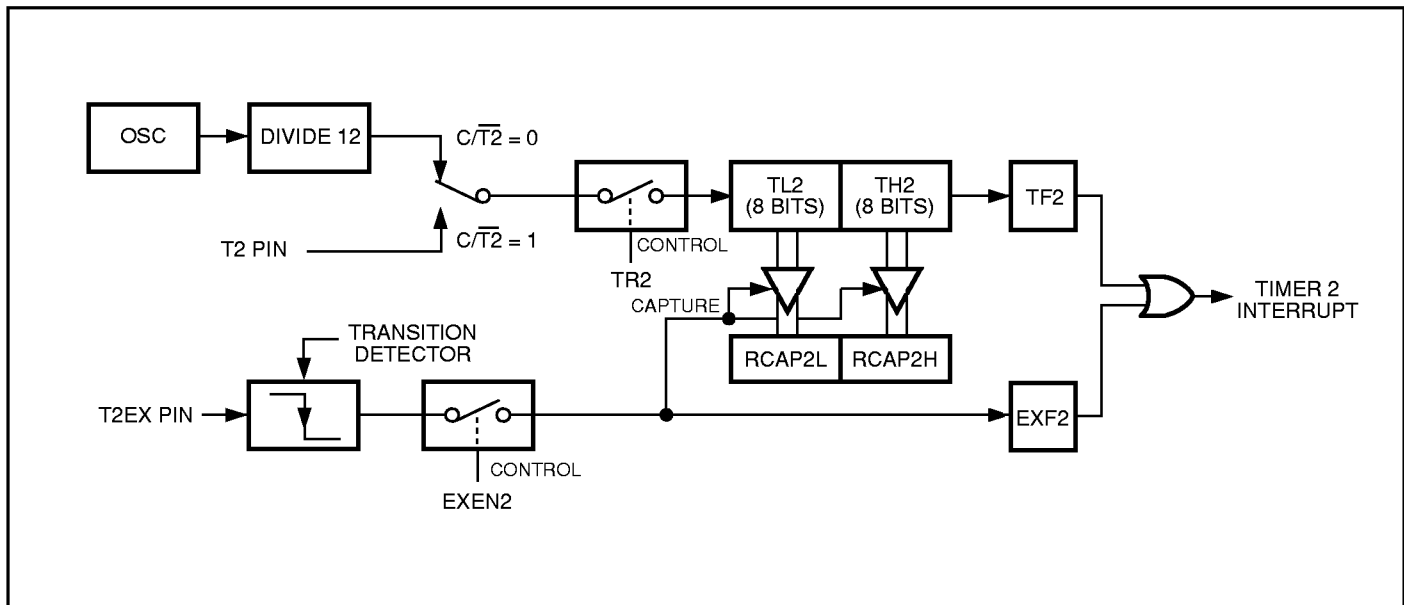
Figure 11. Timer 2 In Capture Mode
