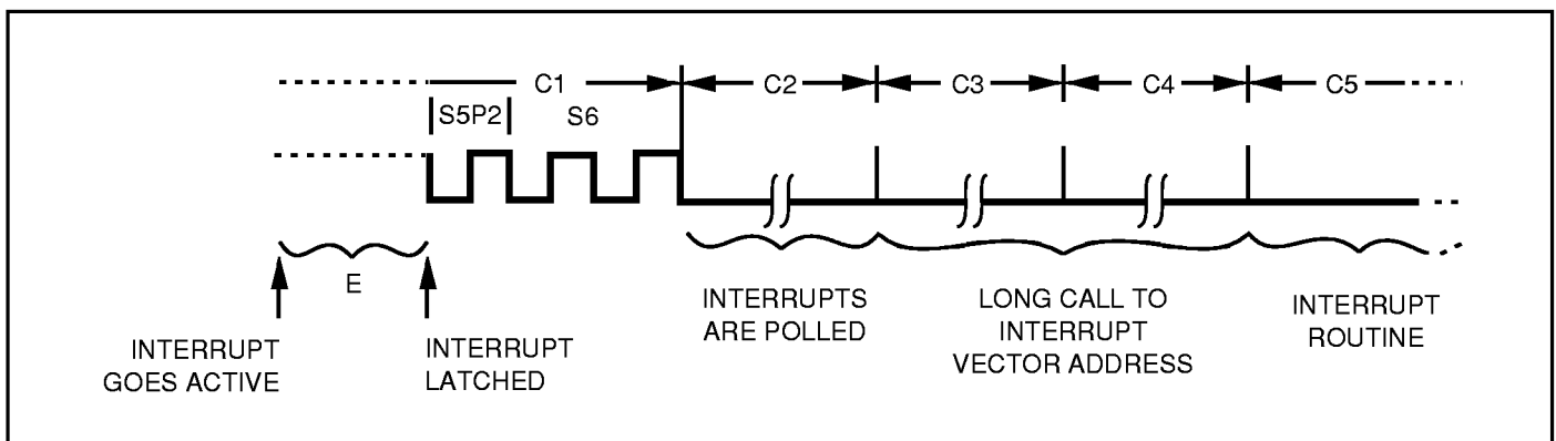
Figure 19. Interrupt Response Timing Diagram
