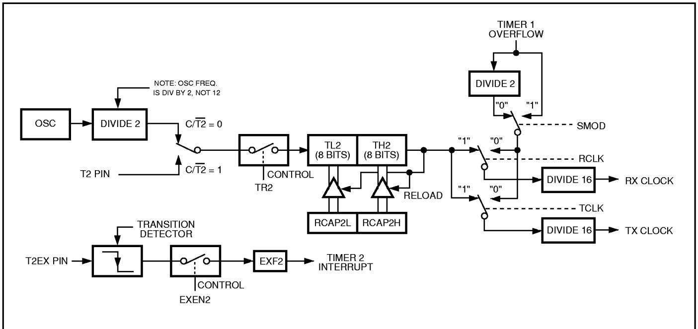
Figure 13. Timer 2 in Baud Rate Generator Mode
