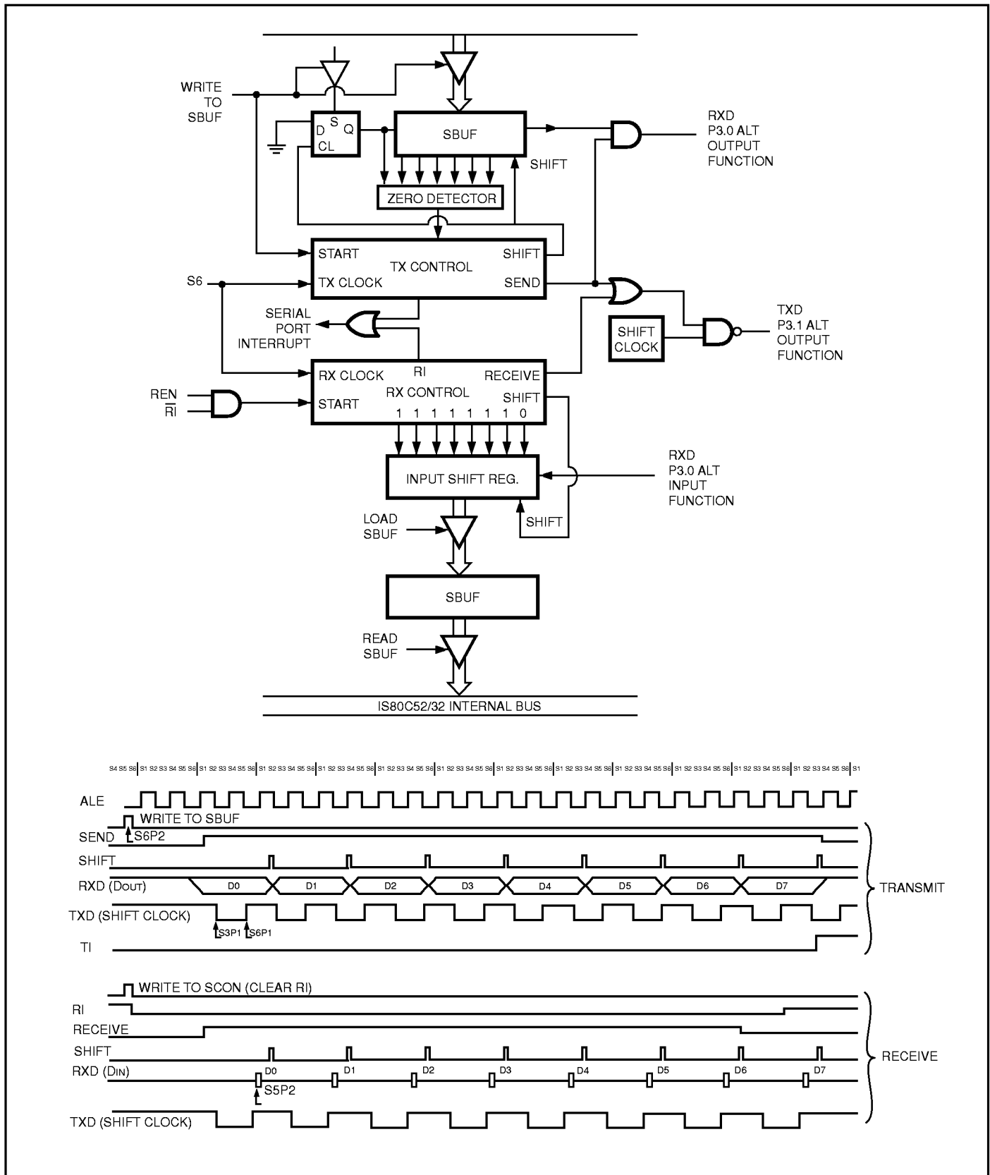
Figure 14. Serial Port Mode 0
