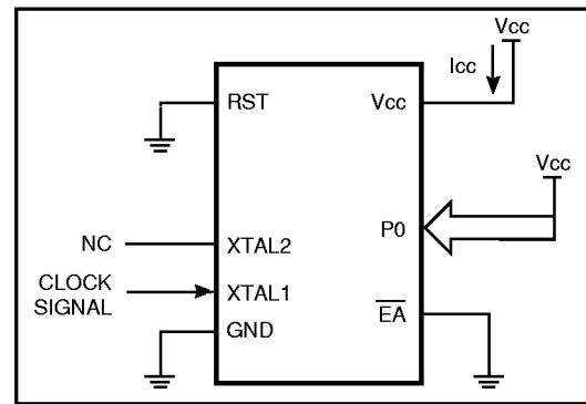
Figure 28. Idle Mode
