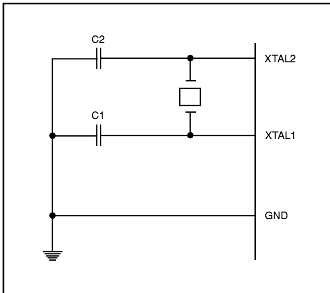
Figure 23. Oscillator Connections
