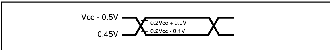
Figure 37. AC Test Point
