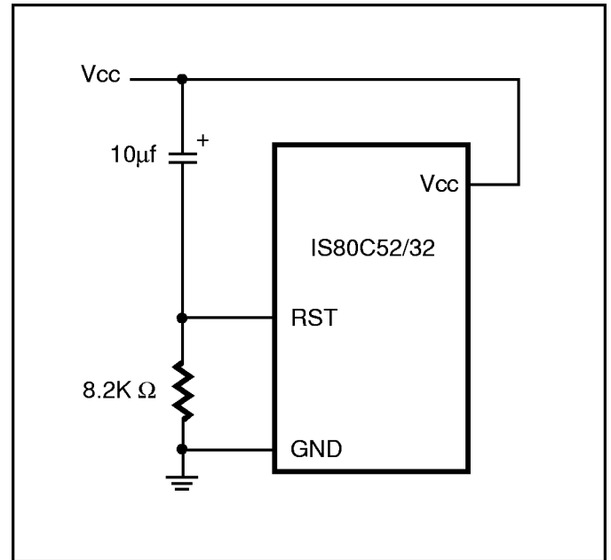
Figure 20. Power-On Reset Circuit
