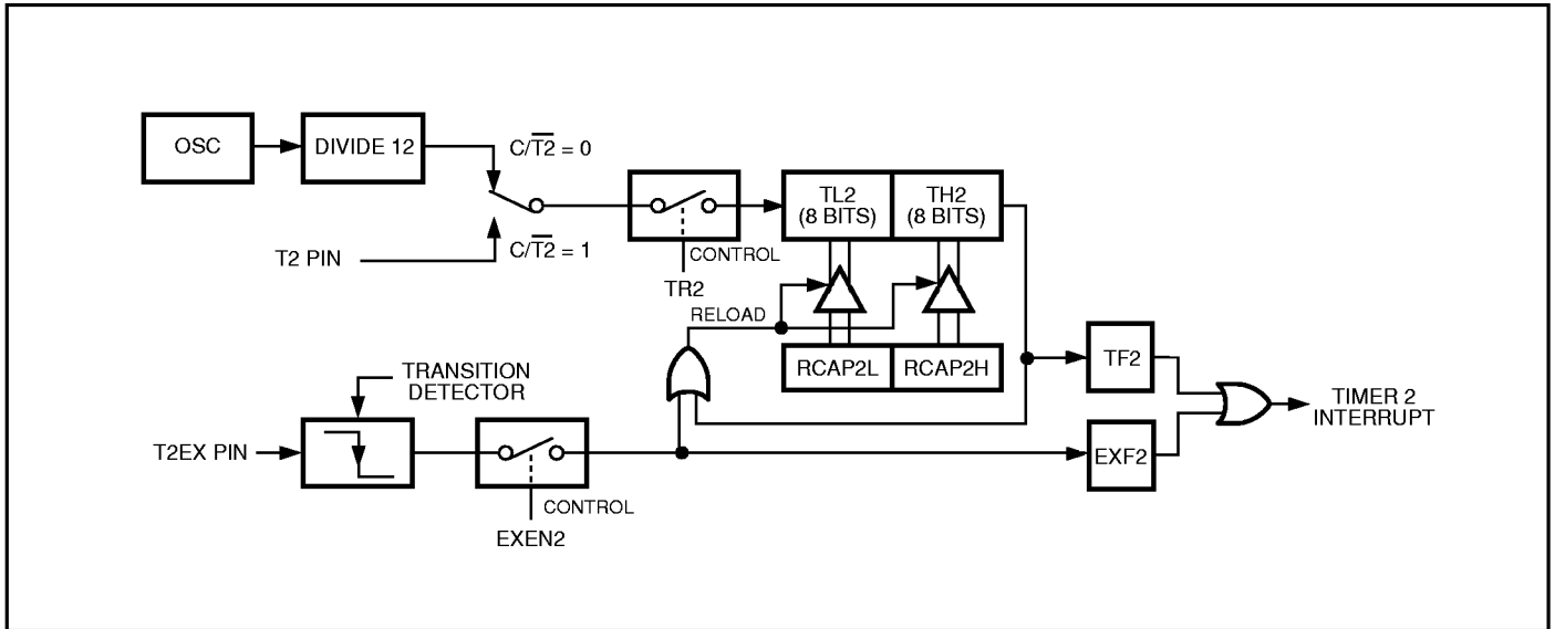
Figure 12. Timer 2 in Auto-Reload Mode
