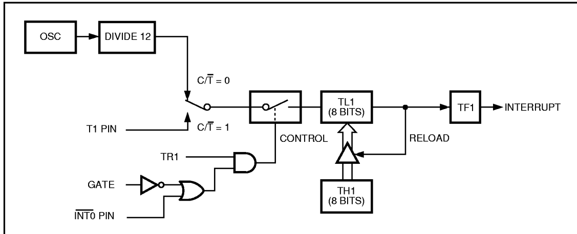
Figure 9. Timer/Counter 1 Mode 2: 8-Bit Auto-Reload
