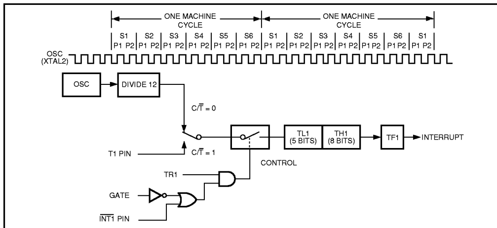
Figure 7. Timer/Counter 1 Mode 0: 13-Bit Counter
