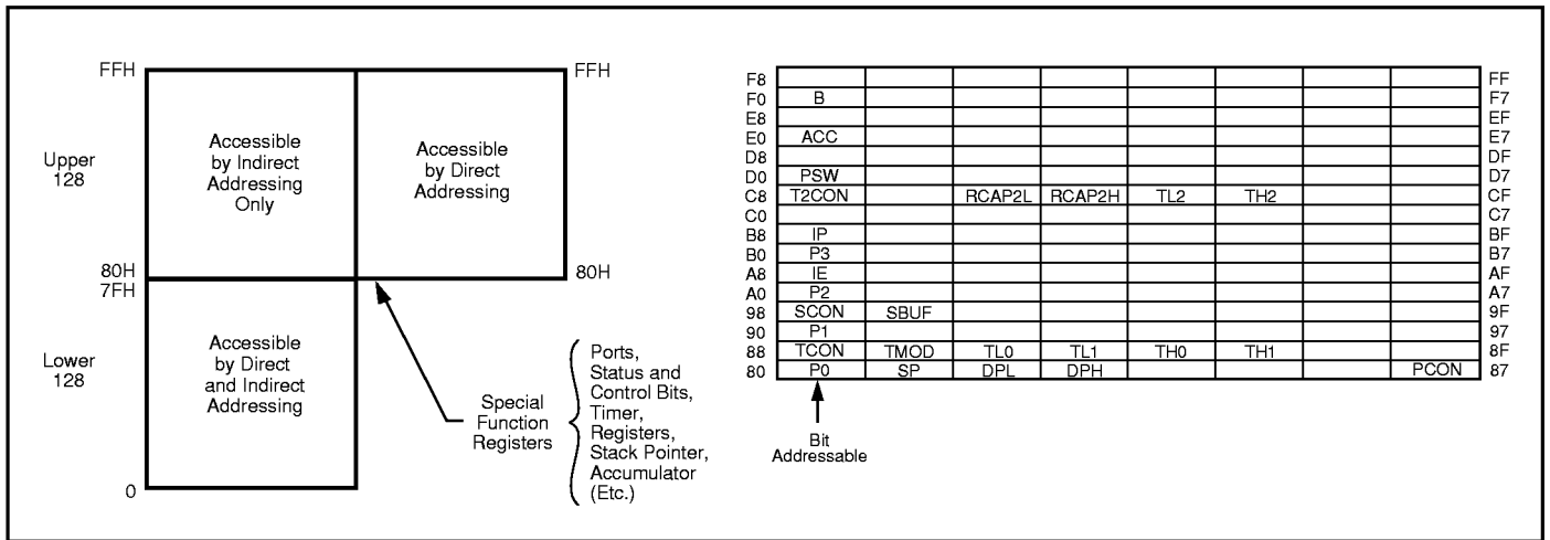
Figure 5. Internal Data Memory and SFR Memory Map
