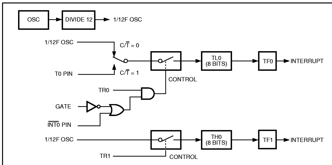
Figure 10. Timer/Counter 0 Mode 3: Two 8-Bit Counters
