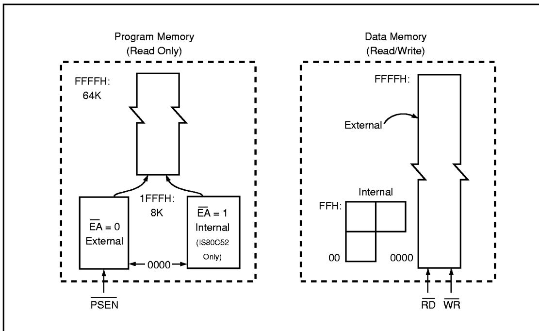
Figure 4. IS80C52/32 Program and Data Memory Structure
