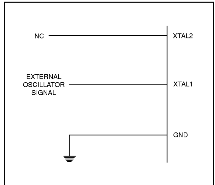
Figure 24. External Clock Drive Configuration
