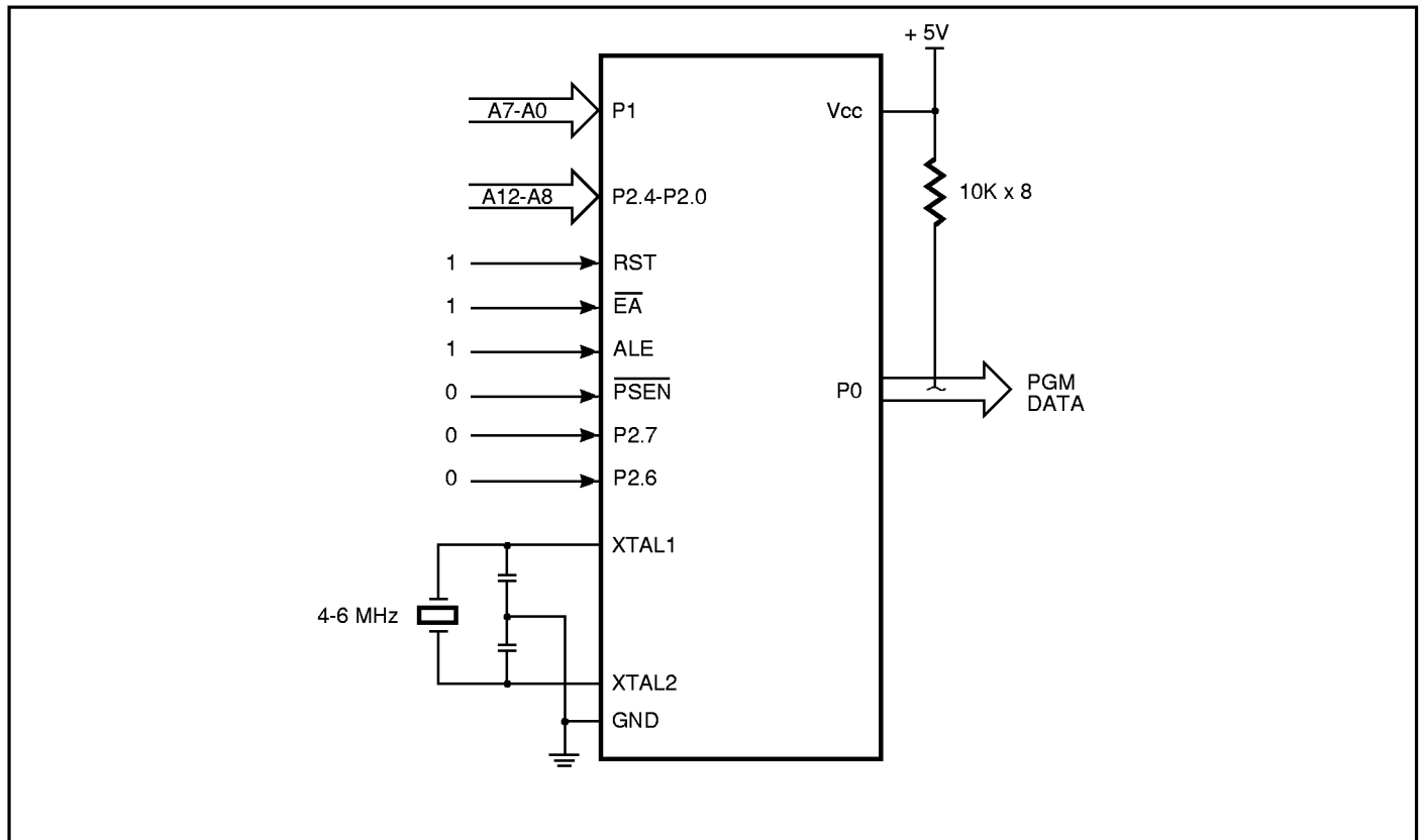
Figure 26. ROM Verification
