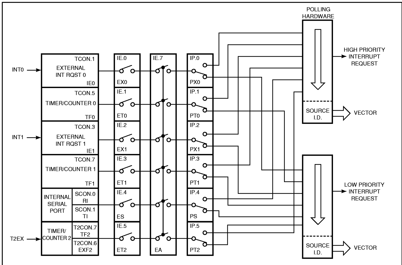
Figure 18. Interrupt System
