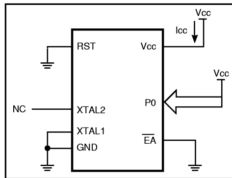
Figure 29. Power-down Mode
