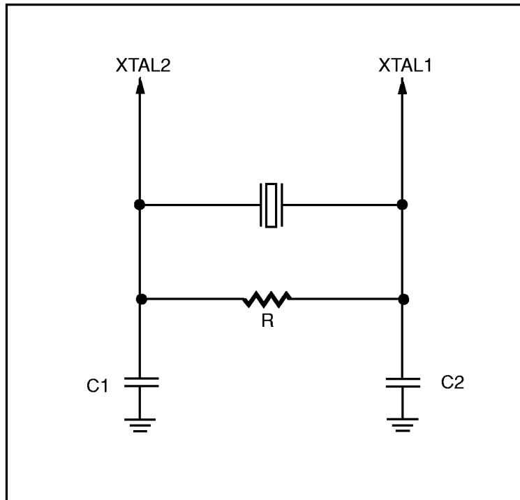
Figure 25. For High Speed (> 24 MHz)
