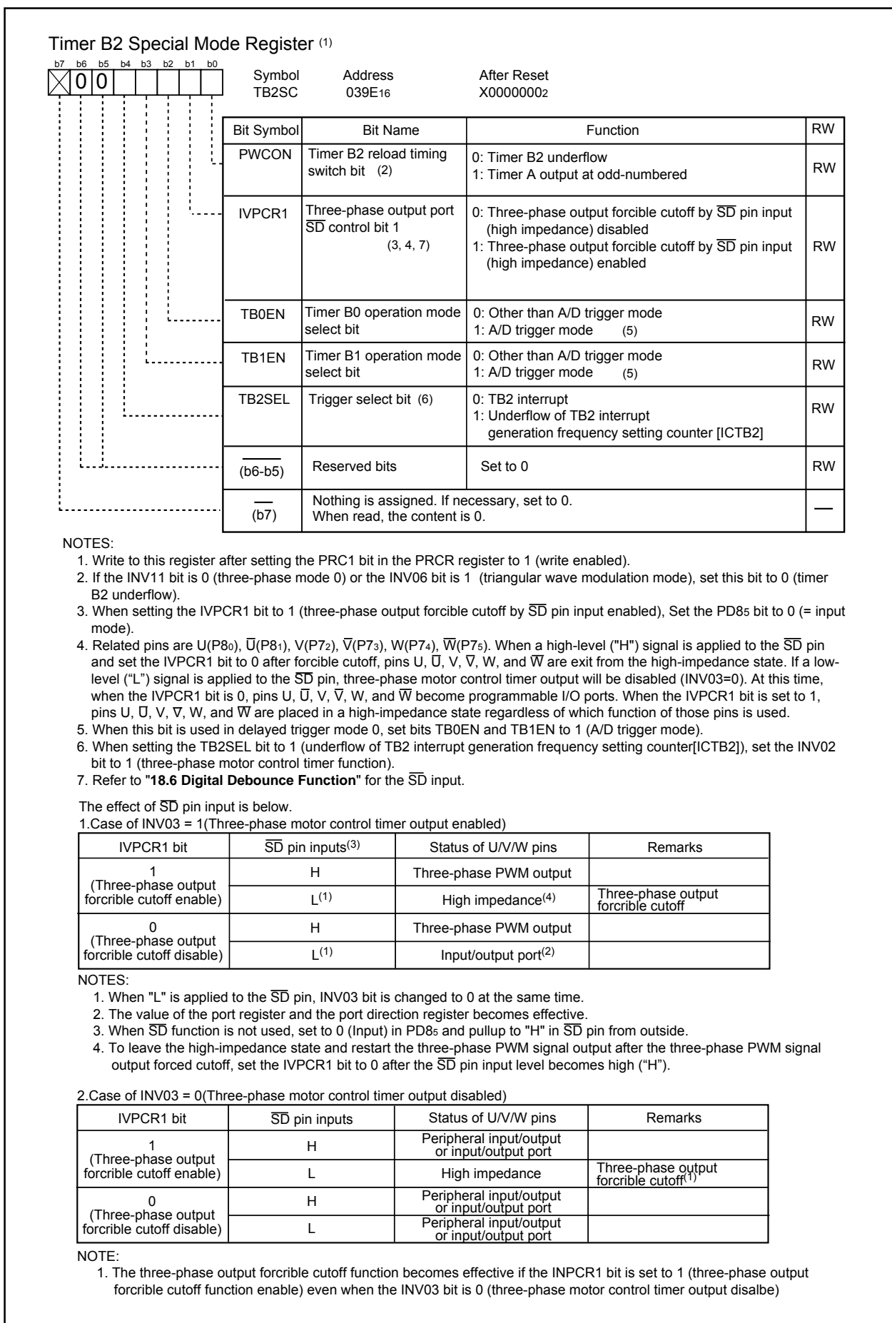
Figure 12.30 TB2SC Register
