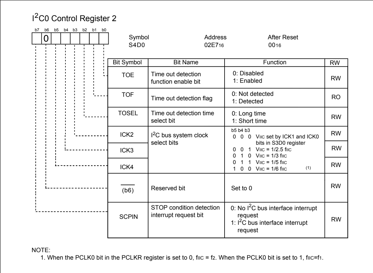
Figure 16.7 S4D0 Register
