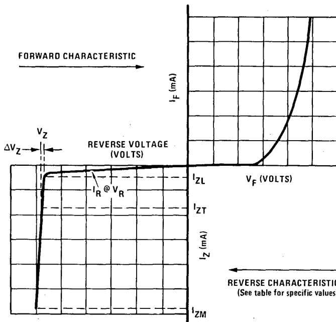
FIGURE 4 Zener Diode Characteristics and Symbol Identification
