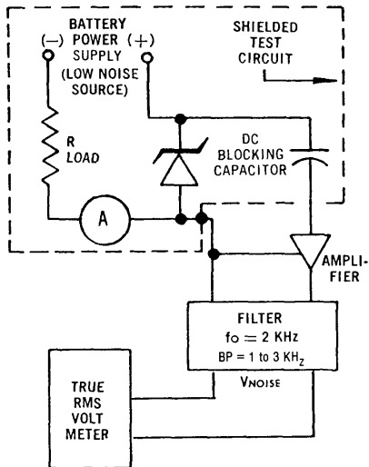
FIGURE 1 Noise Density Measurement Circuit
