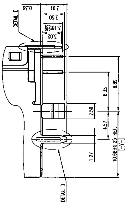
VIEW B
