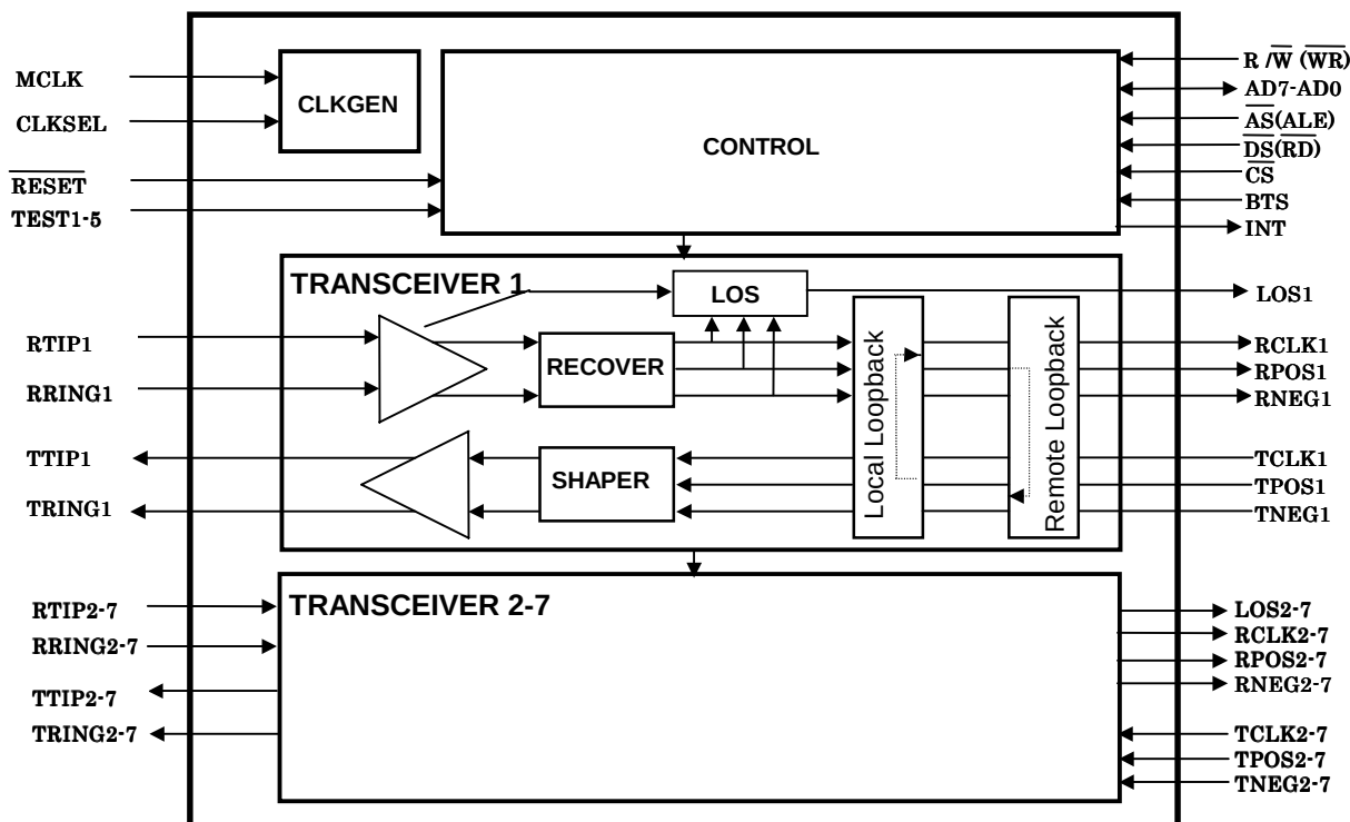
7 Channel T1 Transceiver Block Diagram
