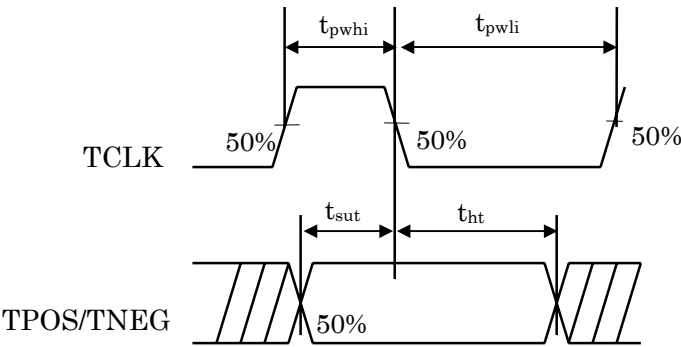
Fig.2 Transmitter Timing
