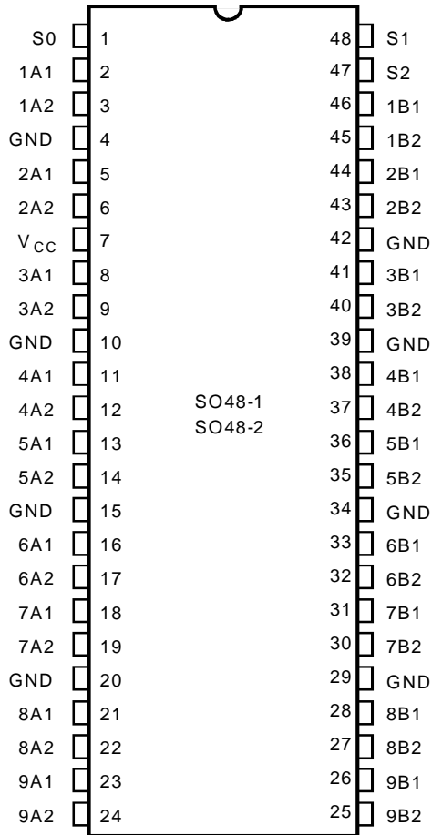
SSOP/ TSSOP TOP VIEW
