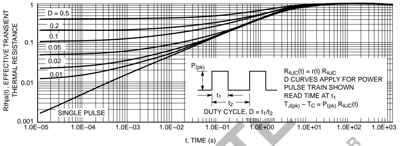
Figure 13. Thermal Response
