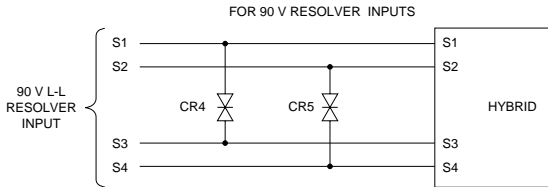
CR4 and CR5 are 1N6136A, bipolar transient voltage suppressors or equivalent.
