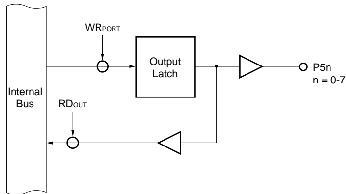
Figure 5-39. Port Specified as Output Port
