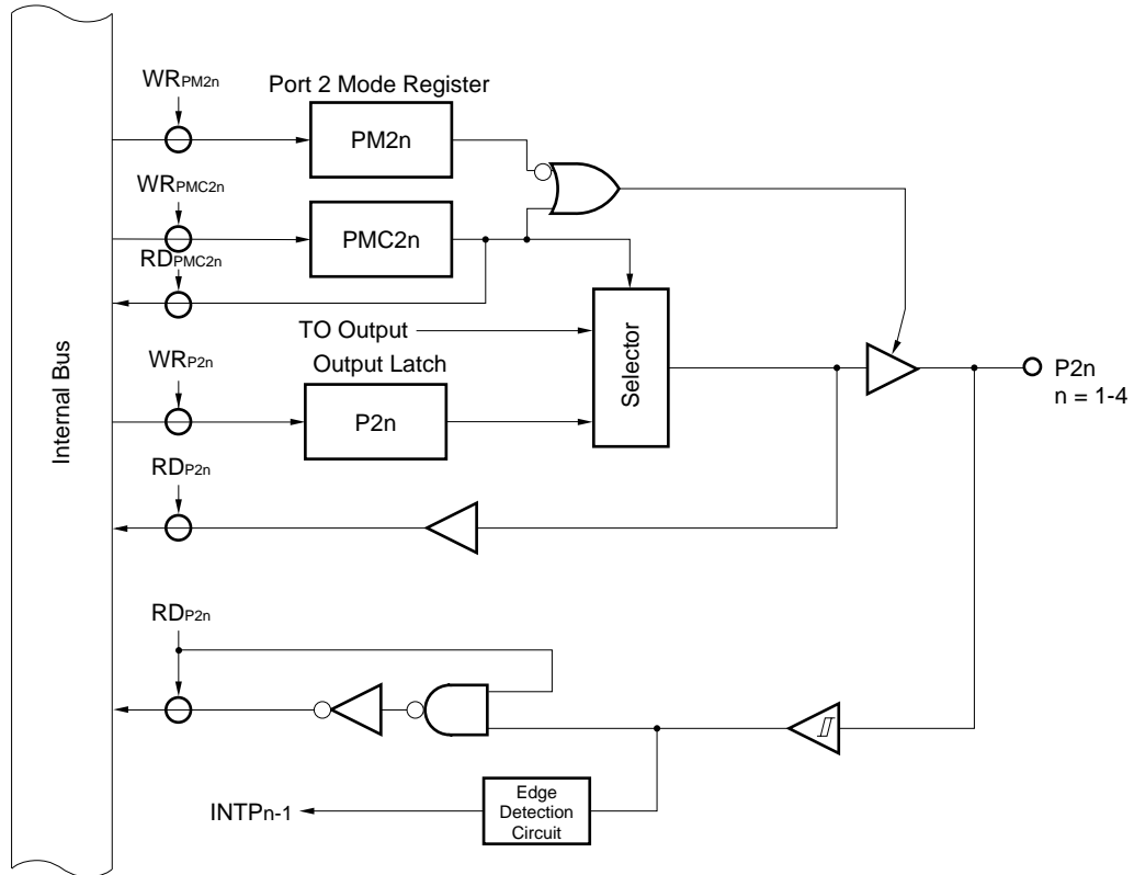
Figure 5-16. Block Diagram of P21 to P24 (Port 2)
