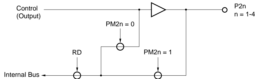
Figure 5-22. Port in Control Mode
