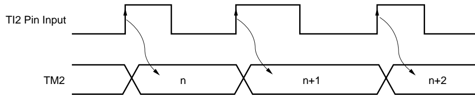
Figure 10-39. External Event Counter Operation
