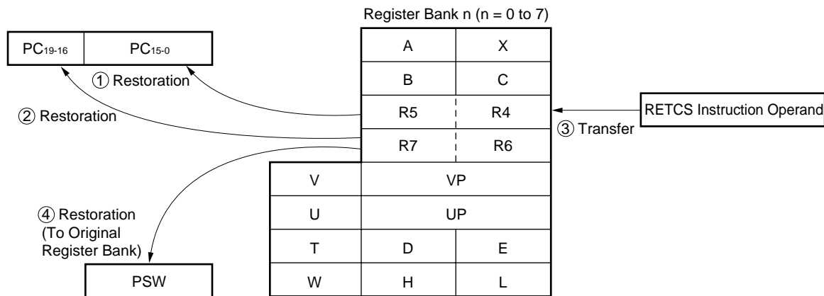
Figure 16-12. Return from Interrupt that Uses Context Switching by Means of RETCS Instruction
