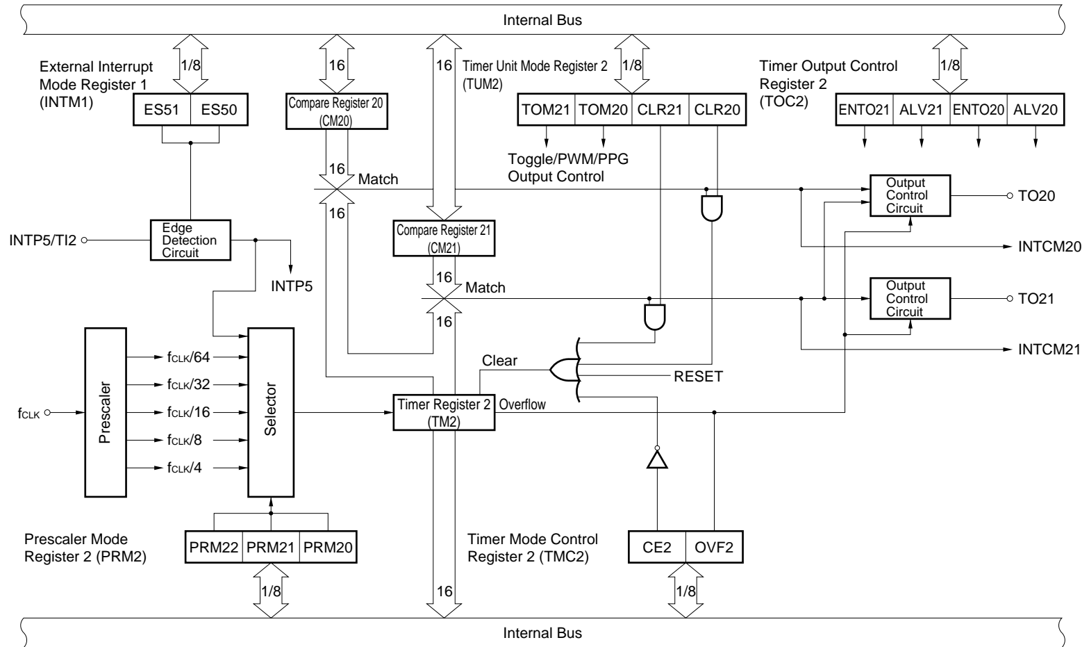
Figure 10-1. Block Diagram of Timer/Counter 2
