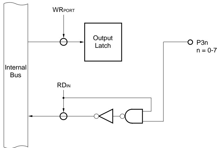
Figure 5-29. Port Specified as Input Port
