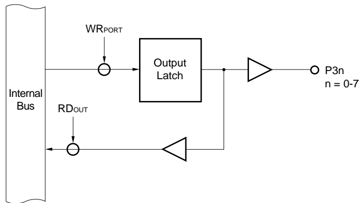
Figure 5-28. Port Specified as Output Port
