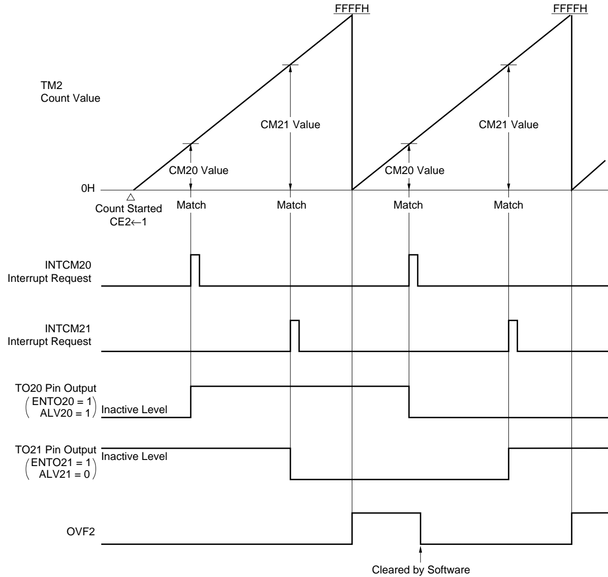
Figure 10-10. Compare Operation (timer/counter 2)
