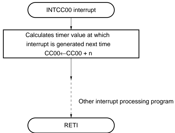
Figure 8-16. Interrupt Request Processing of Interval Timer Operation
