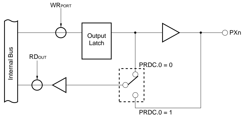
Figure 5-60. Concept of Control (in output port mode)
