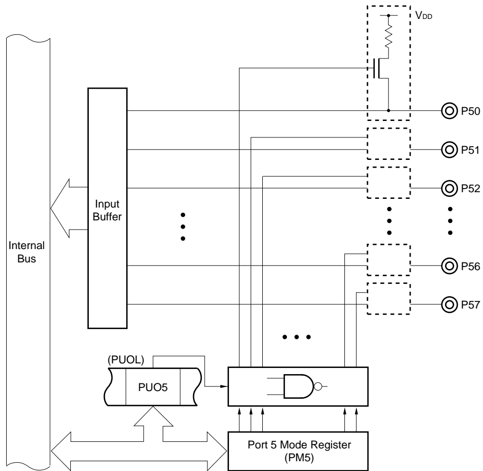
Figure 5-42. Pull-Up Resistor Specification (Port 5)
