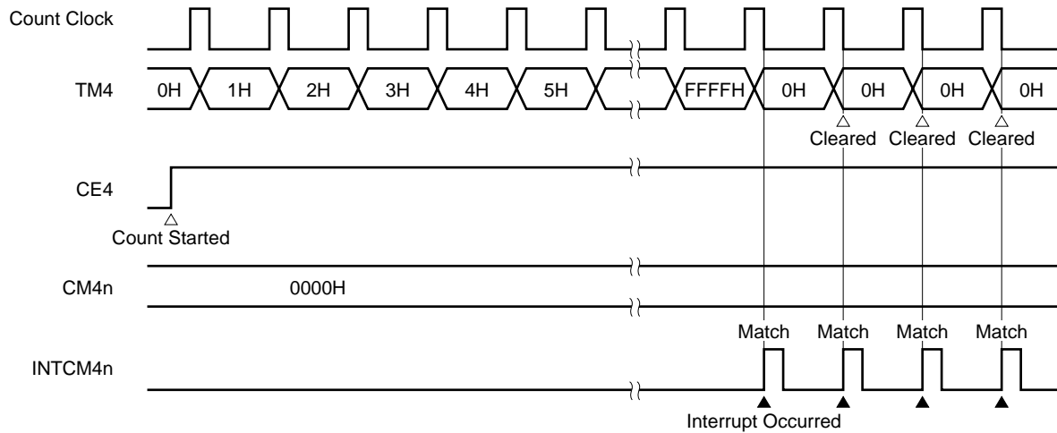
Figure 11-17. Operation When Compare Register (CM40, CM41) Is Set to 0000H
