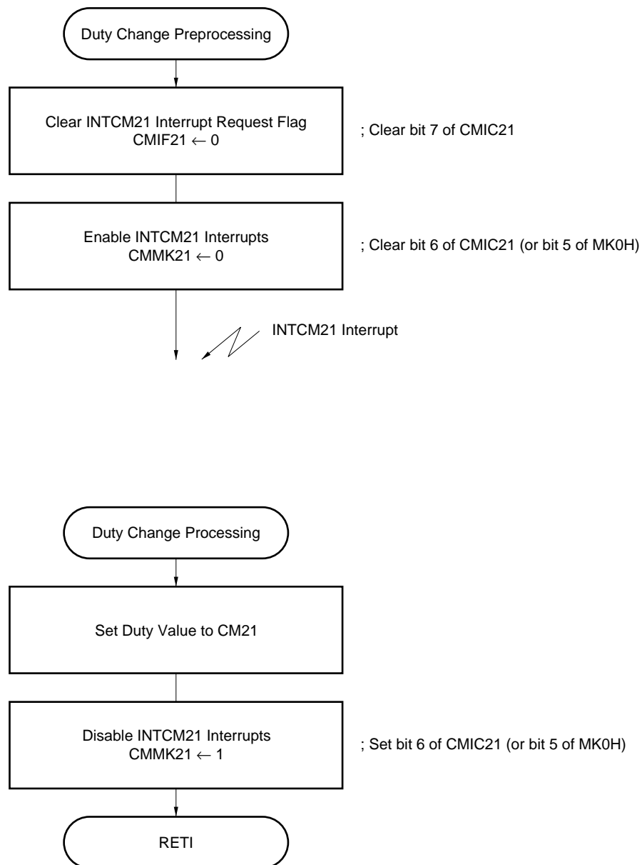
Figure 10-34. Changing PWM Output Duty
