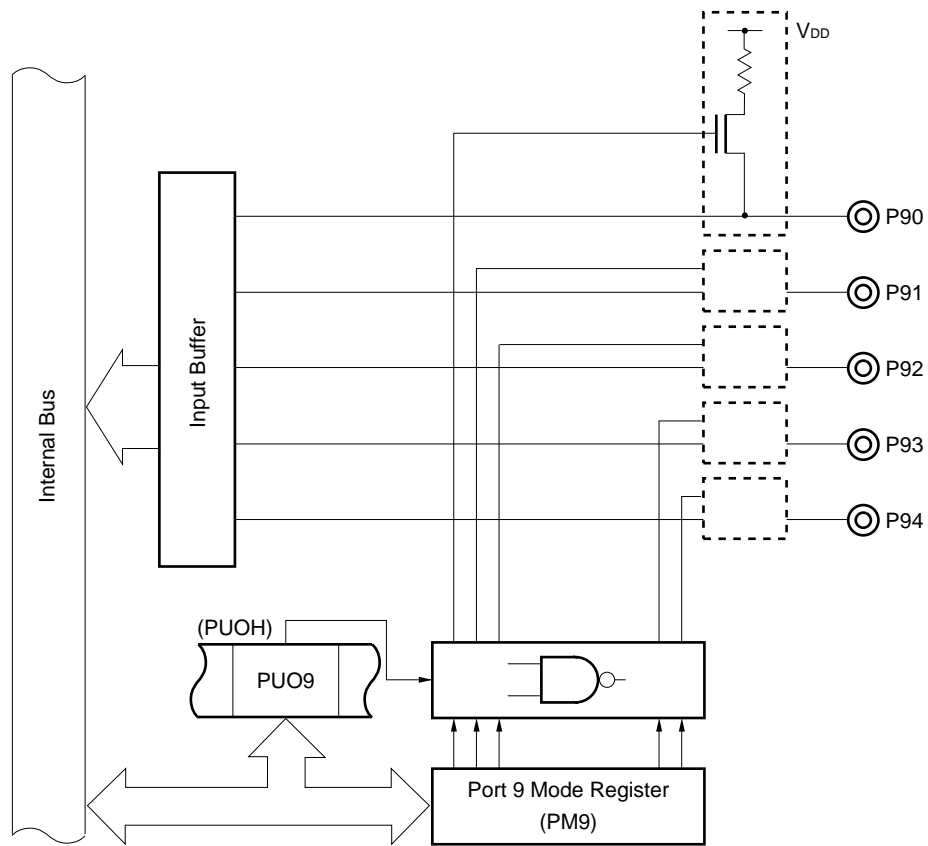
Figure 5-58. Specifying Pull-up Resistor (port 9)
