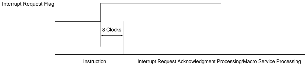
Figure 16-21. Interrupt Request Generation and Acknowledgment (Unit: Clocks)
