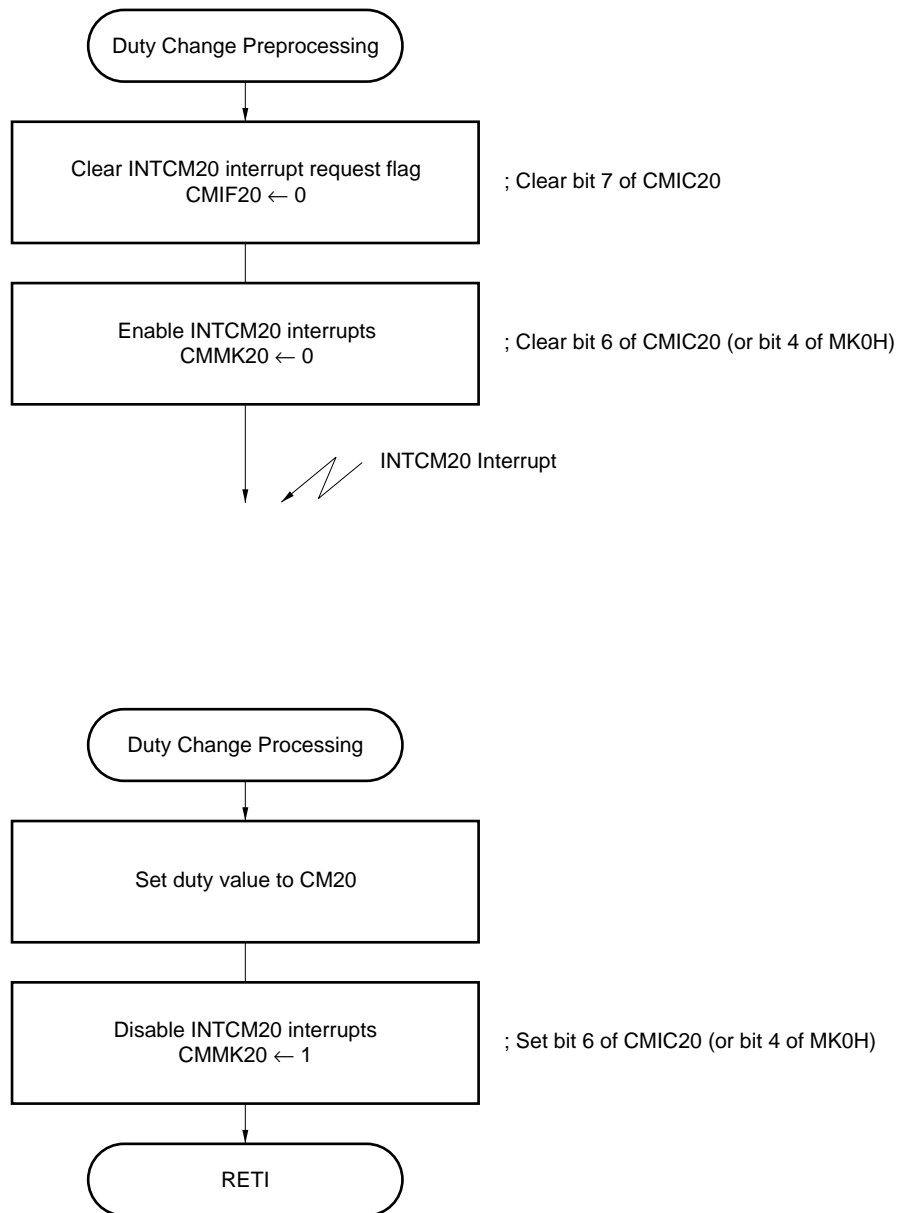
Figure 10-38. Changing PPG Output Duty
