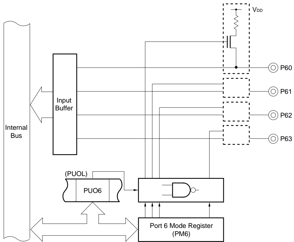
Figure 5-48. Pull-Up Resistor Specification (Port 6)
