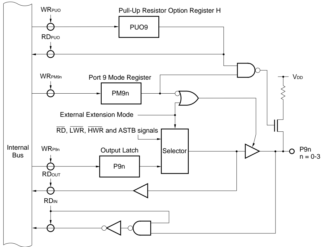
Figure 5-51. Block Diagram of P90 to P93 (Port 9)
