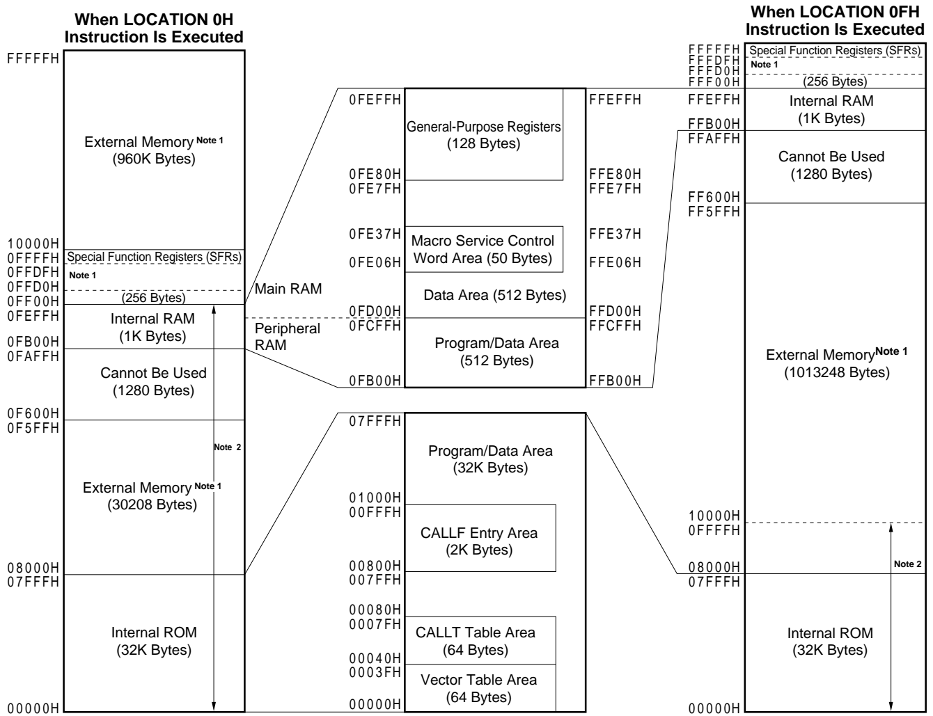
Figure 3-1. \mu PD784044 Memory Map
