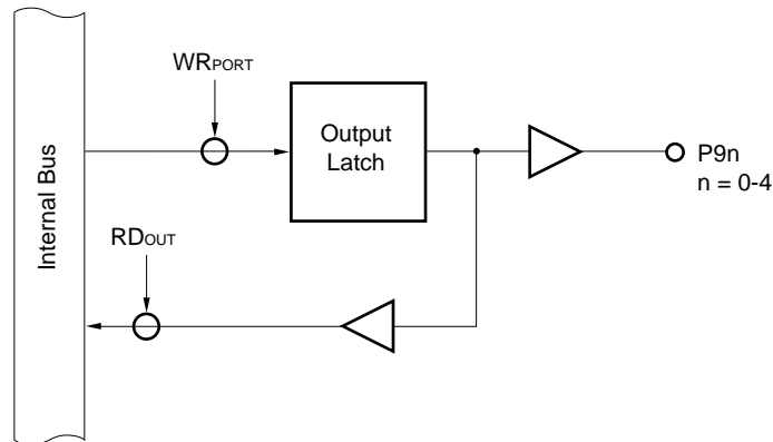
Figure 5-55. Port in Output Port Mode
