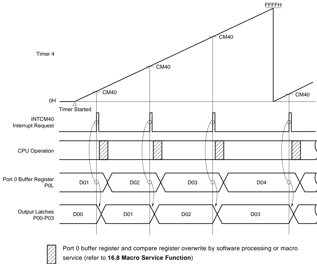
Figure 6-3. Operation Timing of Real-Time Output Port
