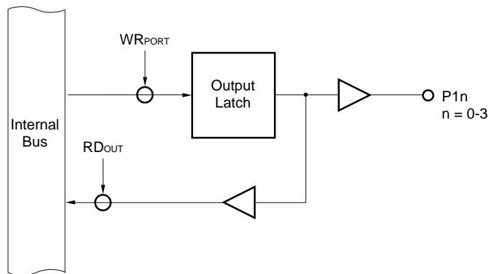
Figure 5-12. Port Specified as Output Port
