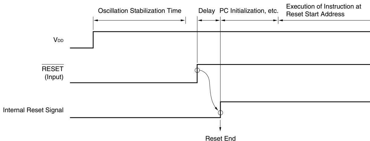
Figure 19-2. Power-On Reset Operation
