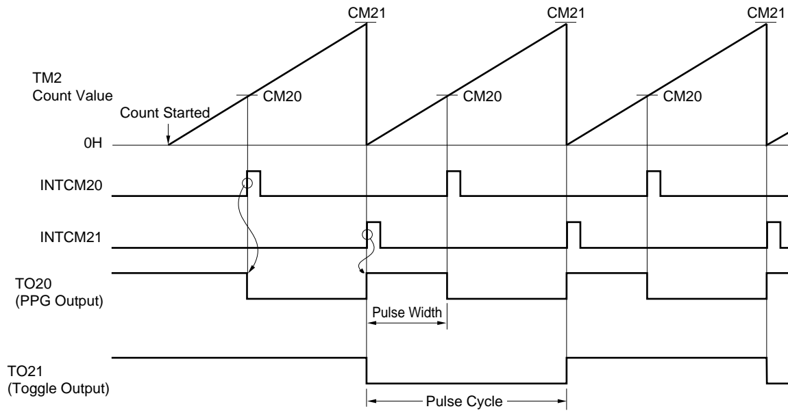
Figure 10-19. Example of PPG Output Using TM2
