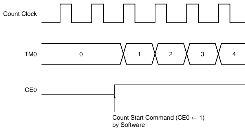
Figure 8-21. Operation When Counting Is Started
