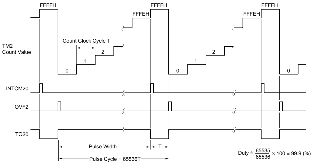
Figure 10-15. Example of PWM Output When CM20 = FFFFH
