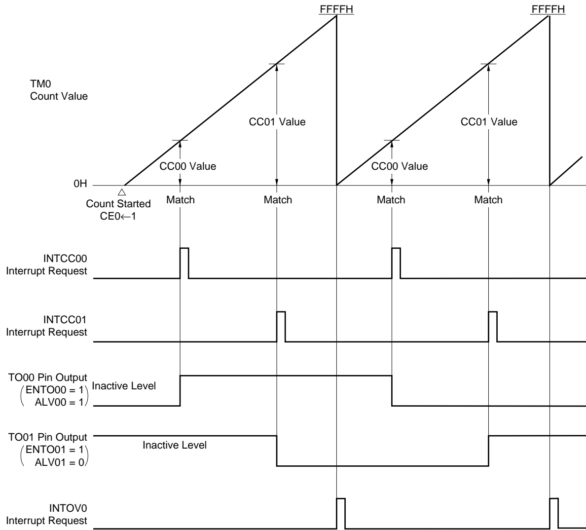
Figure 8-8. Compare Operation (timer 0)
