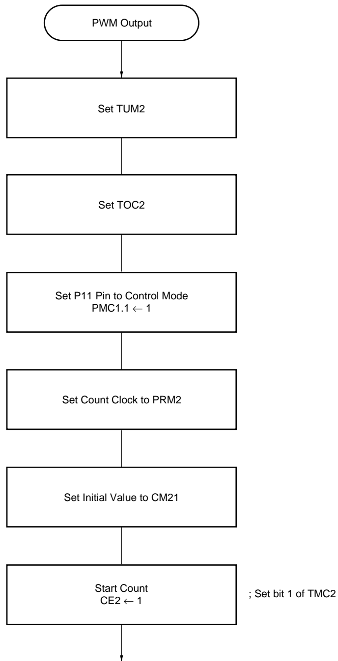
Figure 10-33. Setting Procedure of PWM Output
