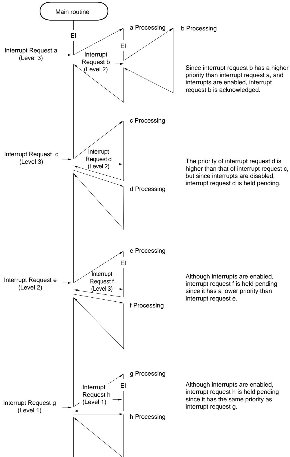
Figure 16-13. Examples of Processing When Another Interrupt Request Is Generated During Interrupt Processing (1/3)
