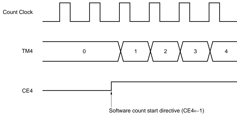
Figure 11-16. Operation When Count Starts
