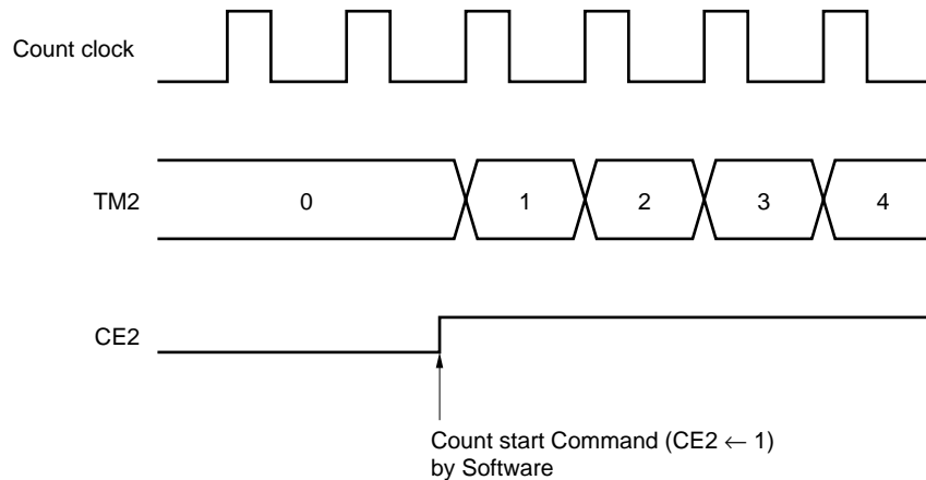
Figure 10-42. Operation When Counting Is Started
