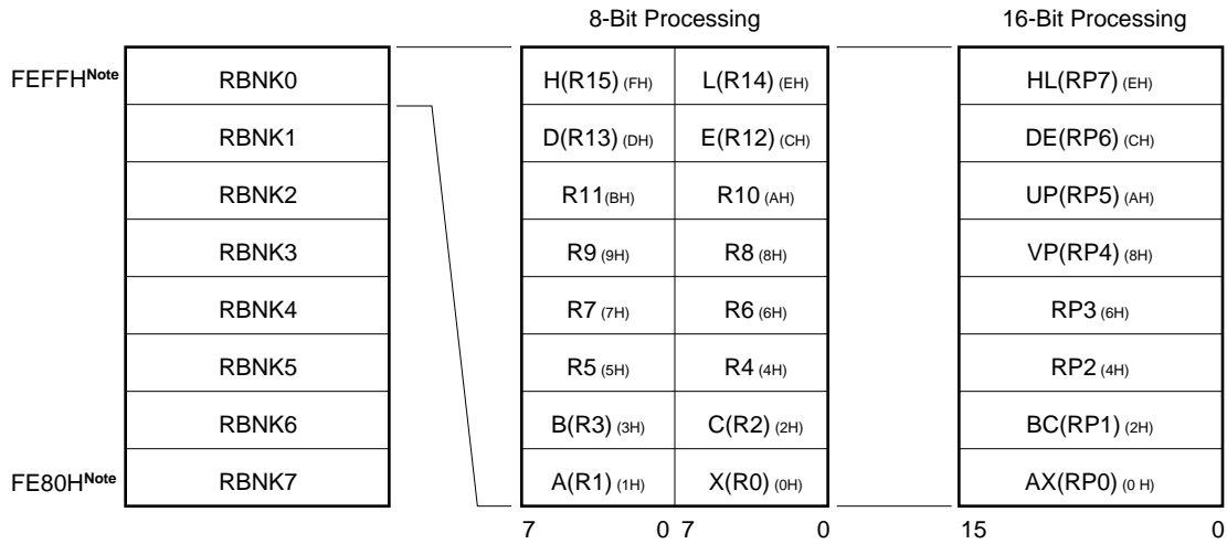
Figure 3-11. General-Purpose Register Addresses
