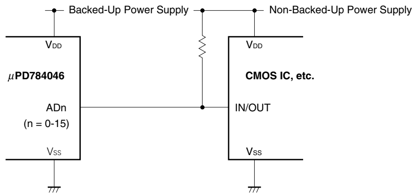
Figure 18-6. Example of Address/Data Bus Processing
