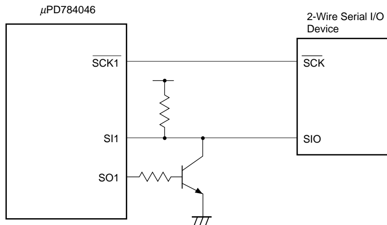
Figure 14-14. Example of Connection to 2-Wire Serial I/O
