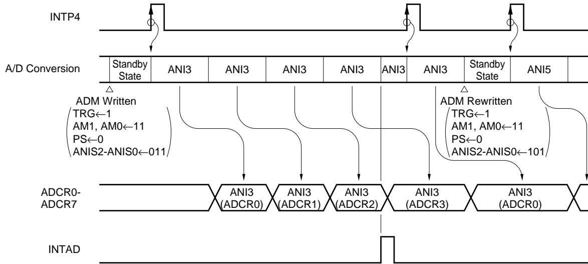
Figure 13-15. A/D Conversion in Select Mode (4-buffer mode) Started by Hardware
