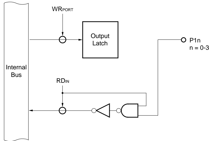
Figure 5-13. Port Specified as Input Port
