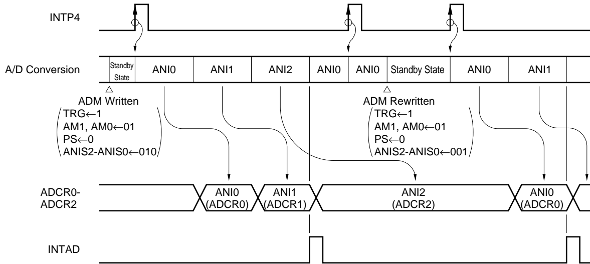
Figure 13-16. A/D Conversion in Scan Mode Started by Hardware
