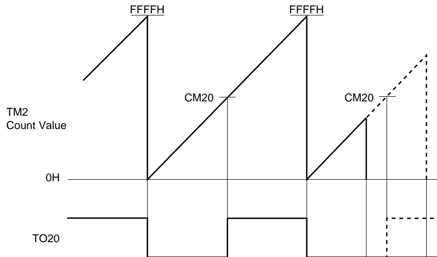
Figure 10-18. When Timer/Counter 2 is Stopped During PWM Signal Output
