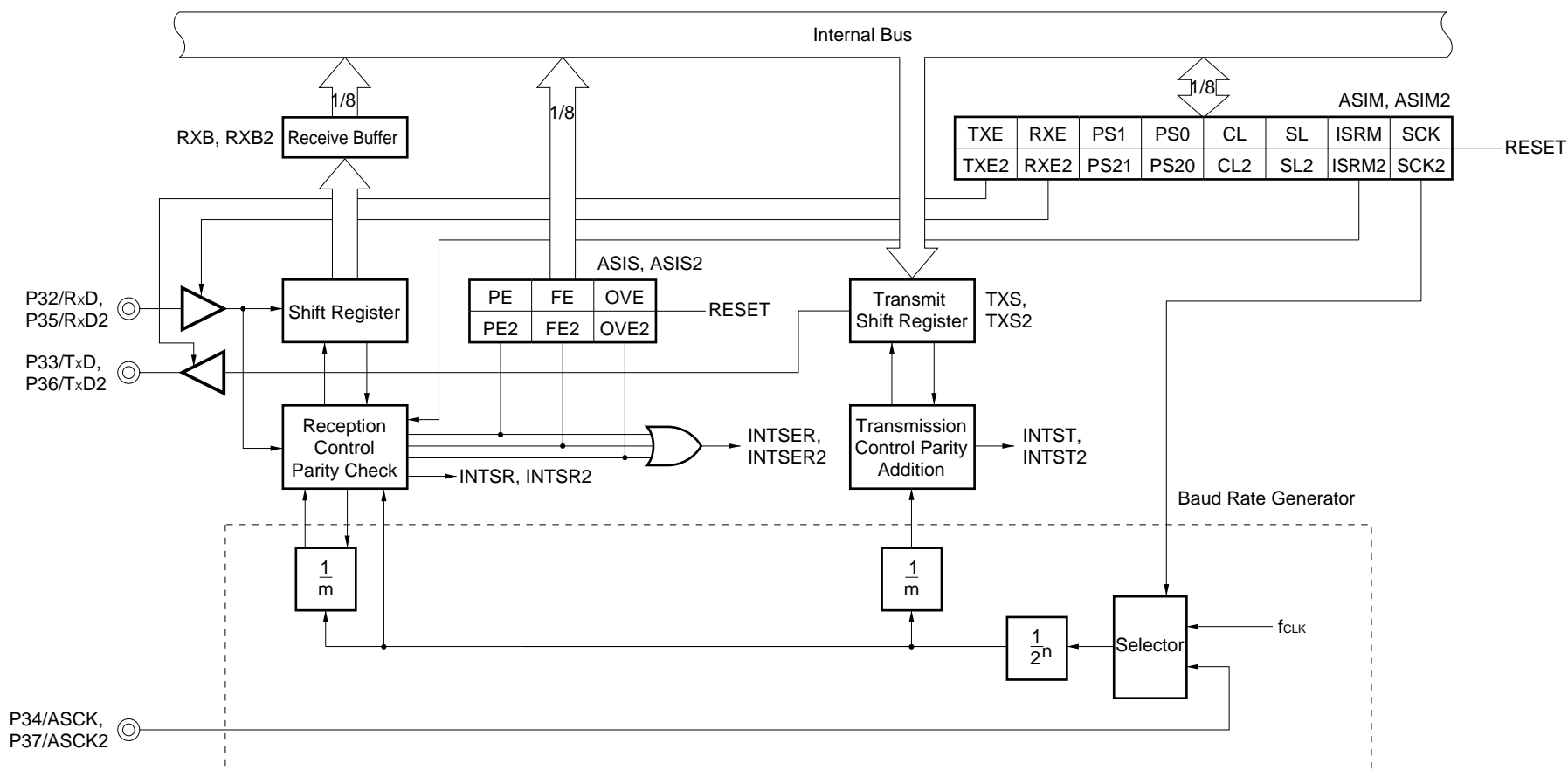
Figure 14-2. Block Diagram of Asynchronous Serial Interface
