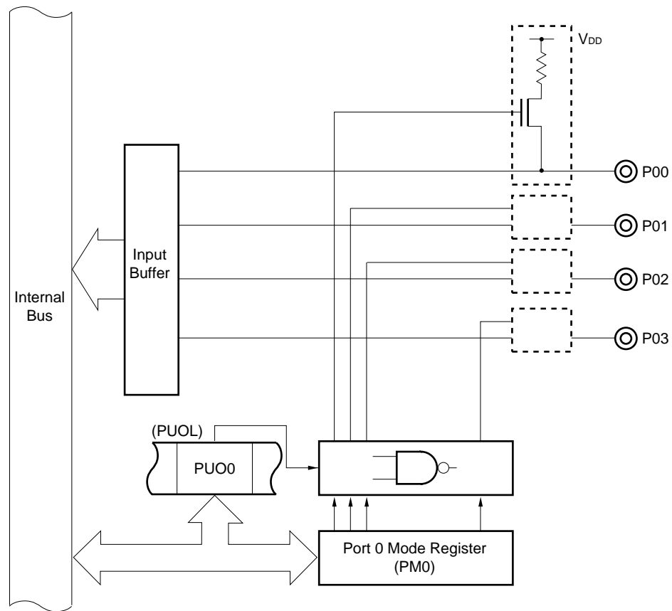
Figure 5-8. Pull-Up Resistor Specification (Port 0)
