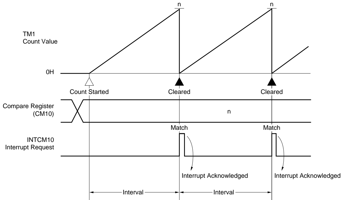
Figure 9-18. Timing of Interval Timer Operation (2)
