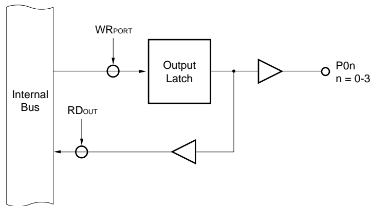
Figure 5-5. Port Specified as Output Port
