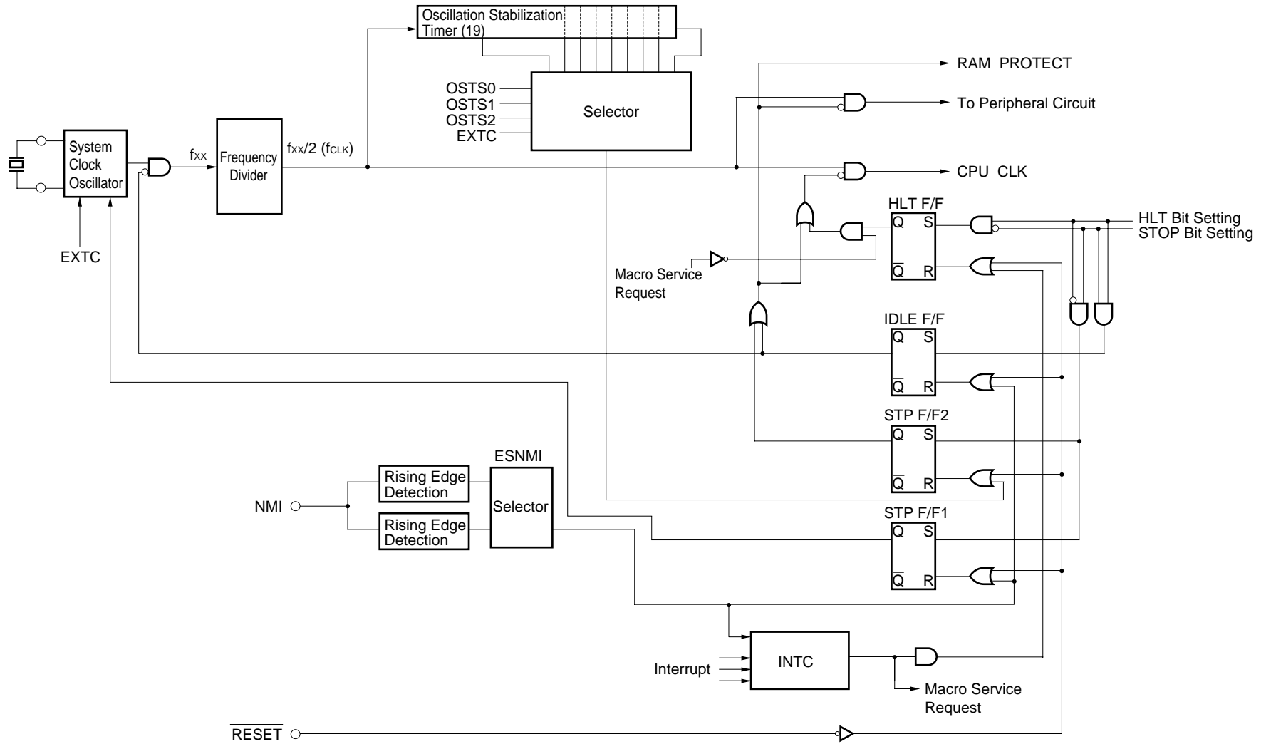
Figure 18-2. Diagram of Standby Function Block
