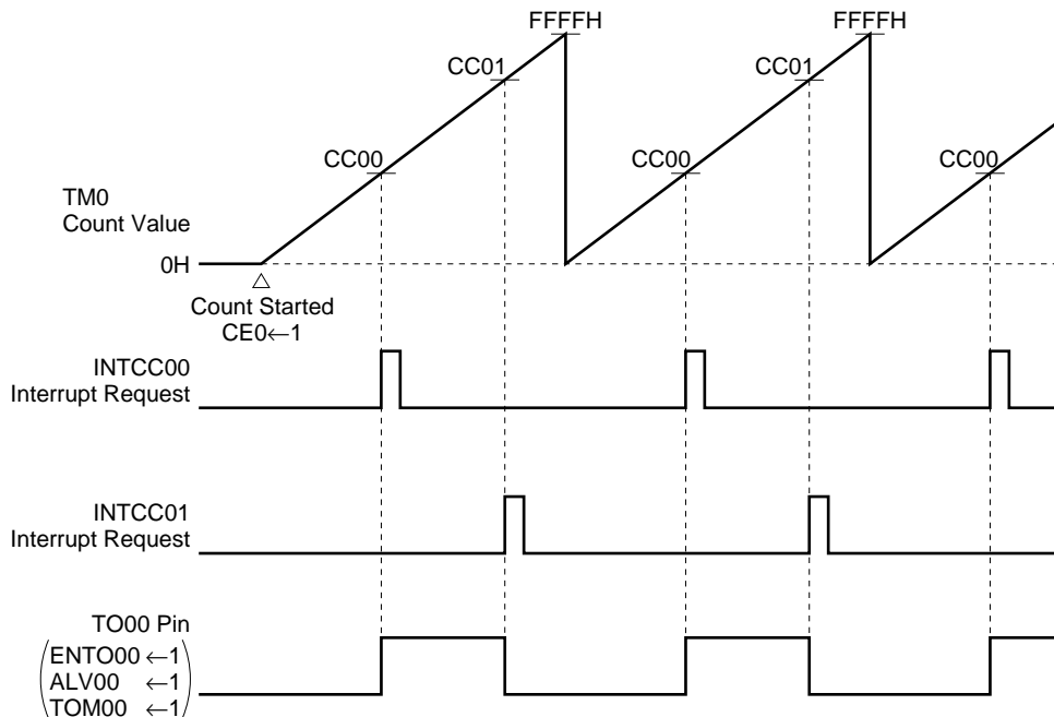
Figure 8-12. Operation of Set/Reset Output (timer 0)
