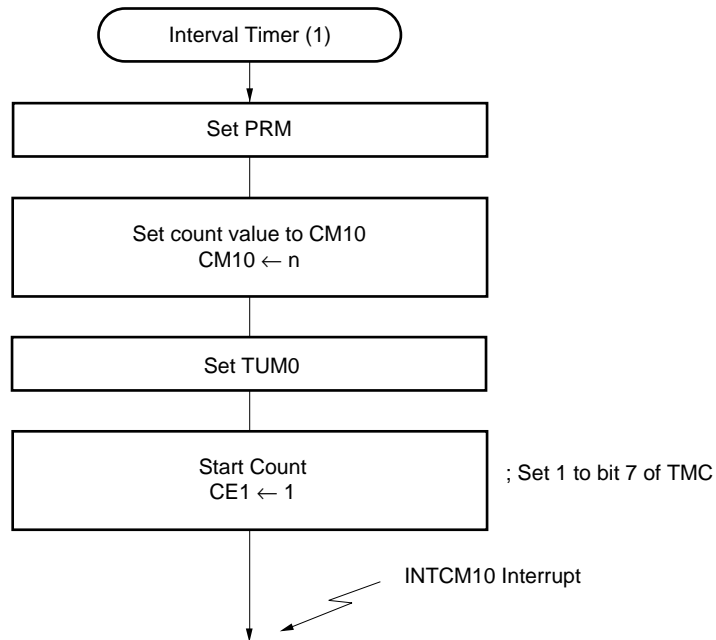
Figure 9-16. Setting Procedure of Interval Timer Operation (1)
