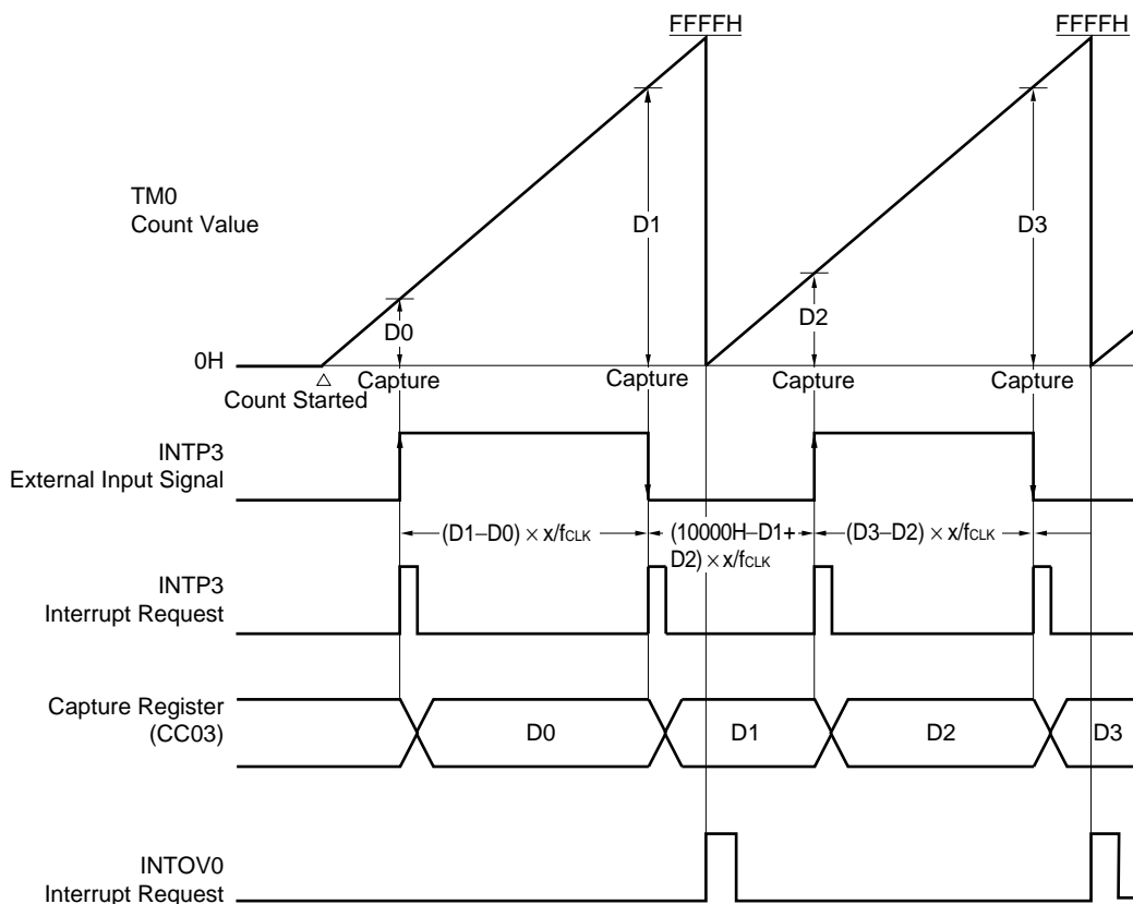
Figure 8-17. Timing of Pulse Width Measurement
