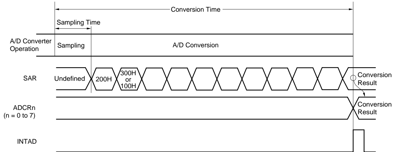
Figure 13-6. Basic Operation of A/D Converter
