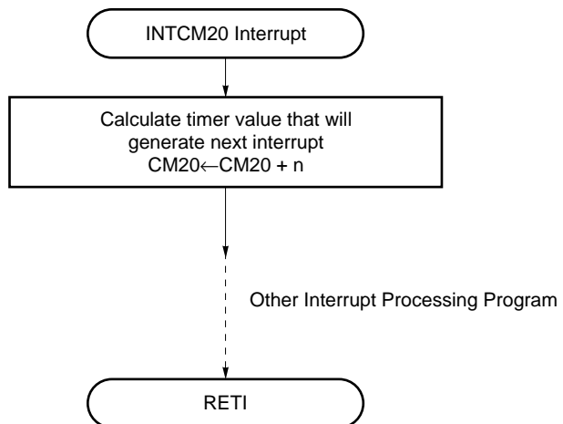
Figure 10-27. Interrupt Request Processing of Interval Timer Operation (1)
