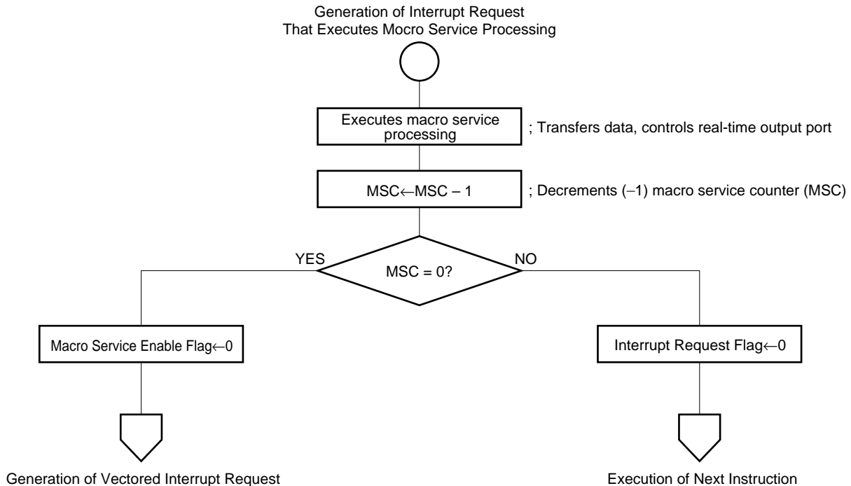
Figure 16-17. Example of Macro Service Processing Sequence
