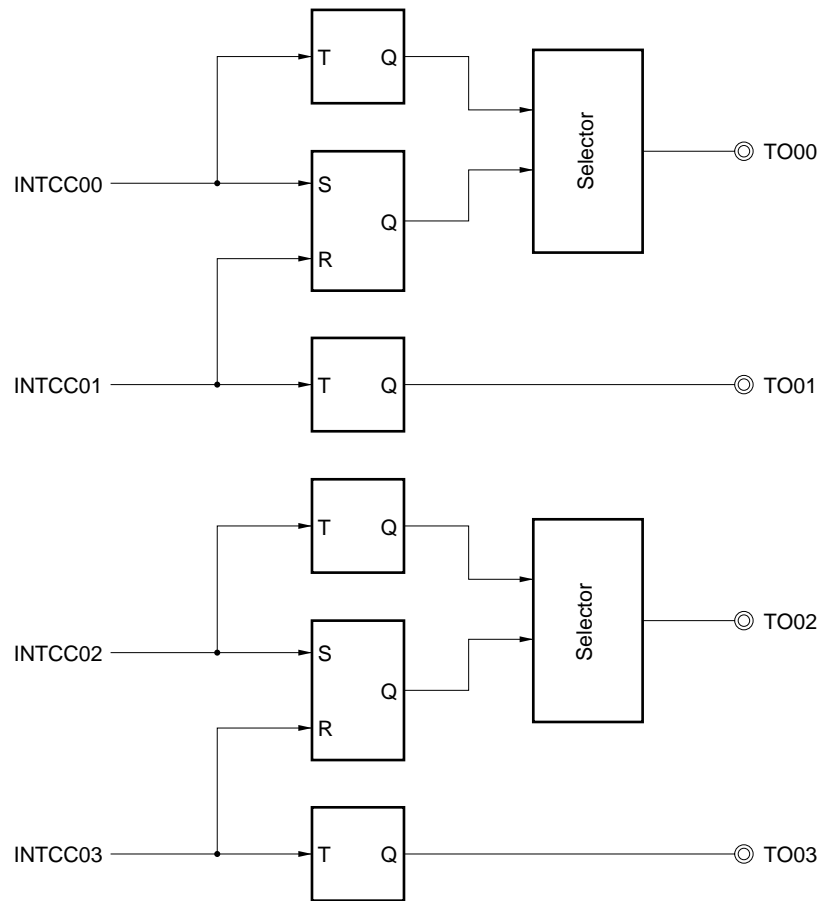
Figure 8-10. Block Diagram of Timer Output Operation of Timer 0
