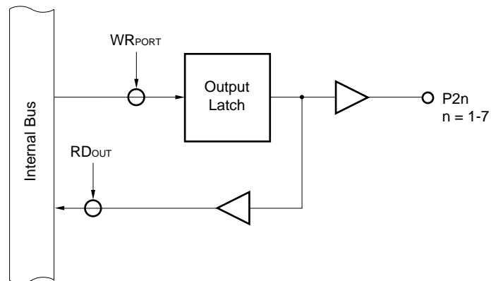
Figure 5-20. Port in Output Port Mode
