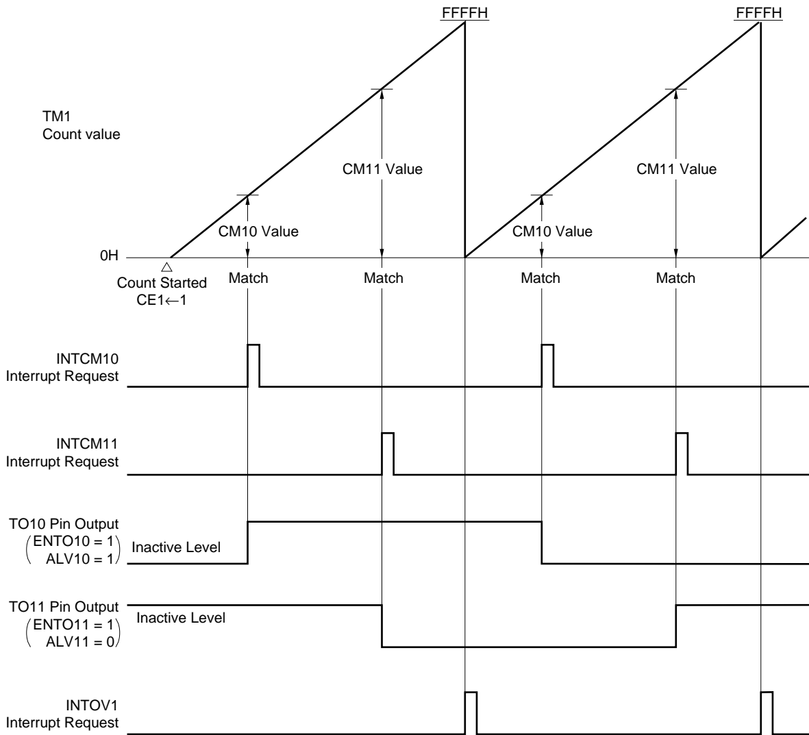
Figure 9-9. Compare Operation (timer 1)
