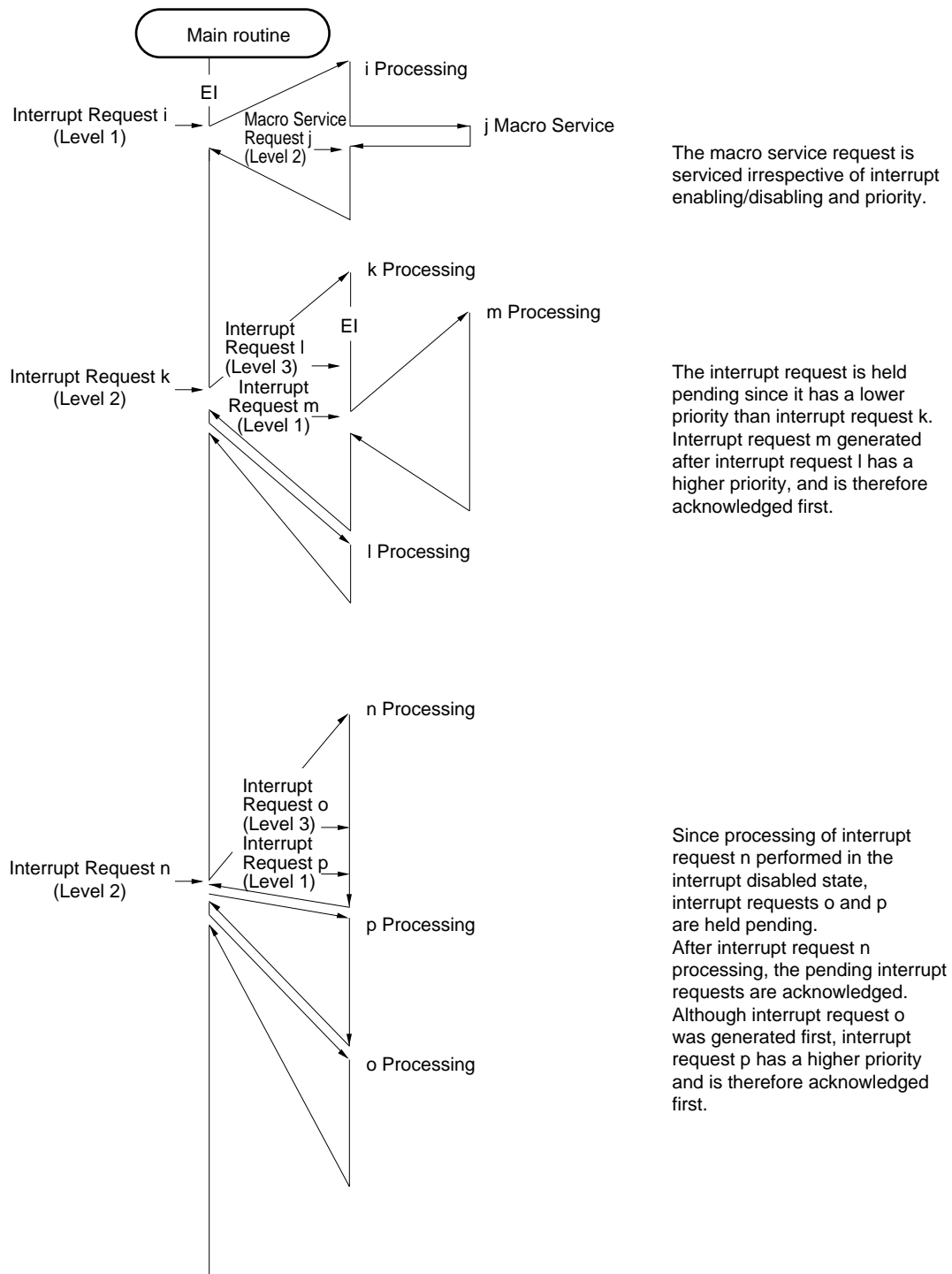
Figure 16-13. Examples of Processing When Another Interrupt Request Is Generated During Interrupt Processing (2/3)
