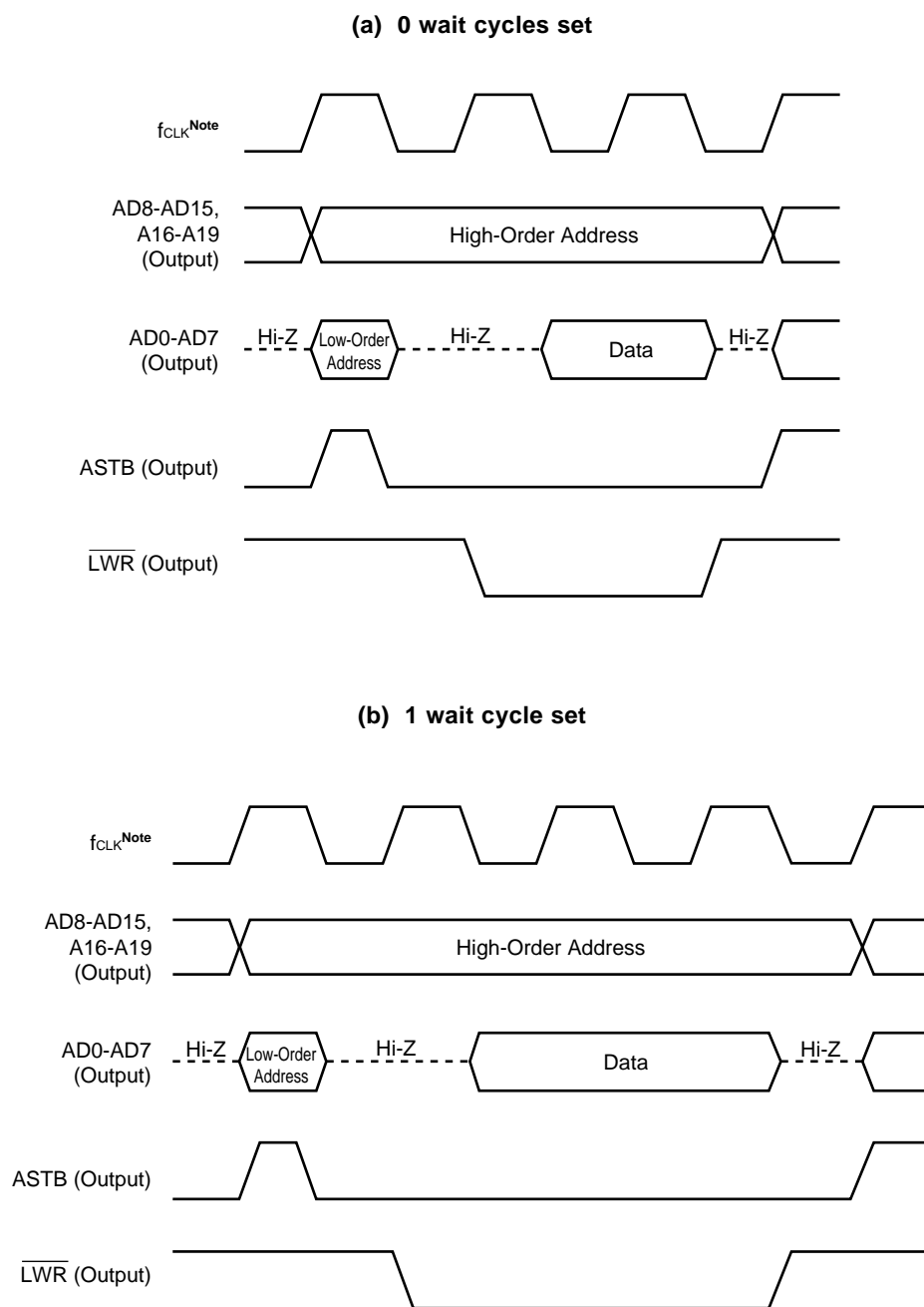
Figure 17-17. Write Timing of Access Wait Function (1/2)
