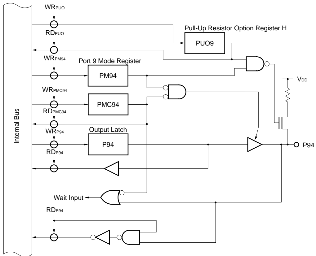
Figure 5-52. Block Diagram of P94 (Port 9)
