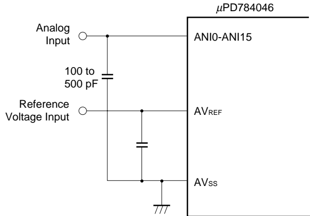
Figure 13-2. Example of Capacitor Connection on A/D Converter Pins
