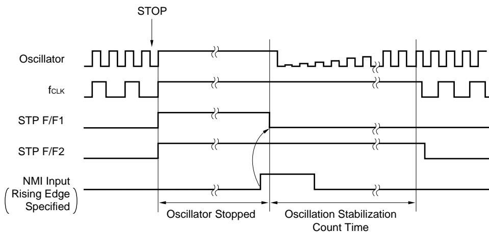
Figure 18-5. STOP Mode Release by NMI Input
