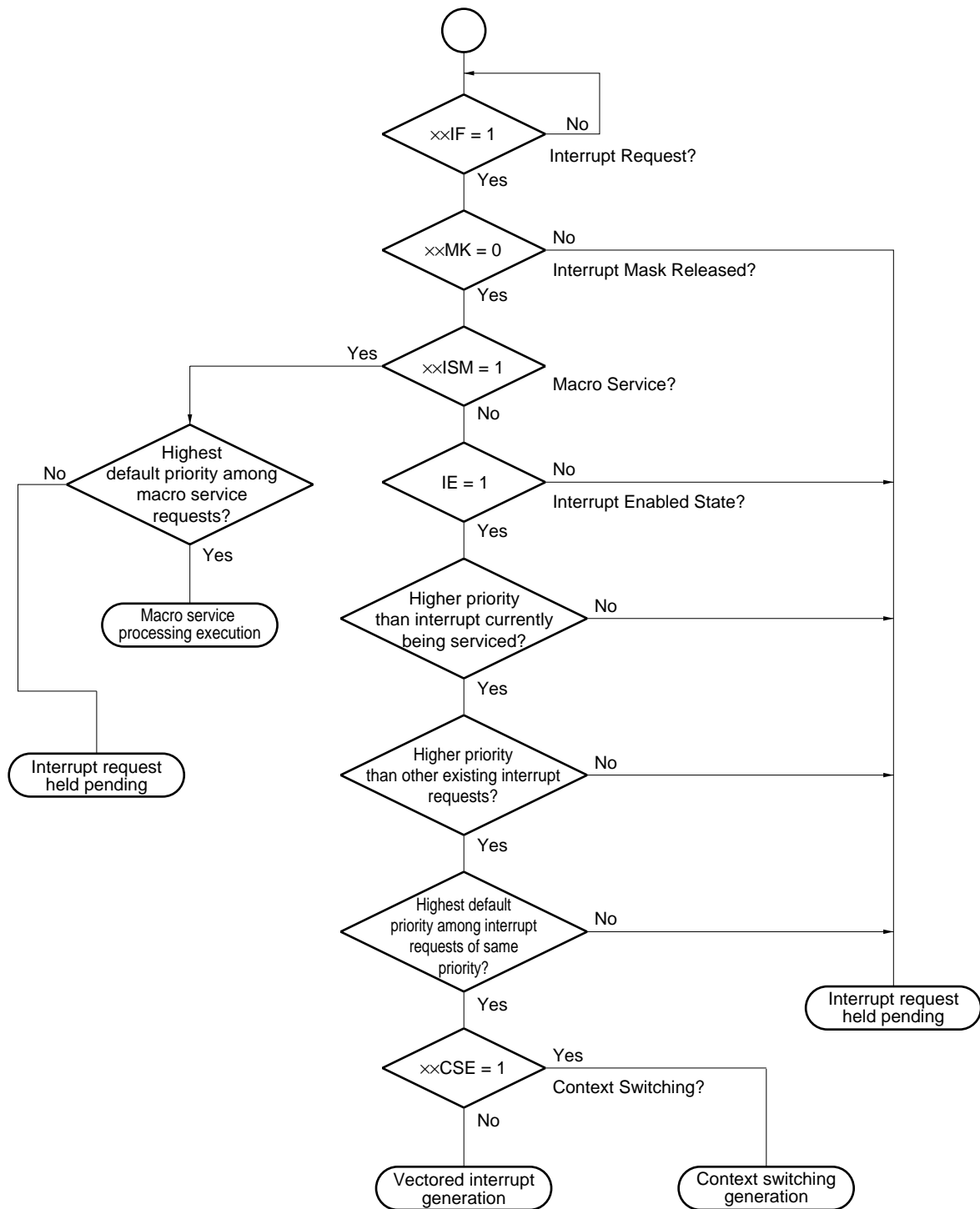
Figure 16-10. Algorithm of Interrupt Acknowledgment Processing
