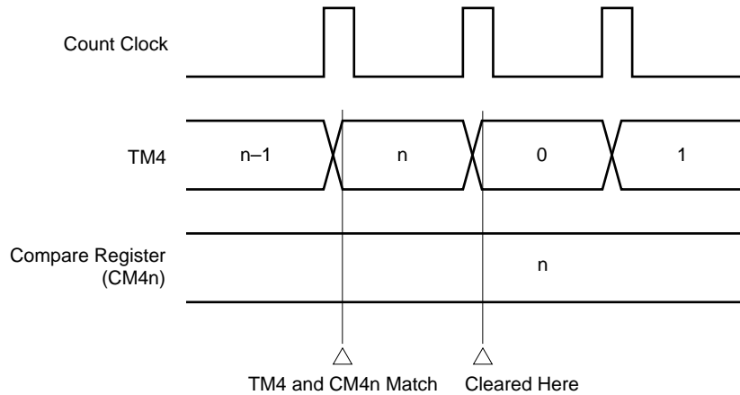
Figure 11-5. TM4 Clear Operation by Match with Compare Register (CM40, CM41)
