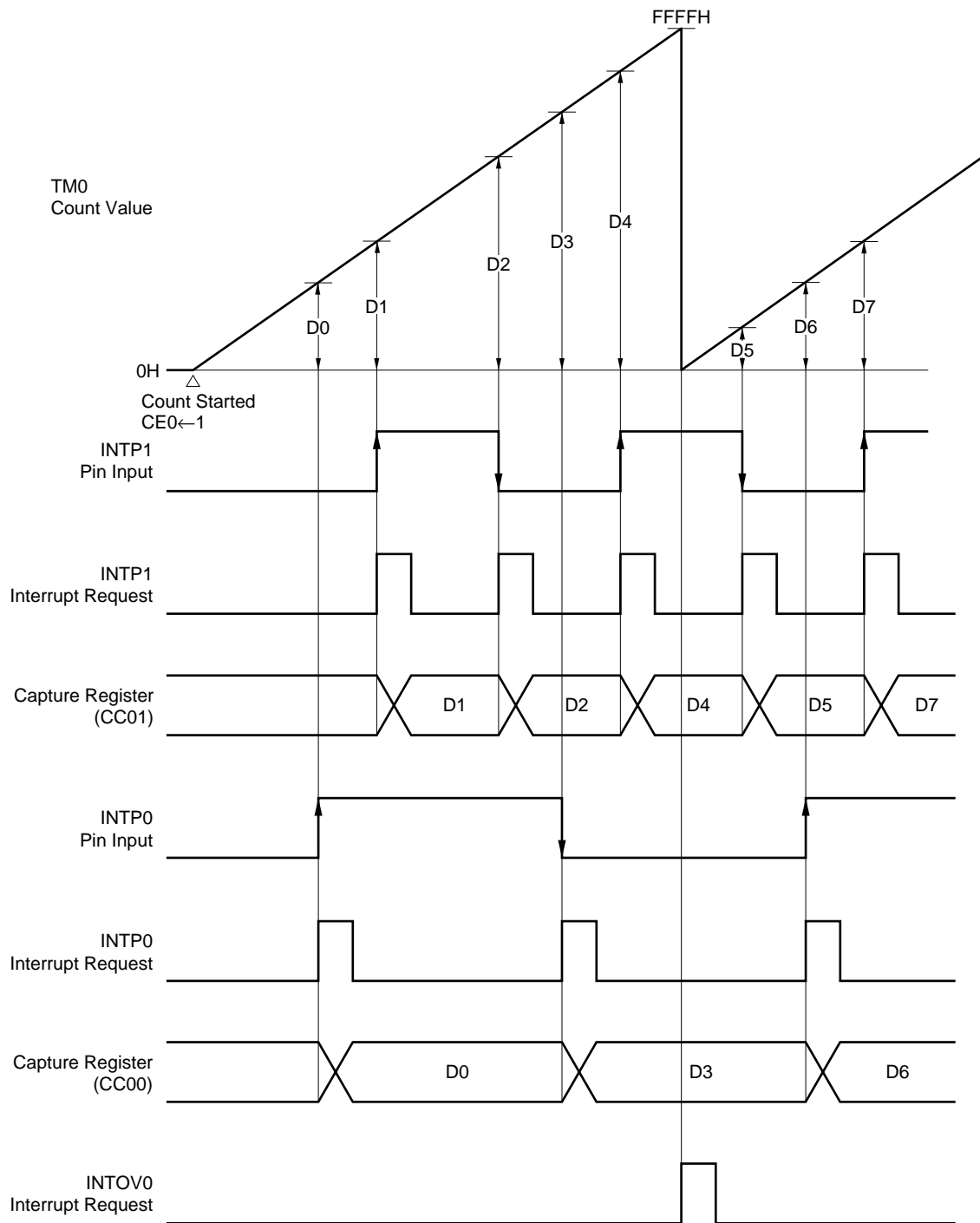
Figure 8-9. Capture Operation (timer 0)
