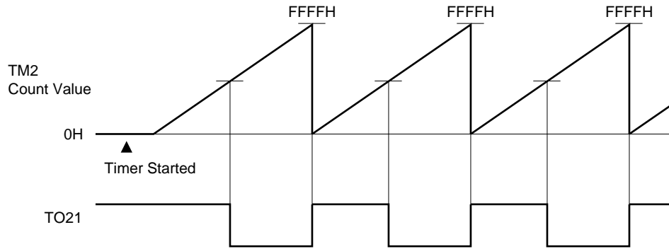
Figure 10-31. Example of Timer/Counter 2 PWM Signal Output
