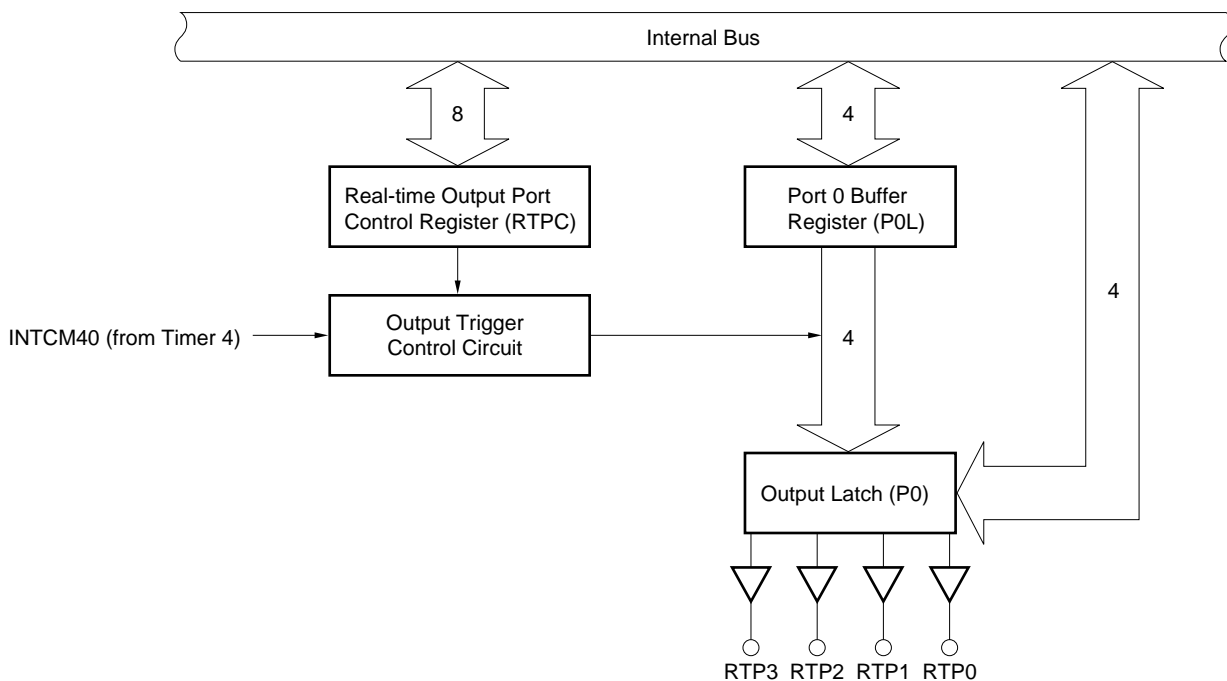
Figure 6-1. Block Diagram of Real-time Output Port
