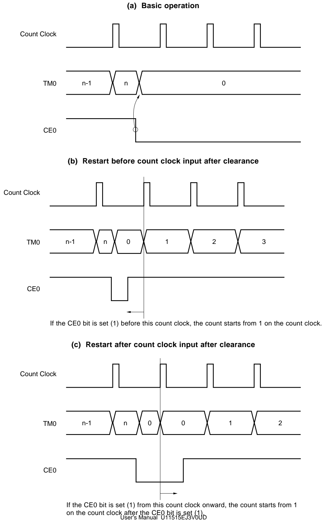
Figure 8-7. Clear Operation of Timer Register 0 (TM0)
