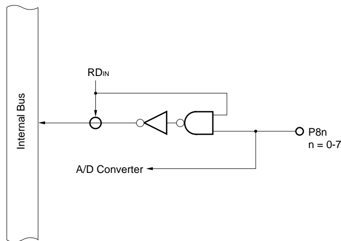
Figure 5-50. Block Diagram of Port 8
