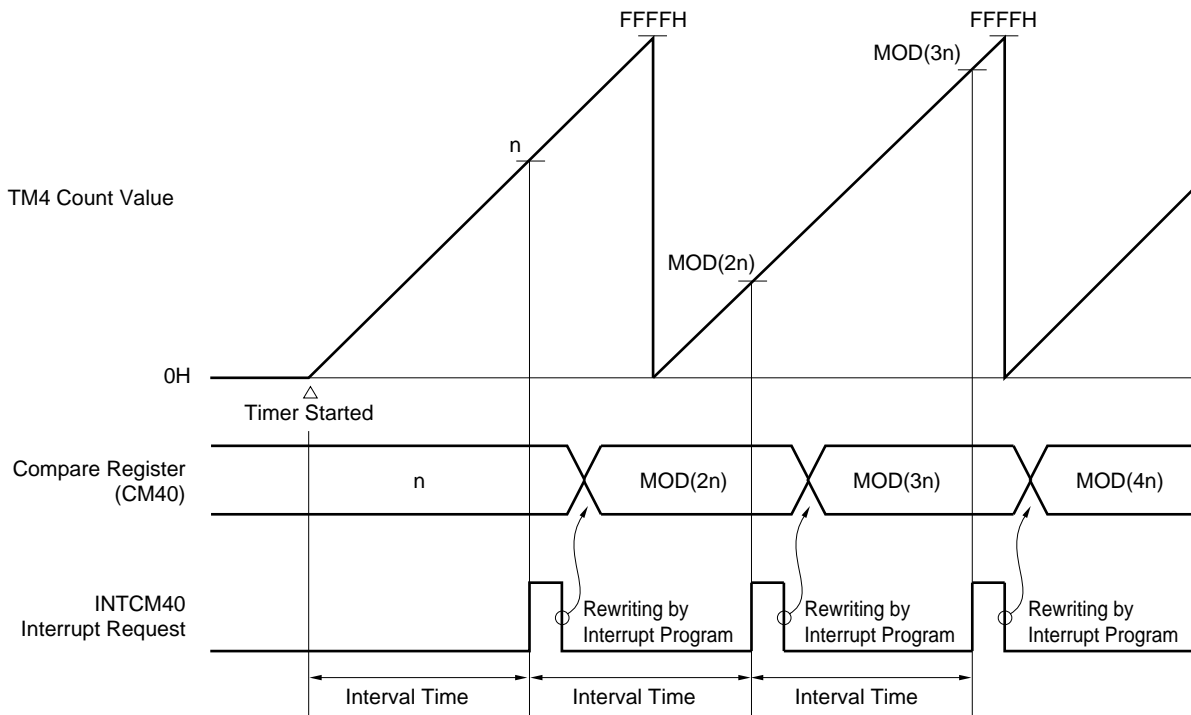
Figure 11-9. Timing of Interval Timer Operation (1)
