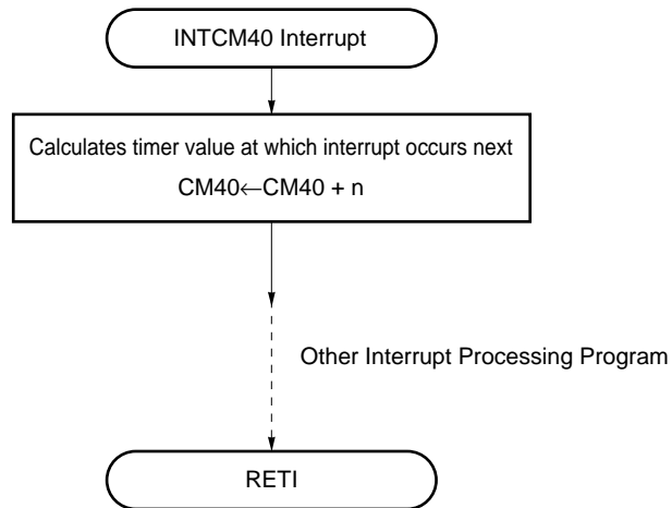
Figure 11-12. Interrupt Request Processing of Interval Timer Operation (1)
