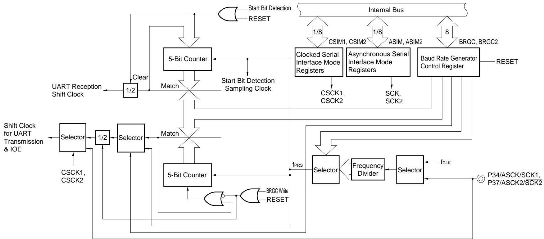
Figure 14-15. Block Diagram of Baud Rate Generator
