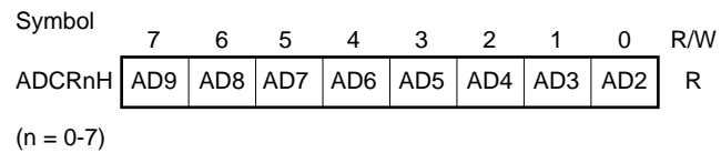
Figure 13-5. Byte Access to A/D Conversion Result Register
