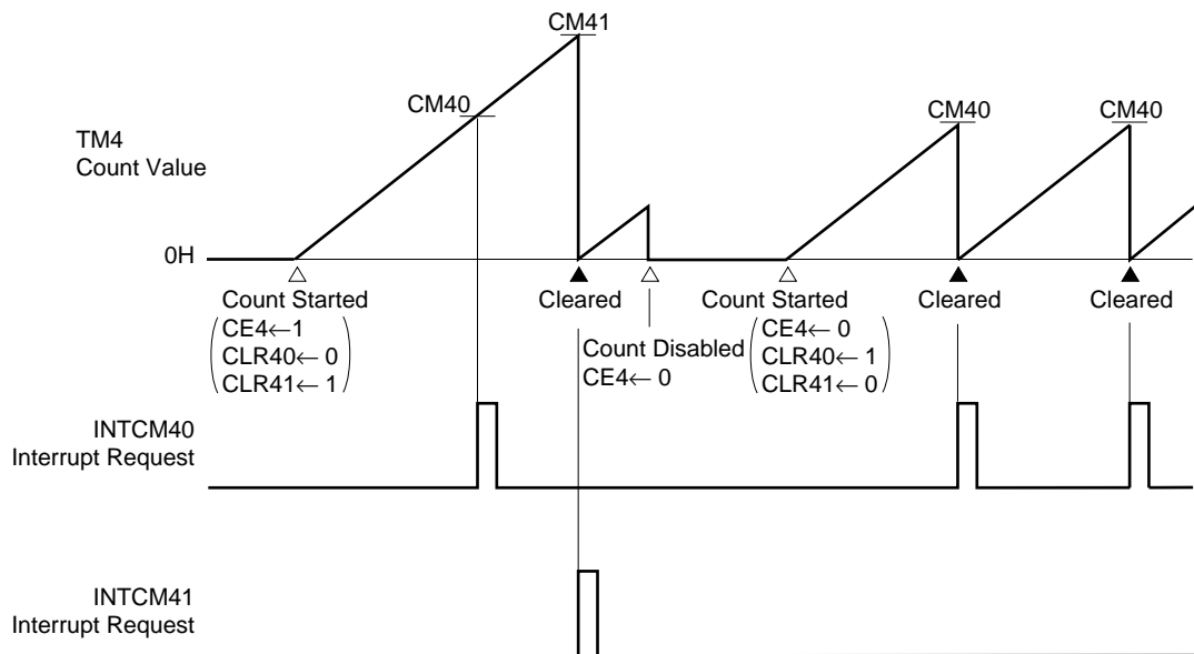
Figure 11-8. TM4 Clearance after Match Detection
