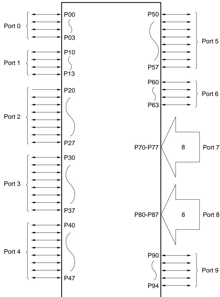
Figure 5-1. Port Configuration
