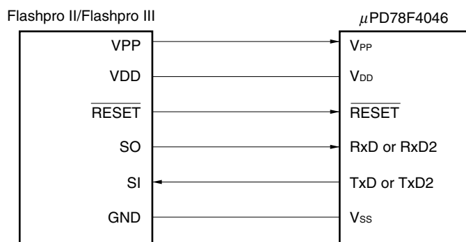
Figure 20-3. Connecting Flashpro II/Flashpro III in UART Mode
