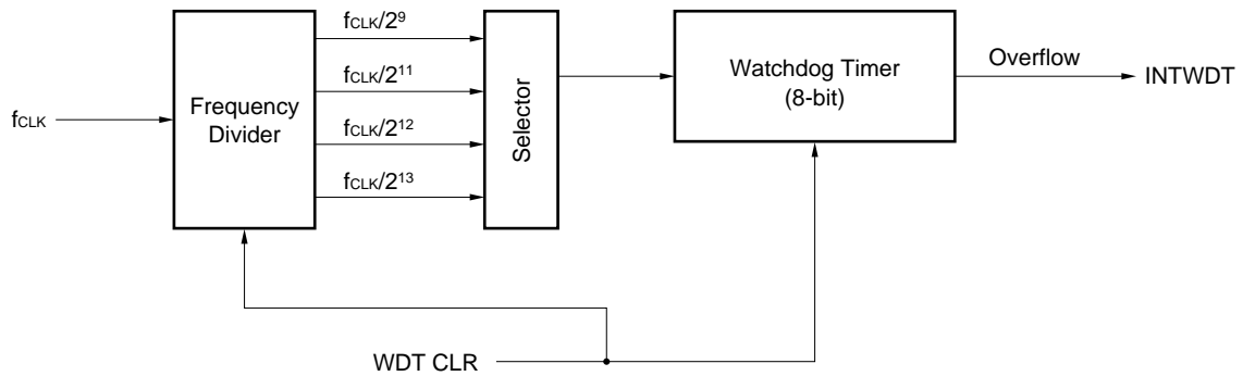
Figure 12-1. Block Diagram of Watchdog Timer
