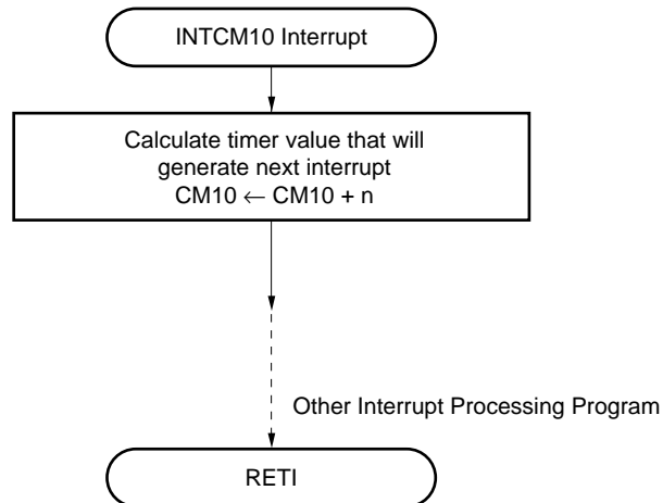
Figure 9-17. Interrupt Request Processing of Interval Timer Operation (1)
