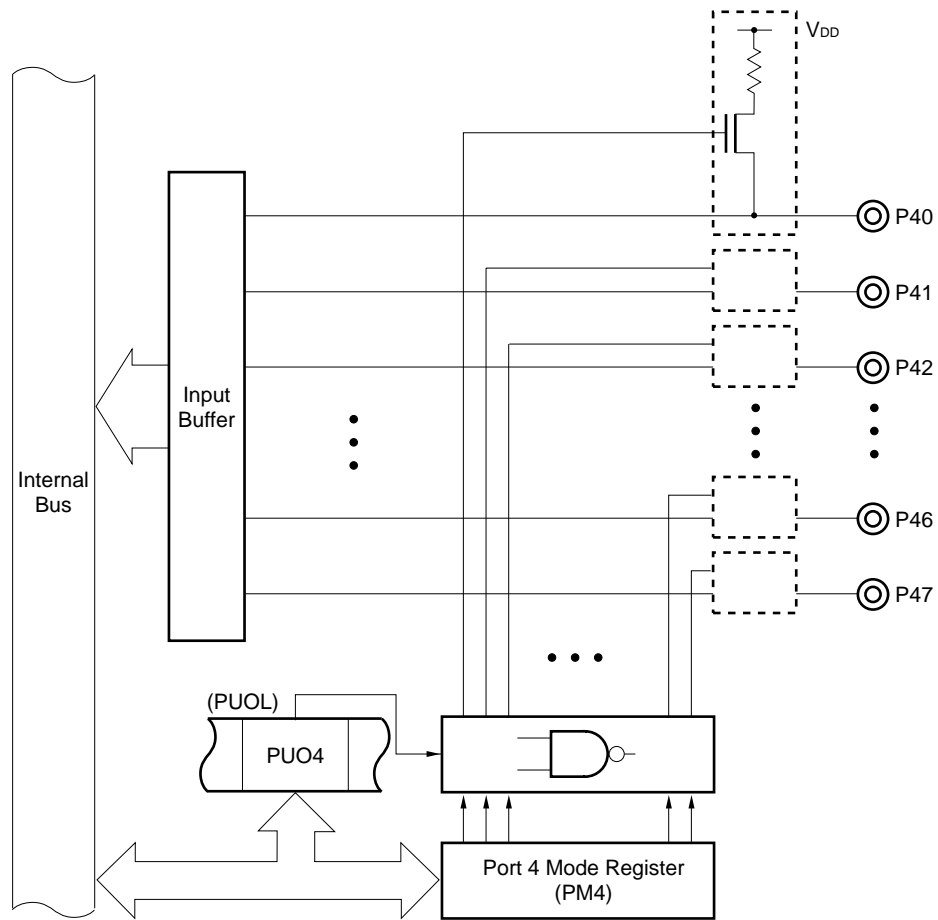
Figure 5-36. Pull-Up Resistor Specification (Port 4)
