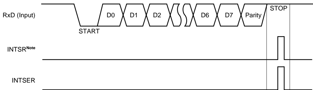
Figure 14-8. Timing of Receive Error
