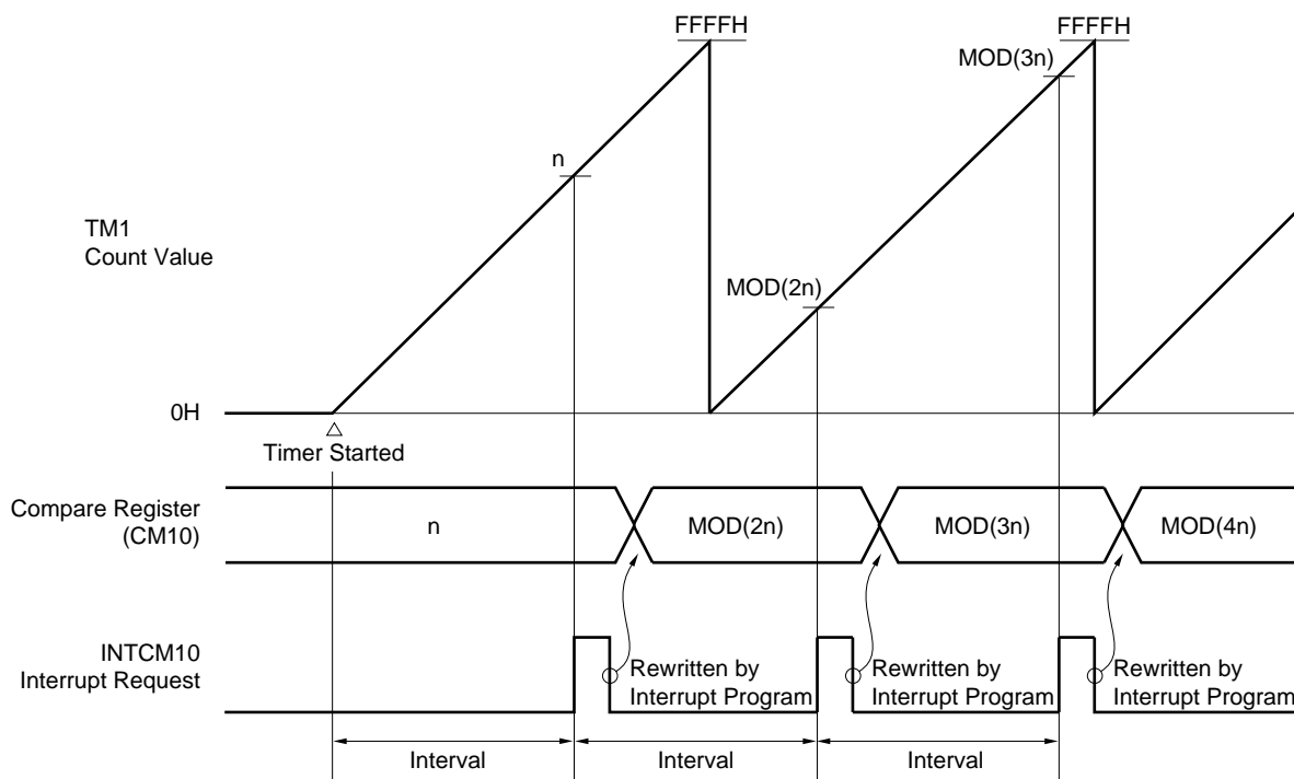
Figure 9-14. Timing of Interval Timer Operation (1)
