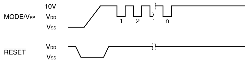
Figure 20-1. Selecting Format of Communication Mode
