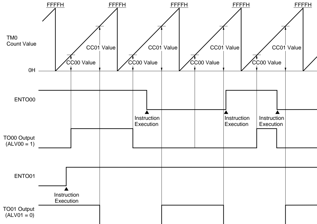
Figure 8-11. Operation of Toggle Output
