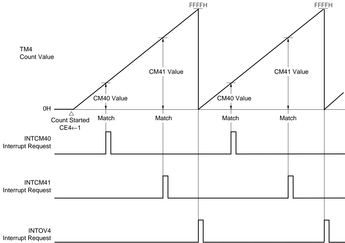
Figure 11-7. Compare Operation (timer 4)
