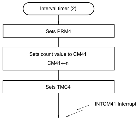
Figure 11-15. Setting Procedure of Interval Timer Operation (2)
