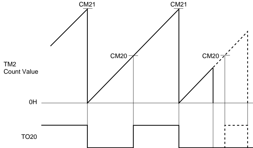
Figure 10-23. When Timer/Counter 2 is Stopped During PPG Signal Output
