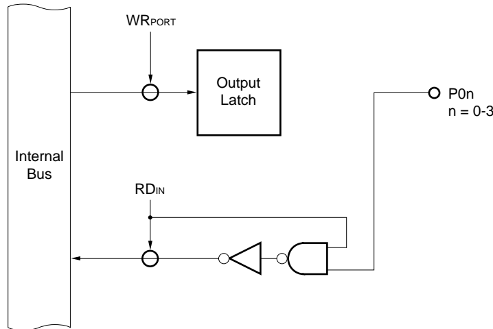
Figure 5-6. Port Specified as Input Port
