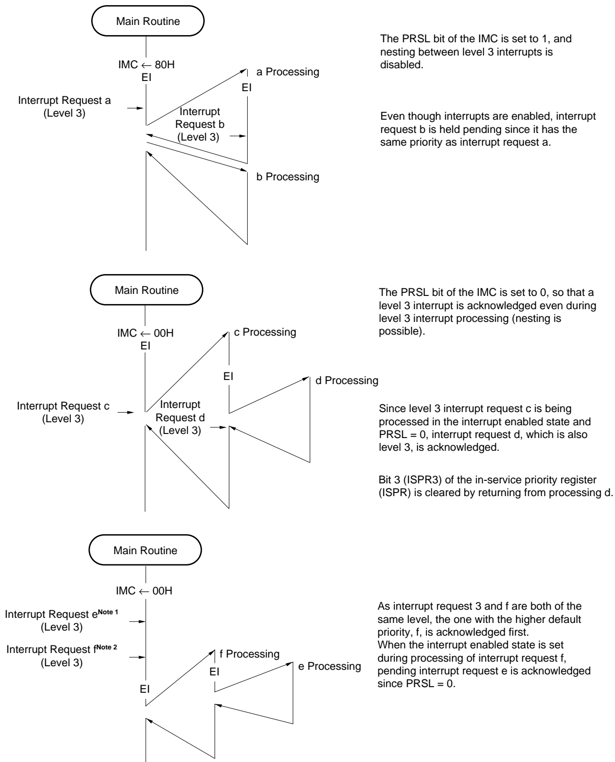
Figure 16-15. Differences in Level 3 Interrupt Acknowledgment According to Setting of Interrupt Mode Control Register (IMC)
