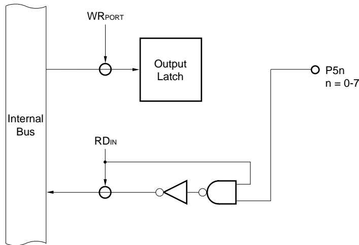
Figure 5-40. Port Specified as Input Port
