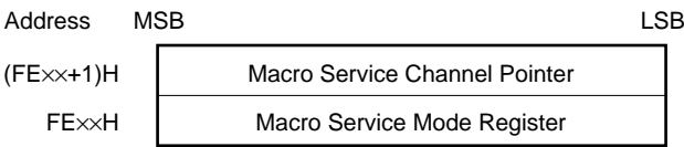
Figure 16-19. Basic Configuration of Macro Service Control Word
