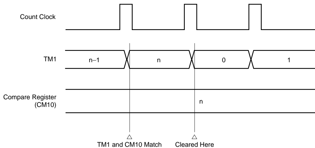
Figure 9-7. TM1 Clear Operation by Match with Compare Register (CM10)
