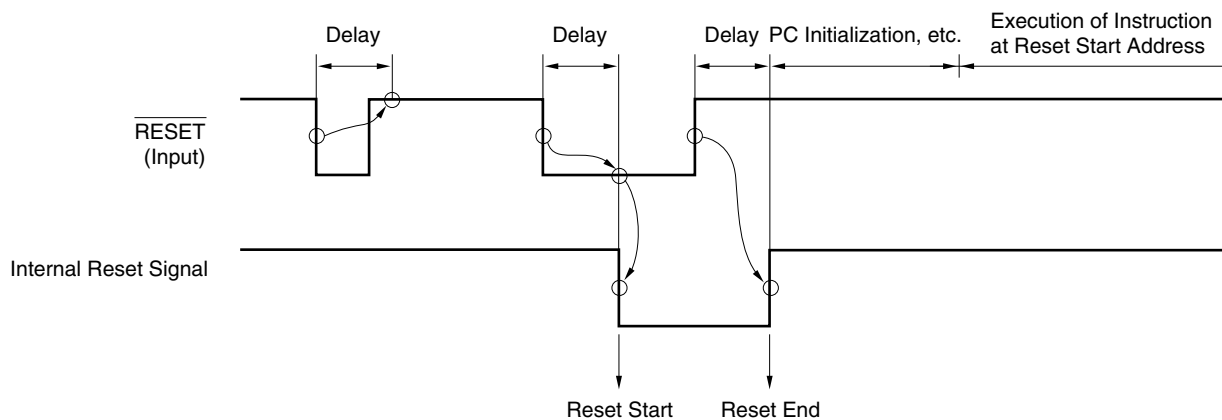
Figure 19-1. Acknowledgment of Reset Signal
