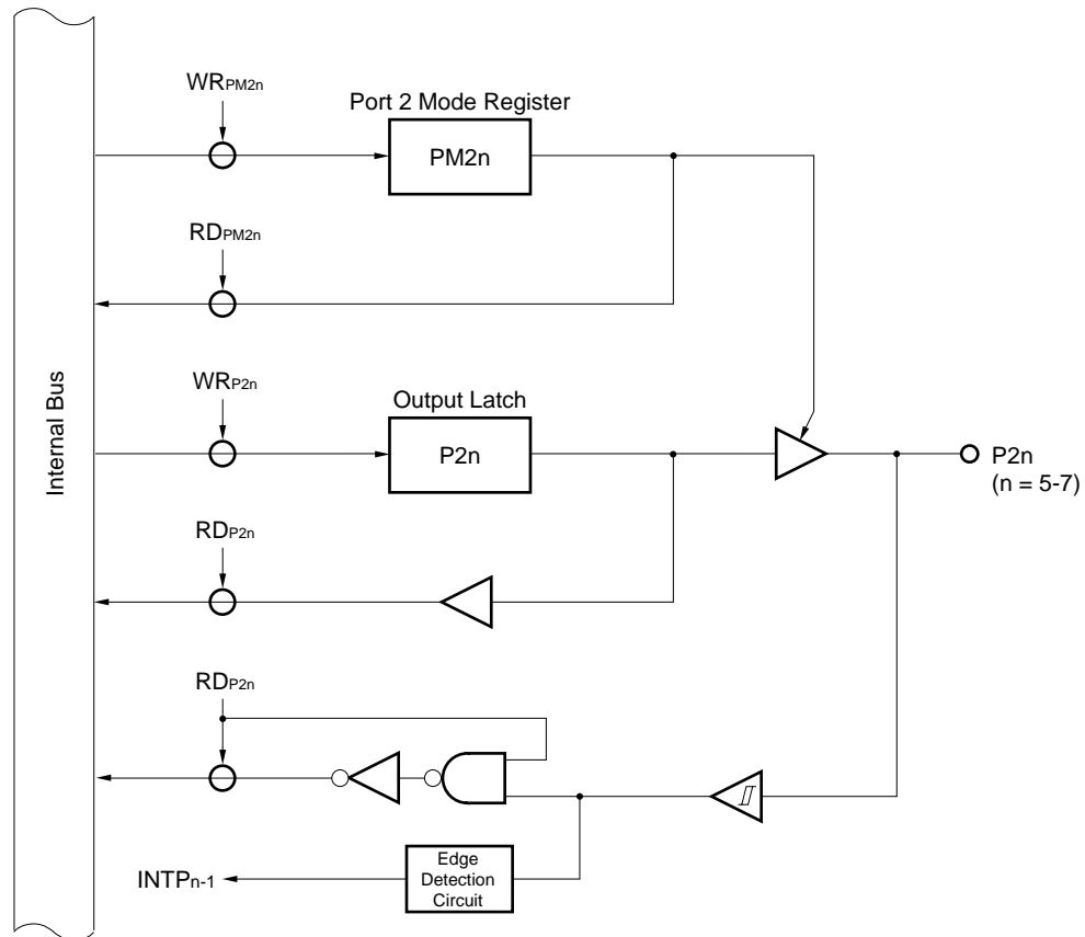
Figure 5-17. Block Diagram of P25 to P27 (Port 2)
