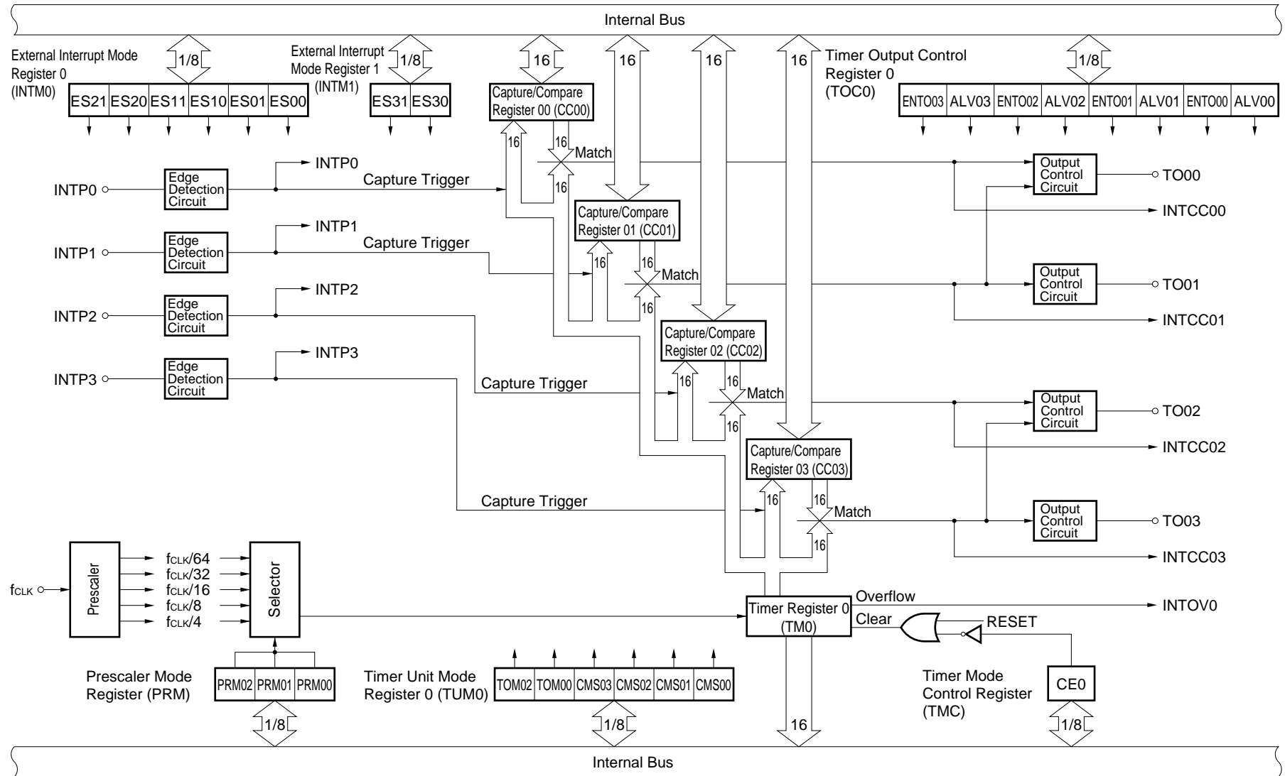
Figure 8-1. Block Diagram of Timer 0
