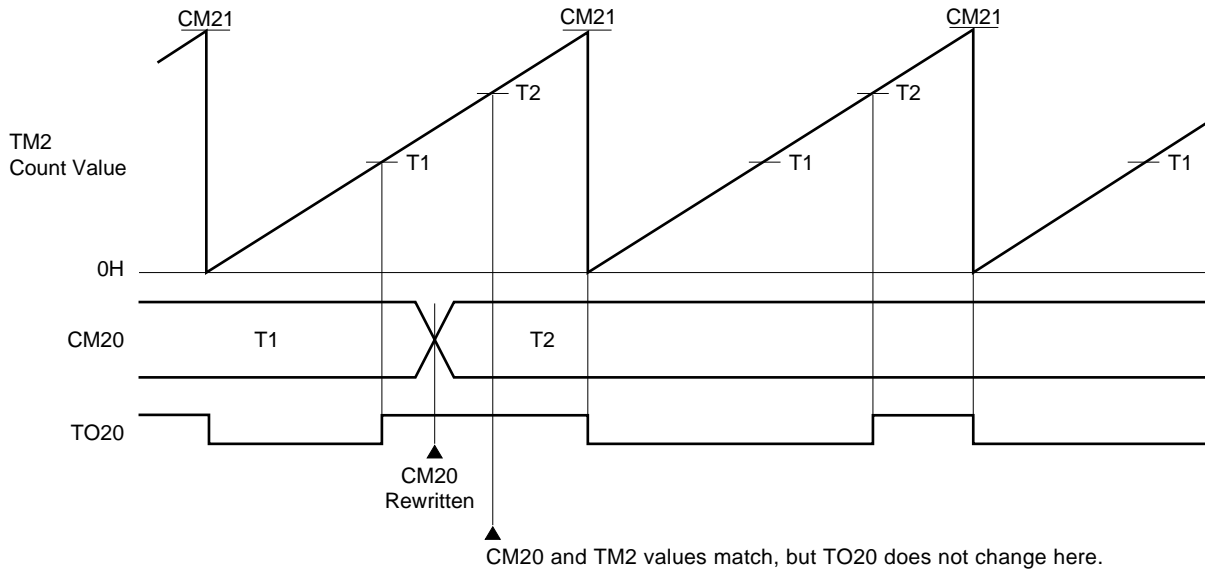
Figure 10-20. Example of Compare Register (CM20) Rewrite
