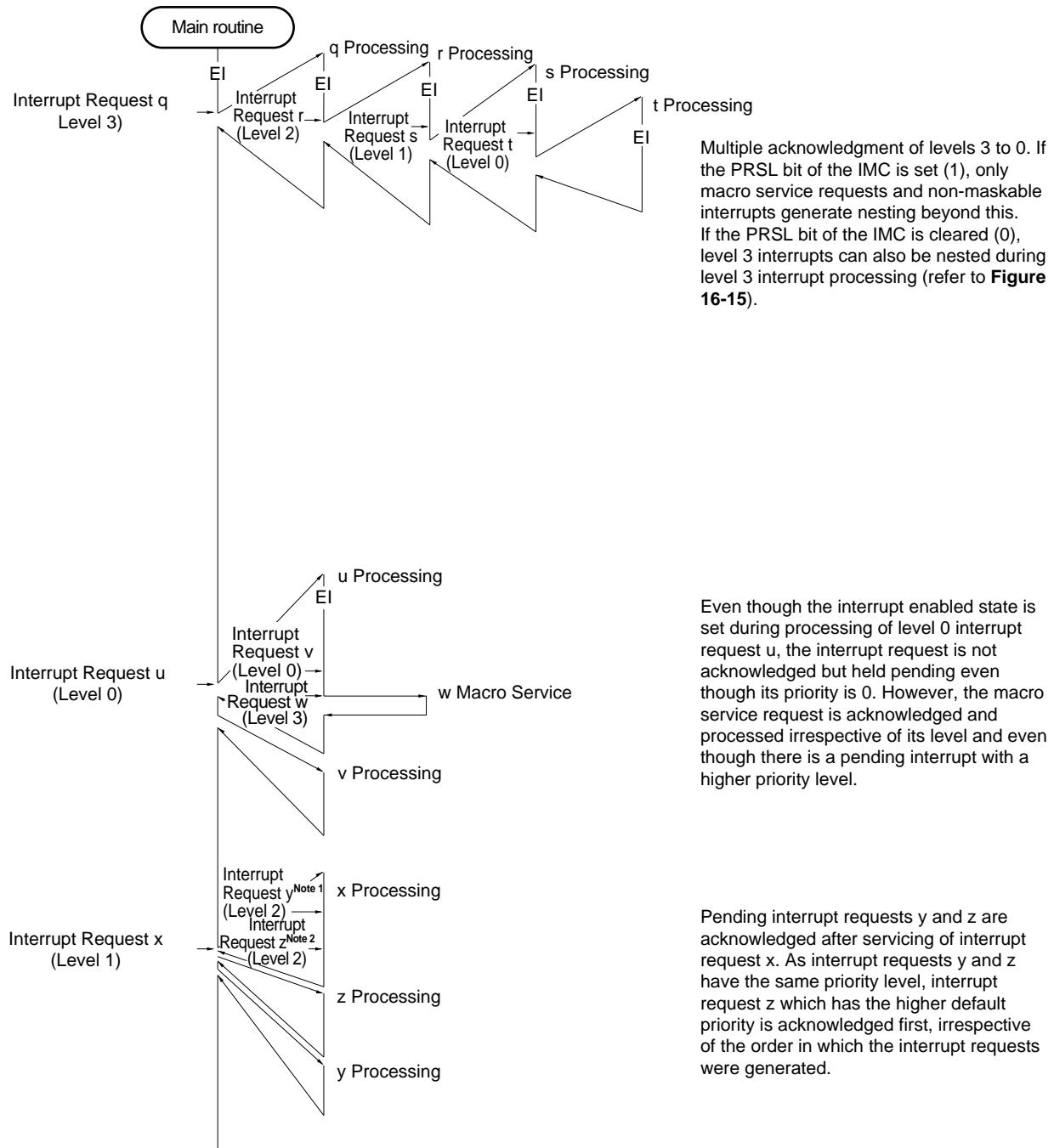
Figure 16-13. Examples of Processing When Another Interrupt Request Is Generated During Interrupt Processing (3/3)
