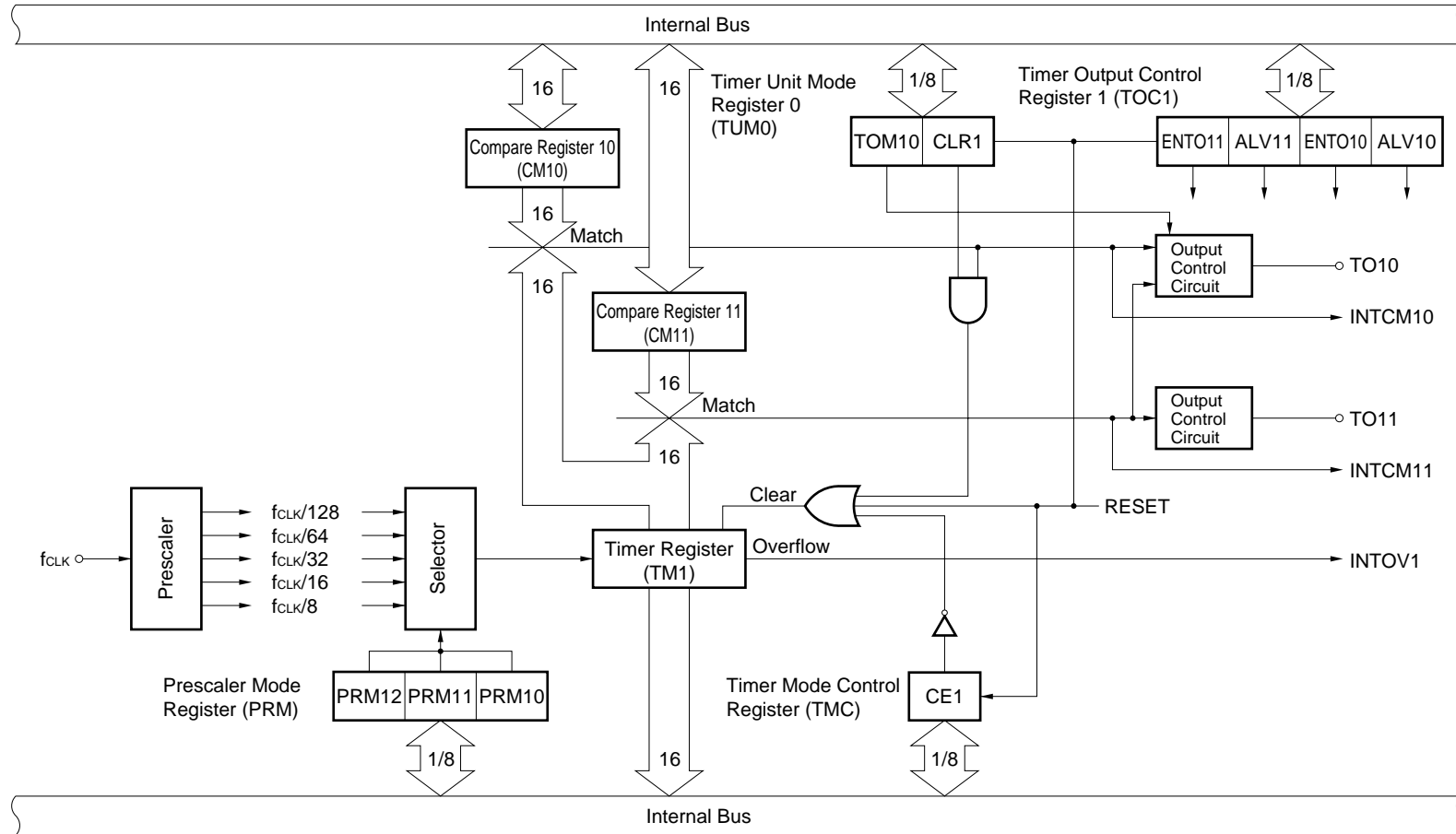
Figure 9-1. Block Diagram of Timer 1
