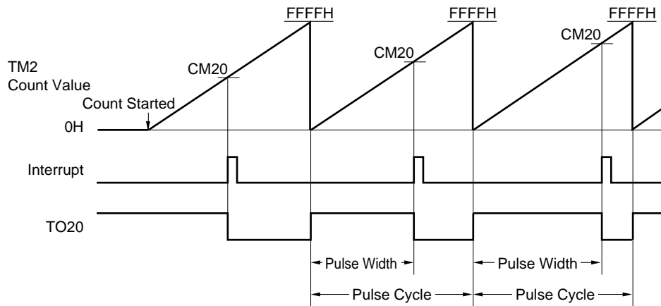
Figure 10-13. PWM Pulse Output
