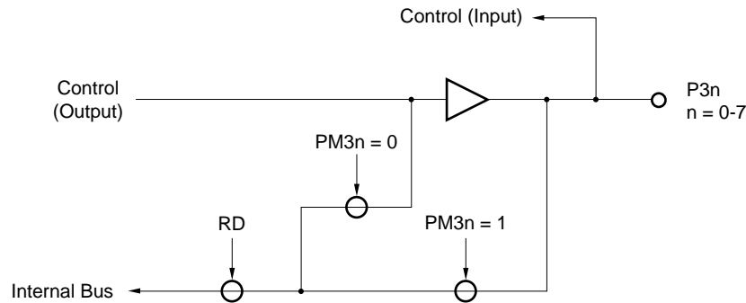
Figure 5-30. Control Specification
