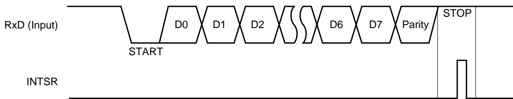
Figure 14-7. Interrupt Timing of Asynchronous Serial Interface Reception Completion
