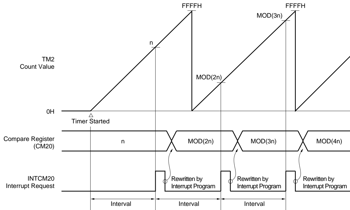
Figure 10-24. Timing of Interval Timer Operation (1)
