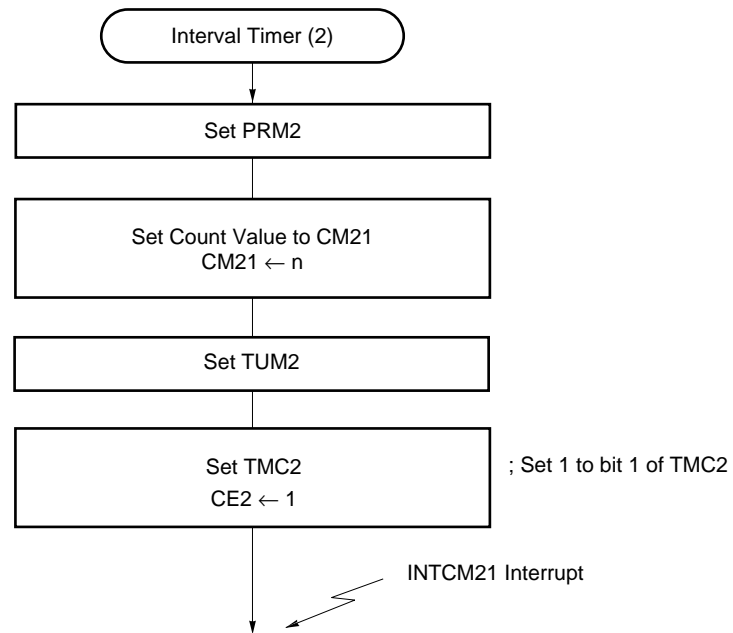
Figure 10-30. Setting Procedure of Interval Timer Operation (2)
