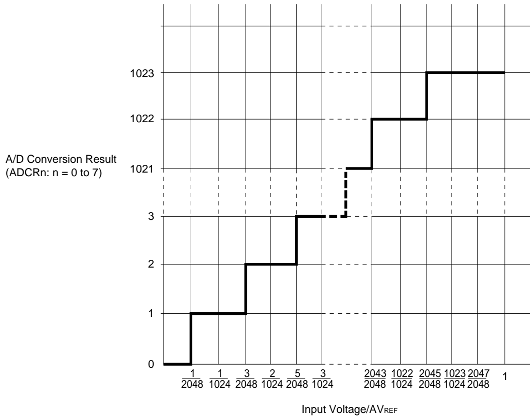
Figure 13-7. Relationship Between Analog Input Voltage and A/D Conversion Result
