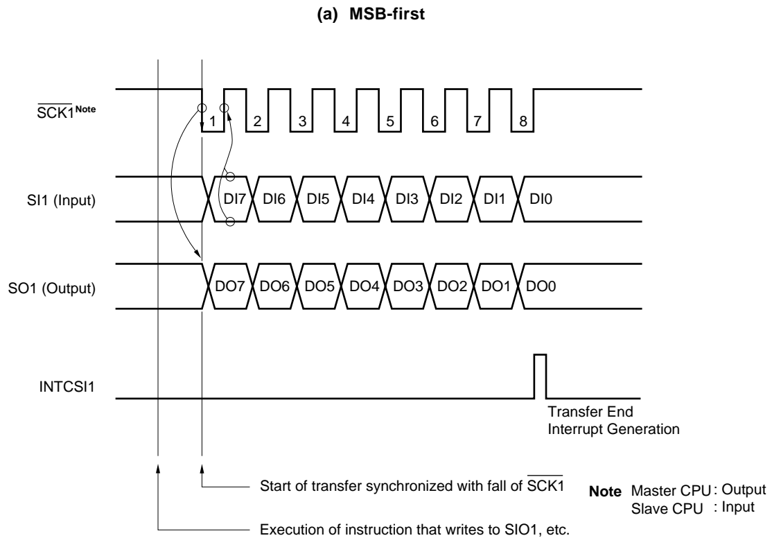
Figure 14-13. Timing of 3-Wire Serial I/O Mode (1/2)
