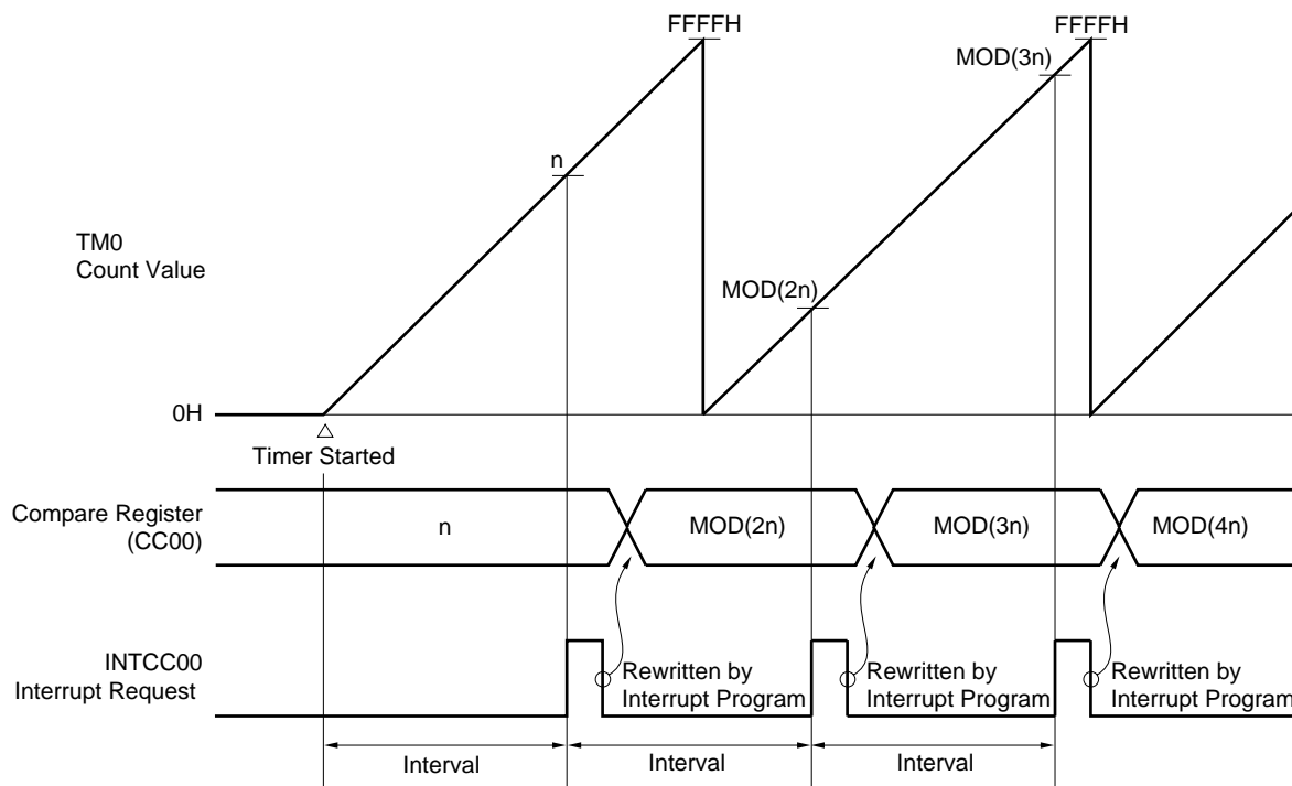
Figure 8-13. Timing of Interval Timer Operation
