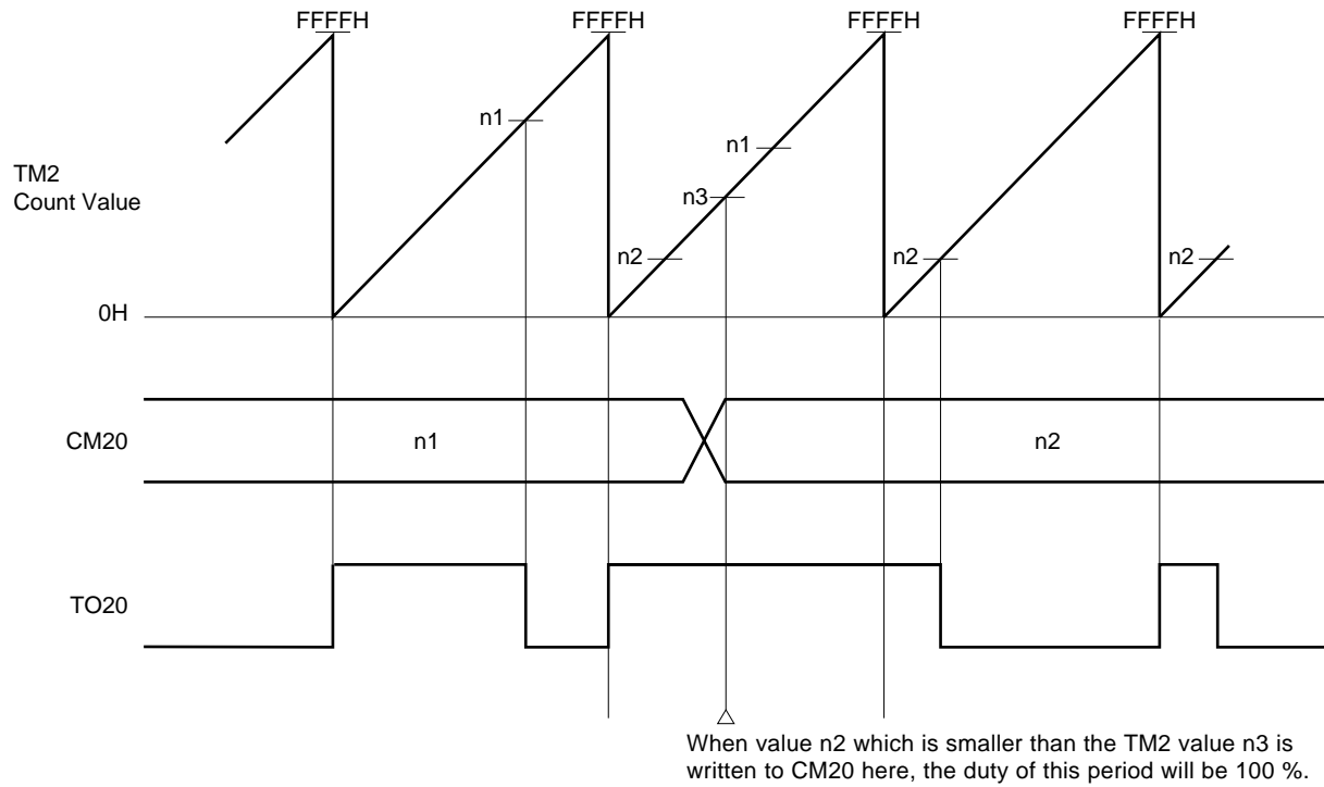
Figure 10-17. Example of 100 % Duty With PWM Output
