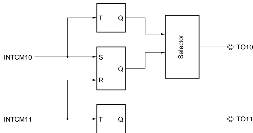
Figure 9-11. Block Diagram of Timer Output Operation of Timer 1
