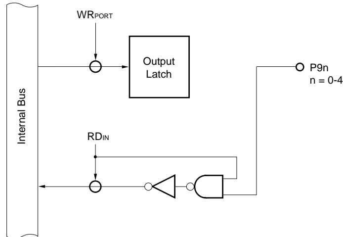
Figure 5-56. Port in Input Port Mode
