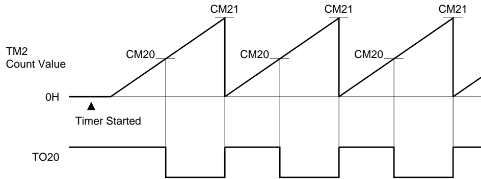
Figure 10-35. Example of Timer/Counter 2 PPG Signal Output
