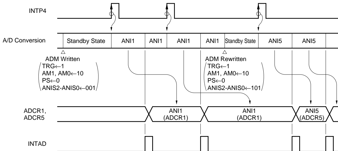
Figure 13-14. A/D Conversion in Select Mode (1-buffer mode) Started by Hardware
