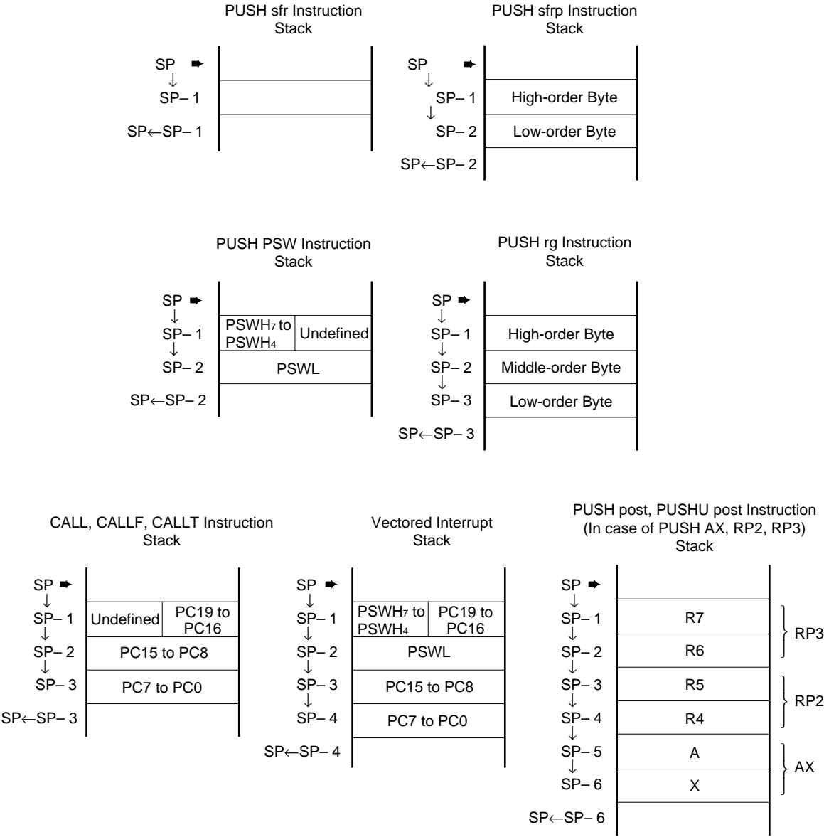
Figure 3-8. Data Saved to Stack Area
