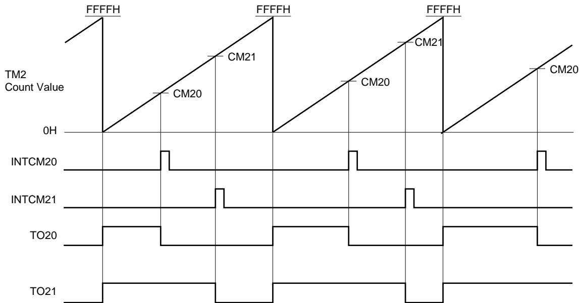
Figure 10-14. Example of PWM Output Using TM2
