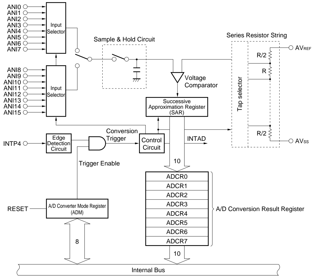
Figure 13-1. Block Diagram of A/D Converter
