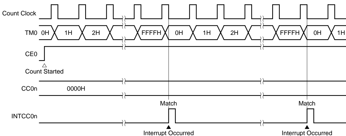
Figure 8-22. Operation When Compare Register (CC00 to CC03) Is Set to 0000H
