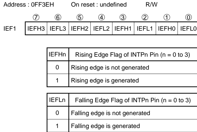
Figure 15-3. Format of Interrupt Valid Edge Flag Register 1 (IEF1)
