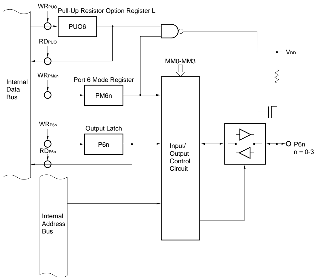
Figure 5-43. Block Diagram of Port 6
