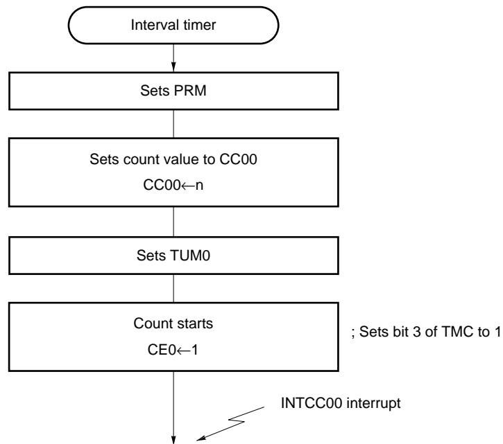
Figure 8-15. Setting Procedure of Interval Timer Operation
