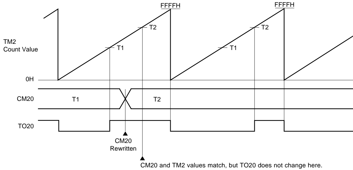
Figure 10-16. Example of Compare Register (CM20) Rewrite
