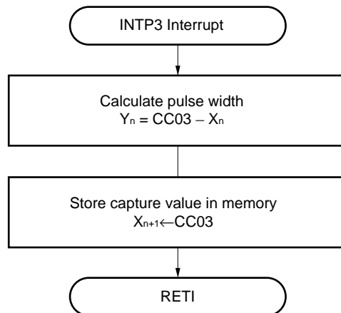
Figure 8-20. Interrupt Request Processing that Calculates Pulse Width
