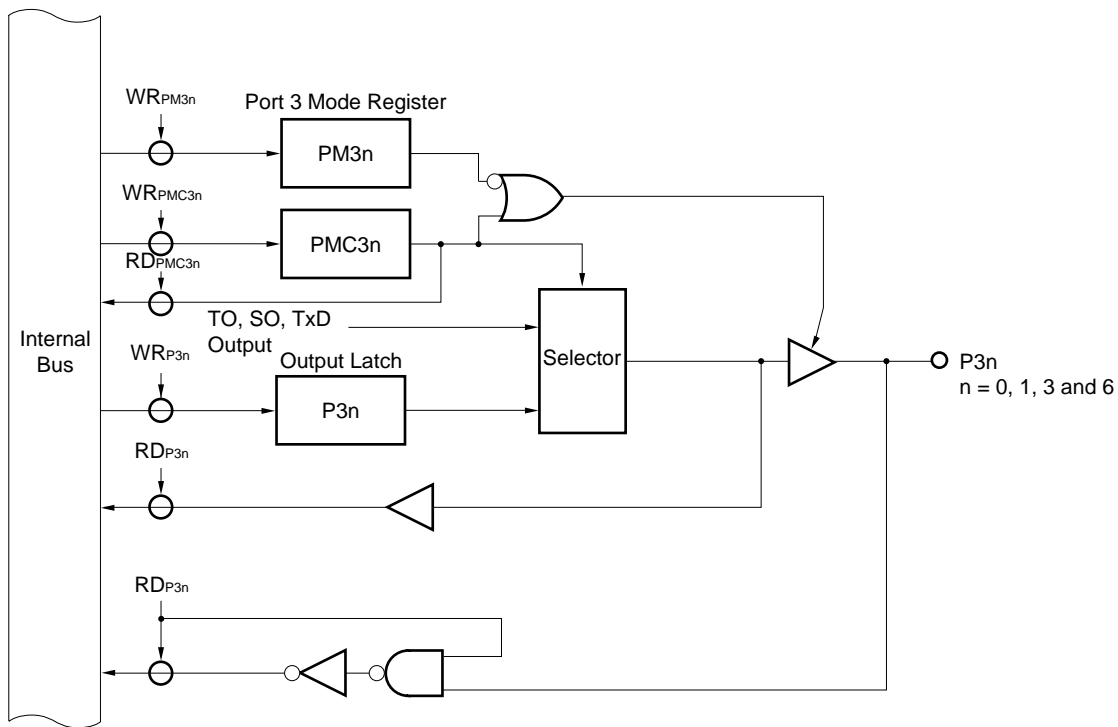
Figure 5-23. Block Diagram of P30, P31, P33 and P36 (Port 3)
