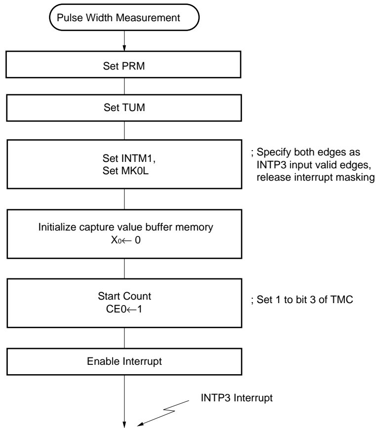
Figure 8-19. Pulse Width Measurement Setting Procedure
