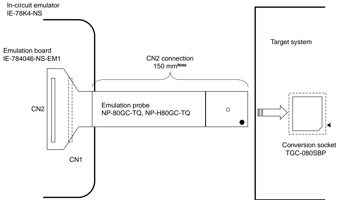
Figure A-2. Distance Between In-Circuit Emulator and Conversion Socket
