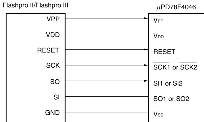
Figure 20-2. Connecting Flashpro II/Flashpro III in 3-Wire Serial I/O Mode
