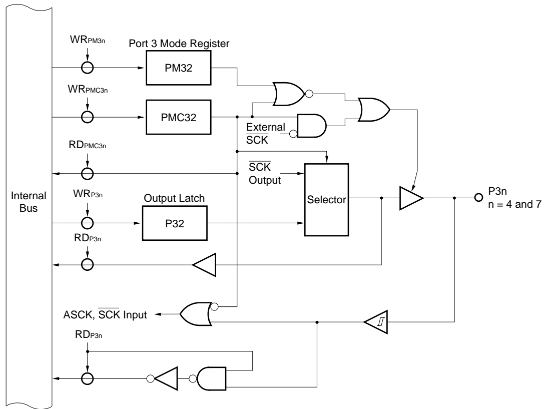
Figure 5-25. Block Diagram of P34 and P37 (Port 3)
