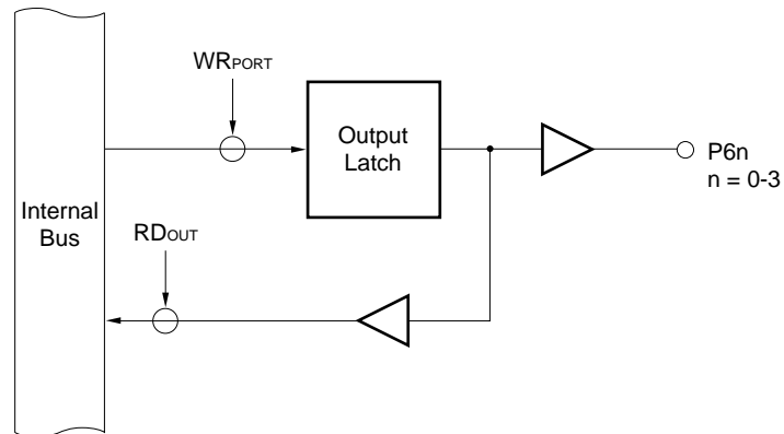
Figure 5-45. Port Specified as Output Port
