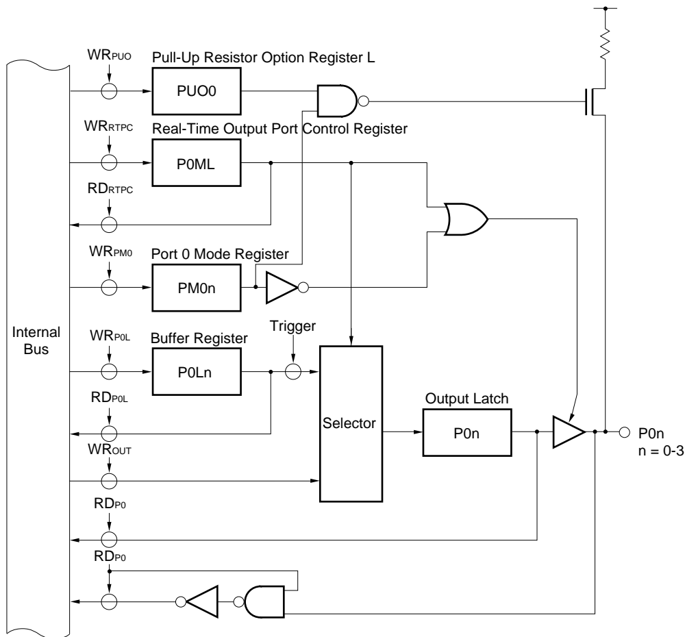
Figure 5-2. Block Diagram of Port 0
