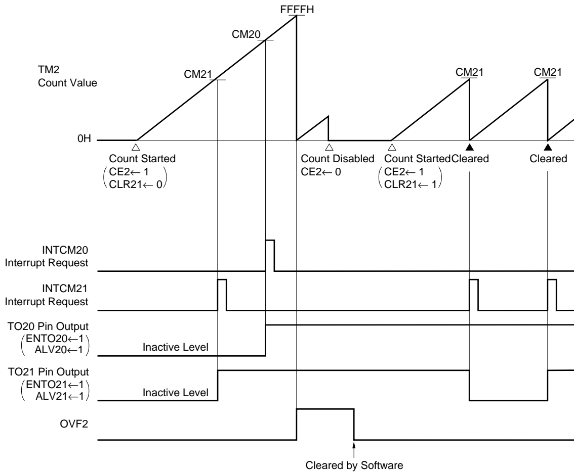
Figure 10-11. TM2 Clearance after Match Detection
