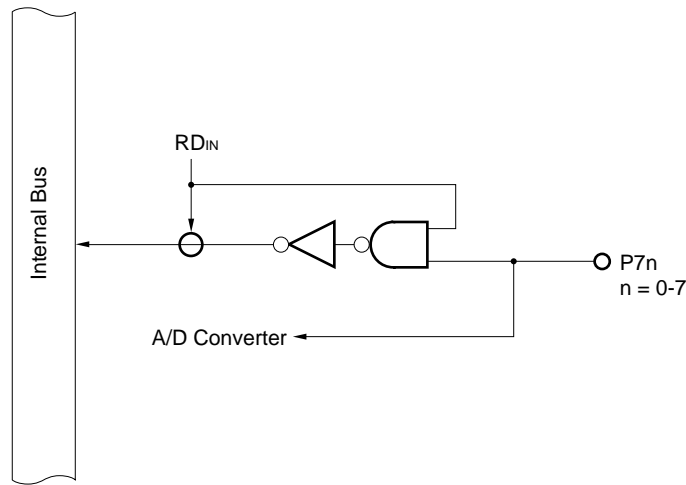
Figure 5-49. Block Diagram of Port 7
