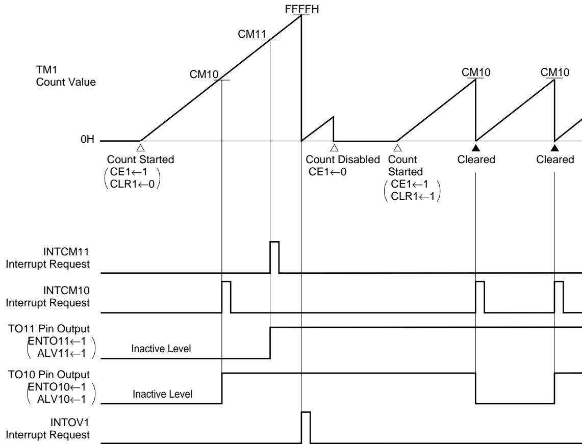
Figure 9-10. Clearing TM1 after Detection of Match
