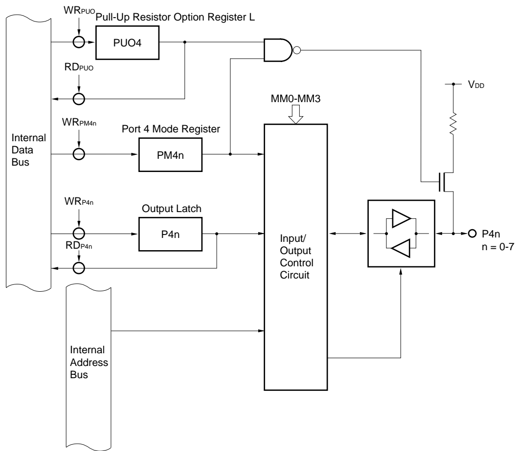
Figure 5-31. Block Diagram of Port 4
