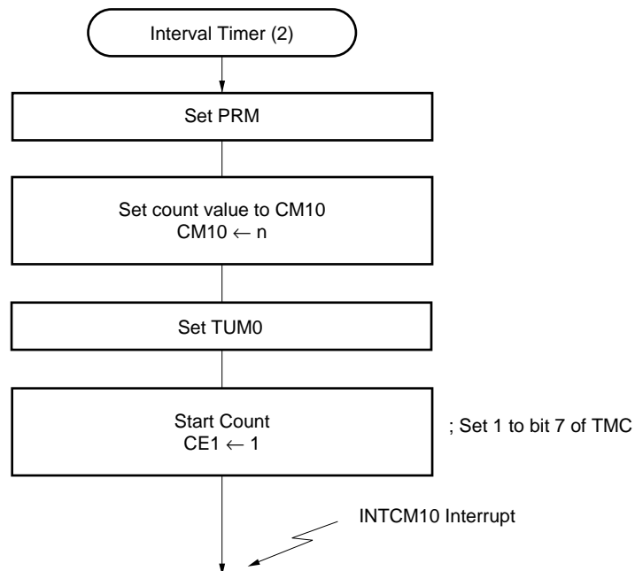
Figure 9-20. Setting Procedure of Interval Timer Operation (2)
