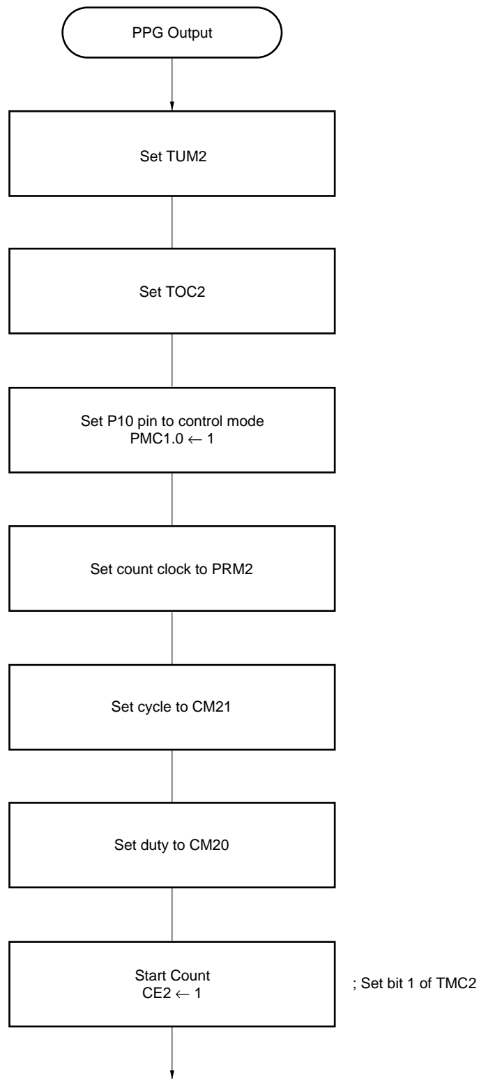
Figure 10-37. Setting Procedure of PPG Output
