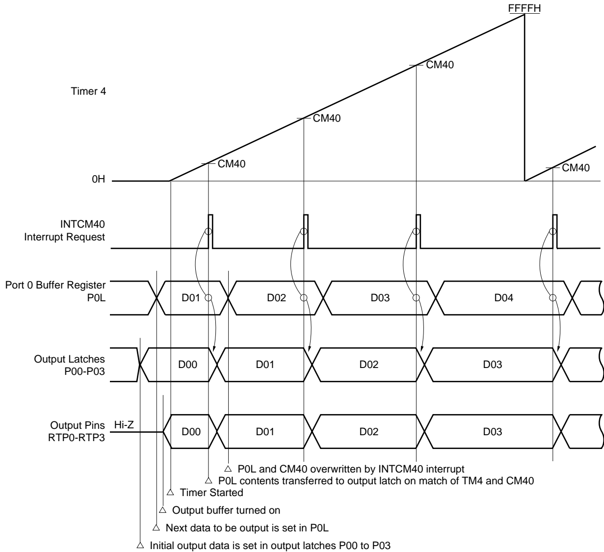
Figure 6-4. Operation Timing of Real-Time Output Port
