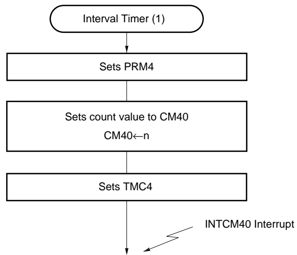
Figure 11-11. Setting Procedure of Interval Timer Operation (1)
