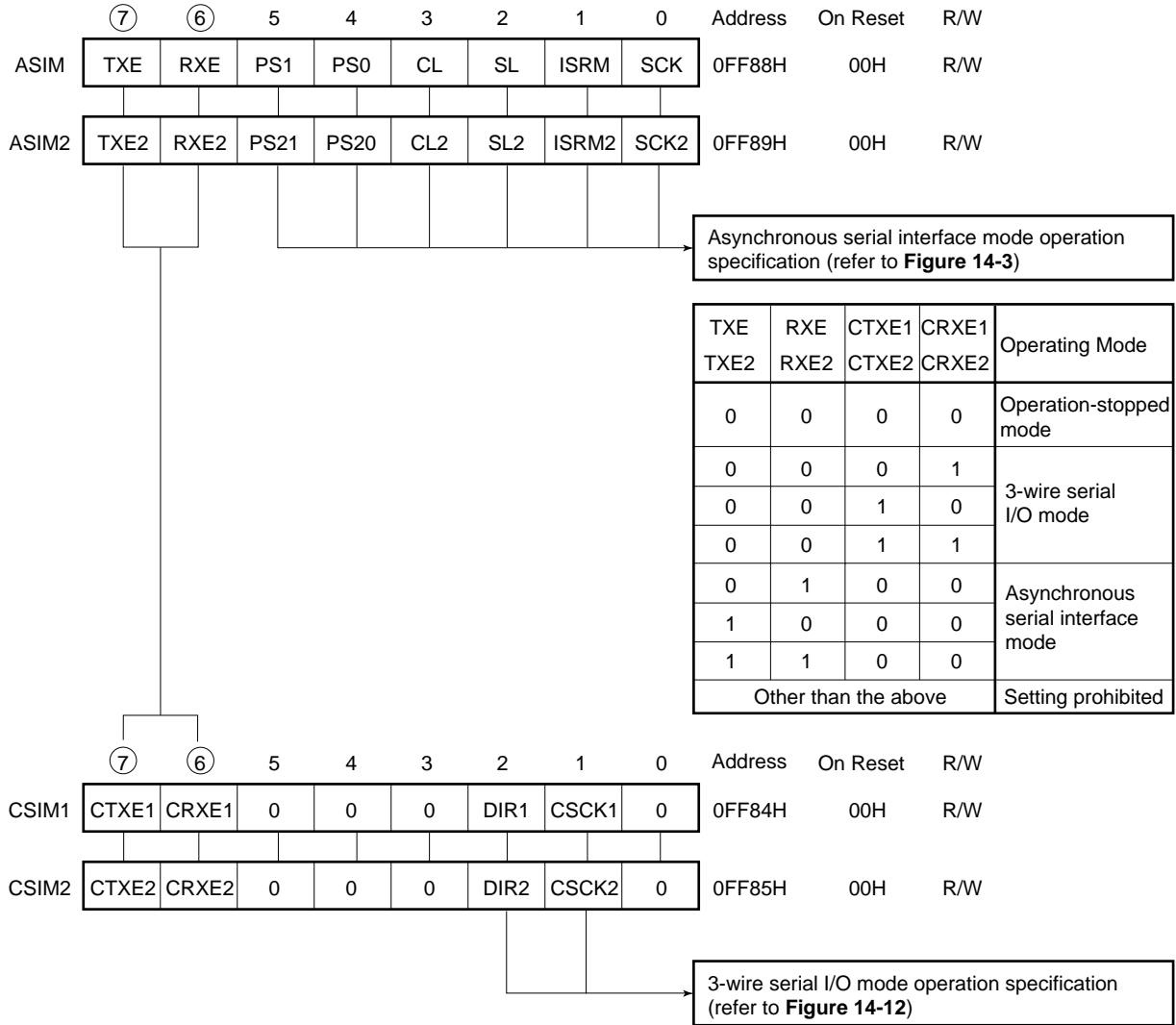
Figure 14-1. Switching Between Asynchronous Serial Interface Mode and 3-Wire Serial I/O Mode
