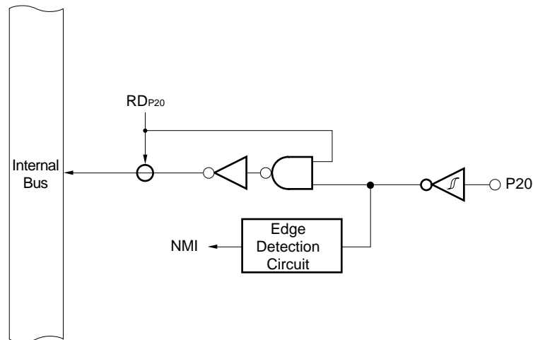
Figure 5-15. Block Diagram of P20 (Port 2)
