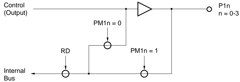
Figure 5-14. Control Specification
