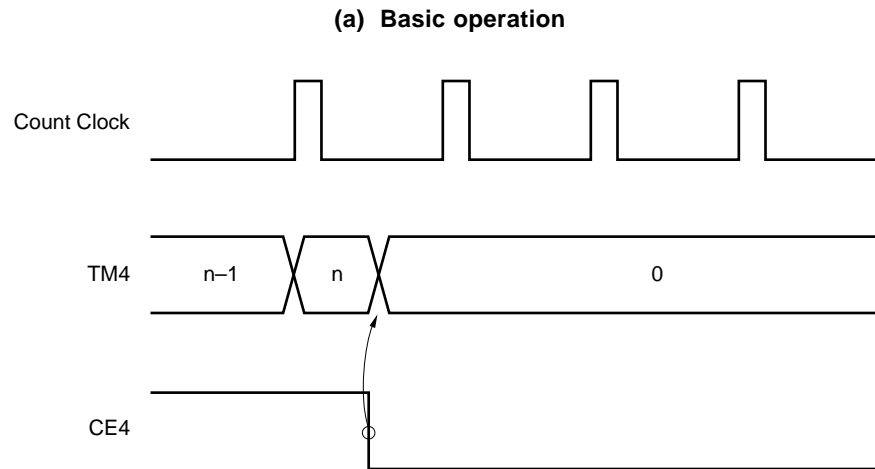
Figure 11-6. Clear Operation of TM4 When CE4 Bit is Cleared (0)
