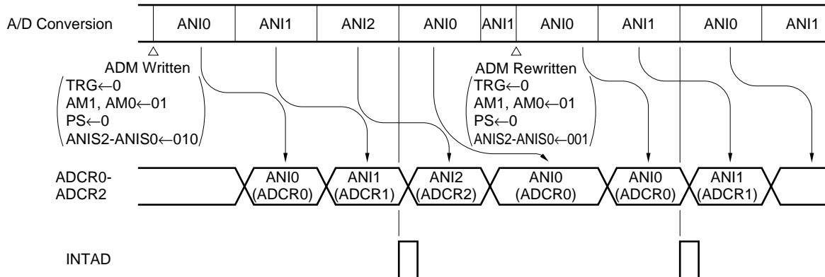
Figure 13-13. A/D Conversion in Scan Mode Started by Software
