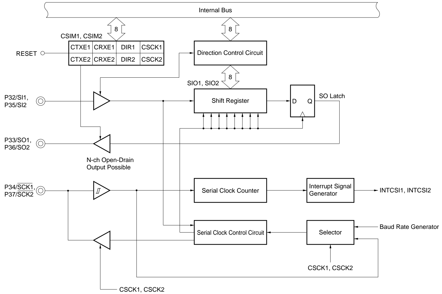
Figure 14-11. Block Diagram of 3-Wire Serial I/O Mode
