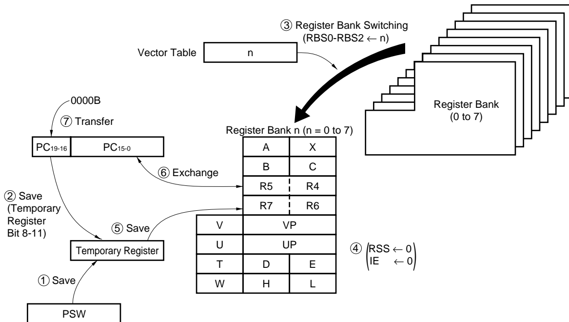
Figure 16-11. Context Switching Operation by Generation of an Interrupt Request
