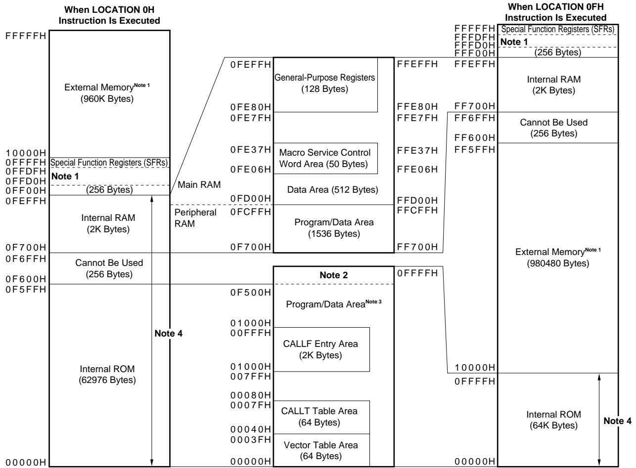
Figure 3-2. \mu PD784046 Memory Map
