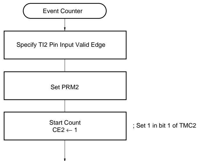
Figure 10-41. Setting Procedure of External Event Counter Operation
