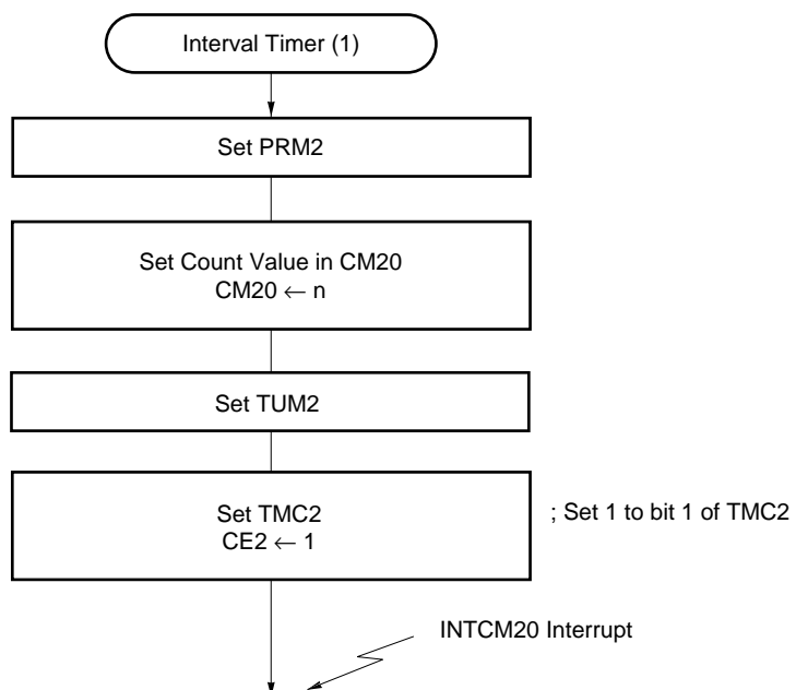
Figure 10-26. Setting Procedure of Interval Timer Operation (1)
