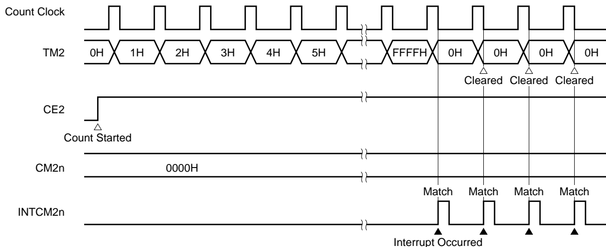
Figure 10-43. Operation When Compare Register (CM20, CM21) Is Set to 0000H
