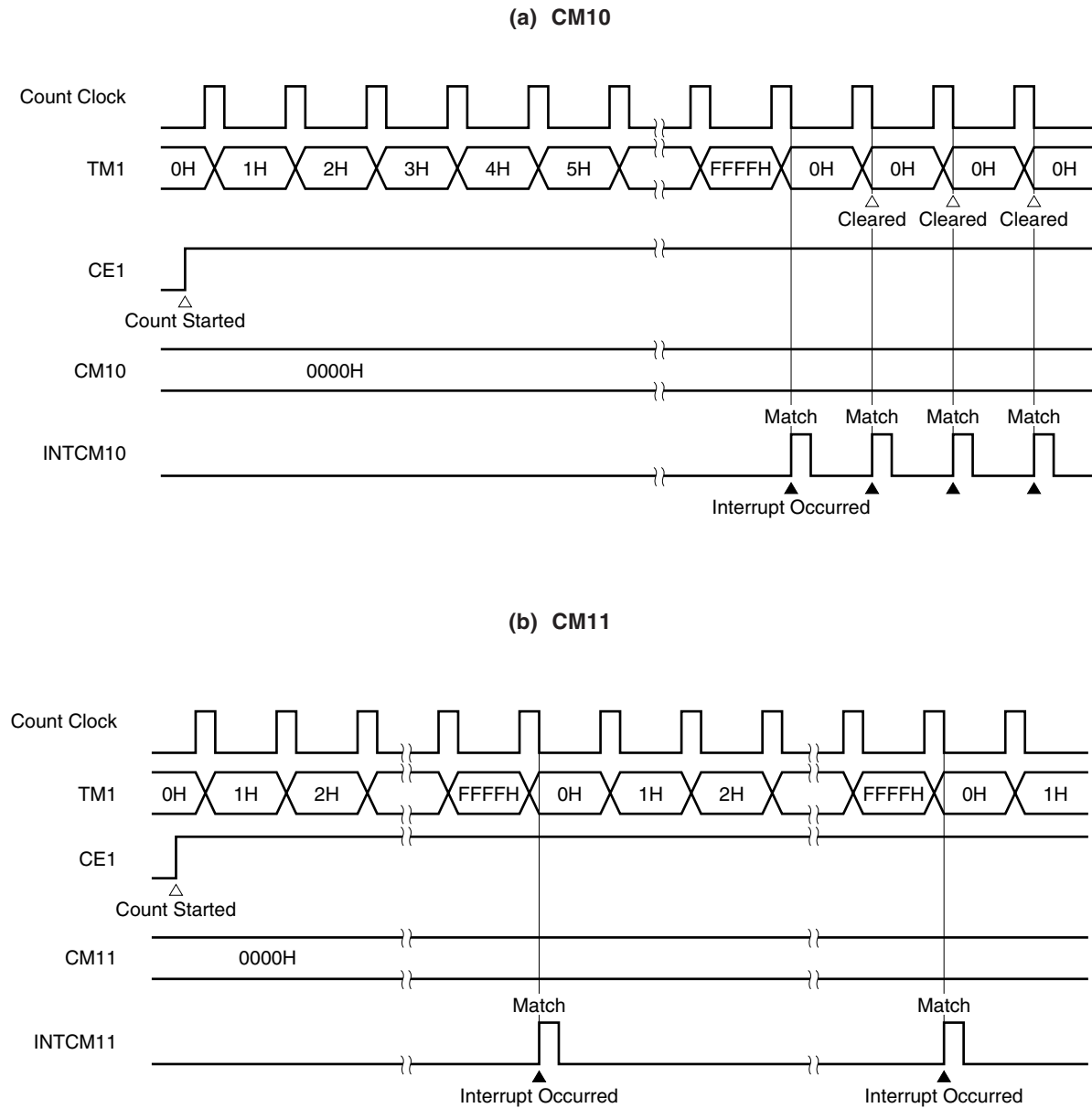
Figure 9-22. Operation When Compare Register (CM10, CM11) Is Set to 0000H
