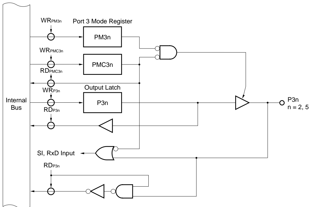
Figure 5-24. Block Diagram of P32 and P35 (Port 3)
