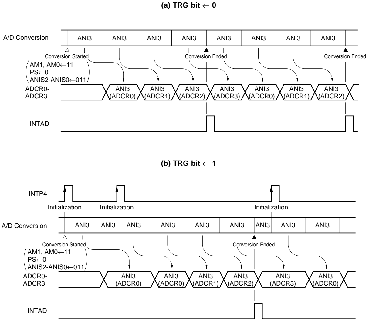
Figure 13-9. Operation Timing in Select Mode (4-buffer mode)
