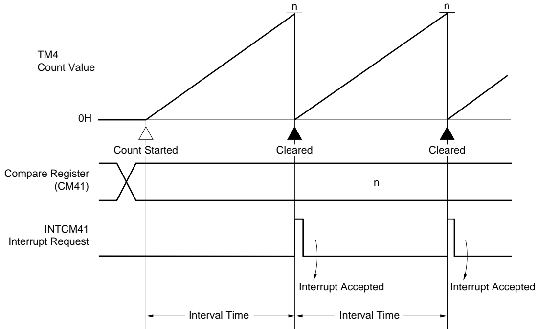
Figure 11-13. Timing of Interval Timer Operation (2)
