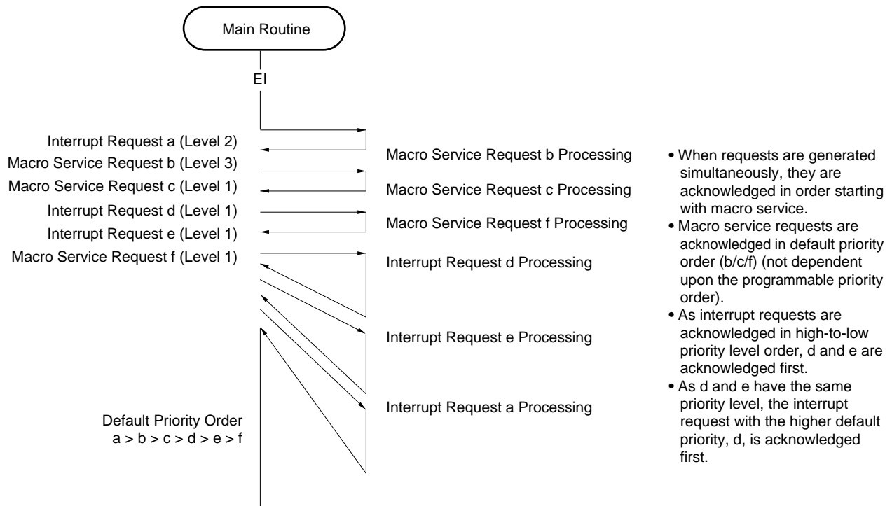
Figure 16-14. Examples of Processing of Simultaneously Generated Interrupts
