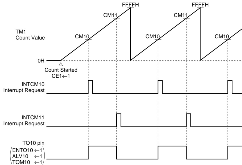
Figure 9-13. Operation of Set/Reset Output (timer 1)
