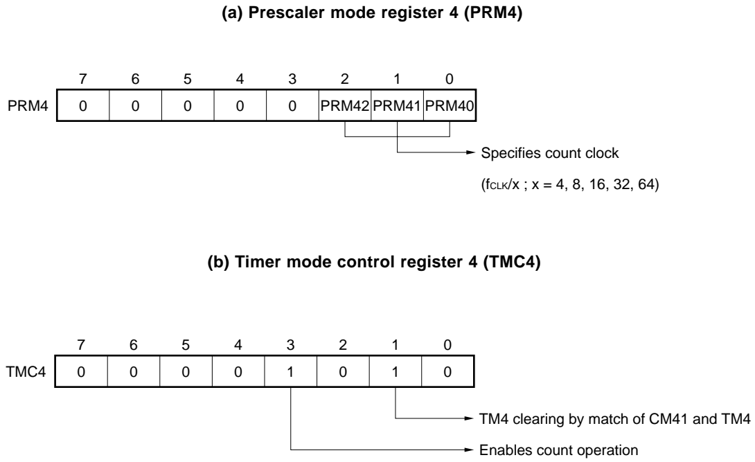
Figure 11-14. Set Contents of Control Register for Interval Timer Operation (2)
