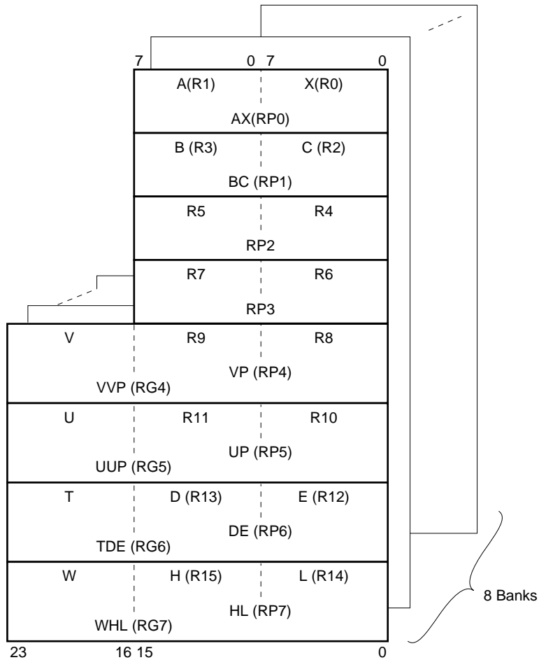
Figure 3-10. Format of General-Purpose Register
