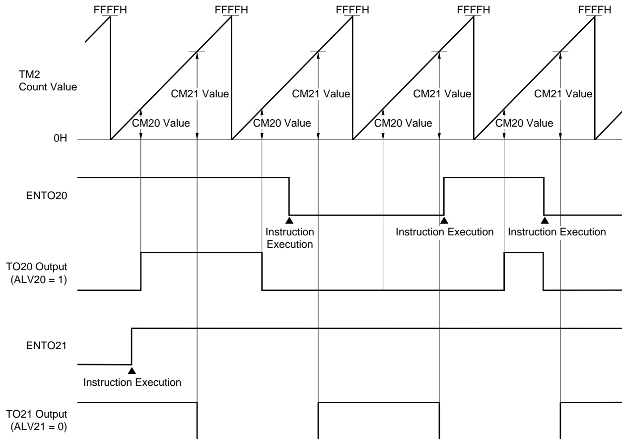
Figure 10-12. Operation of Toggle Output
