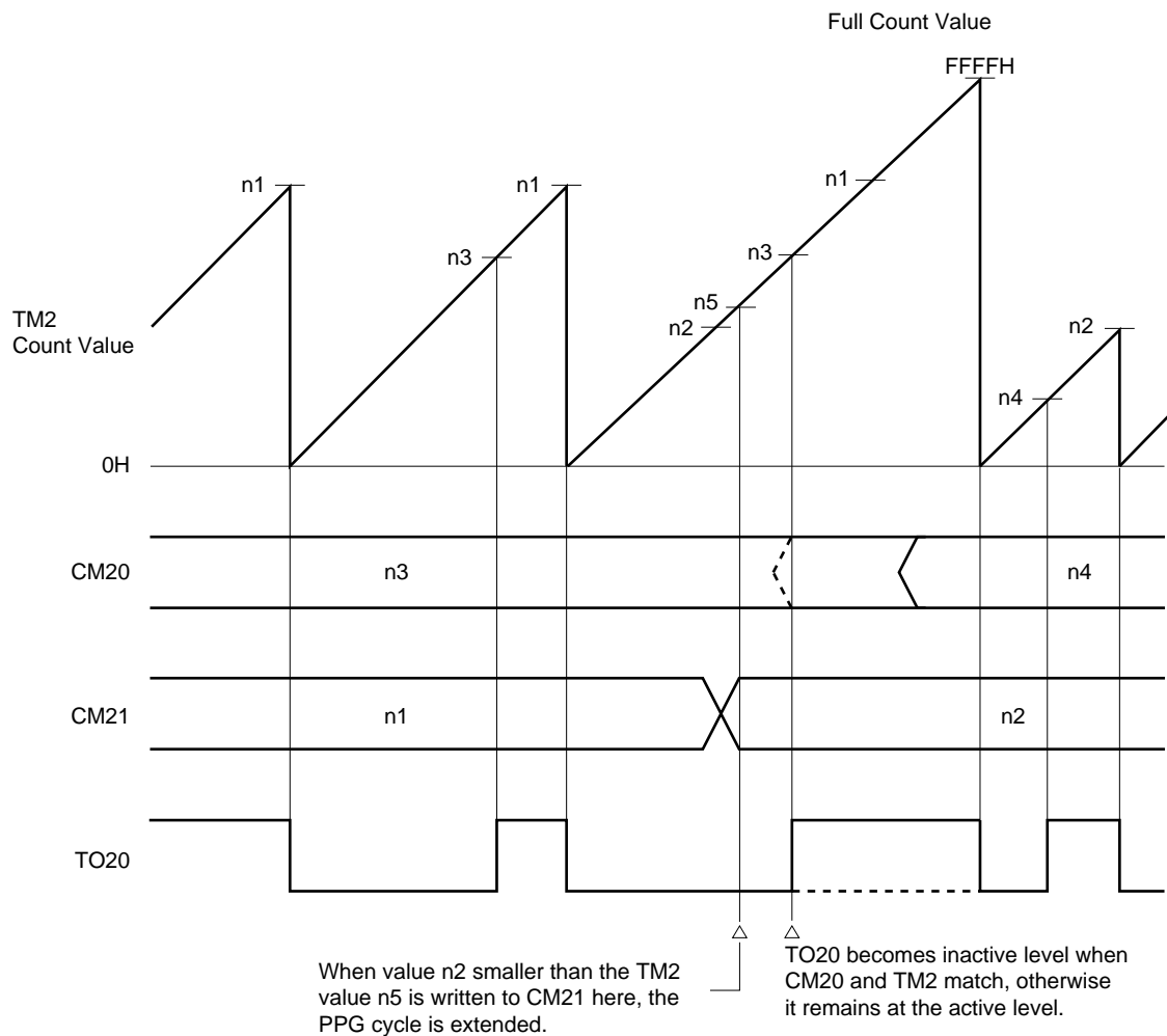
Figure 10-22. Example of Extended PPG Output Cycle
