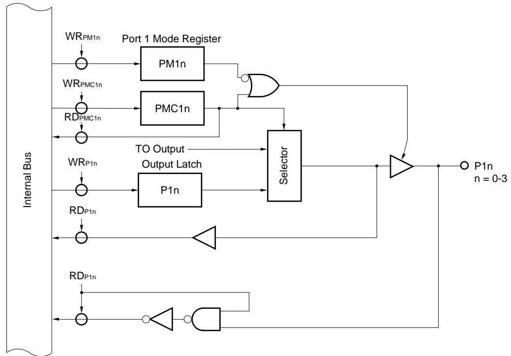
Figure 5-9. Block Diagram of Port 1
