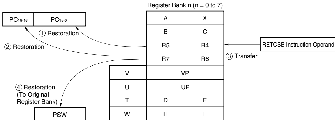
Figure 16-8. Return from BRKCS Instruction Software Interrupt (RETCSB Instruction Operation)
