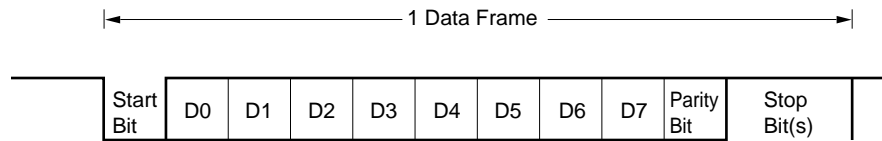
Figure 14-5. Data Format of Asynchronous Serial Interface Transmit/Receive
