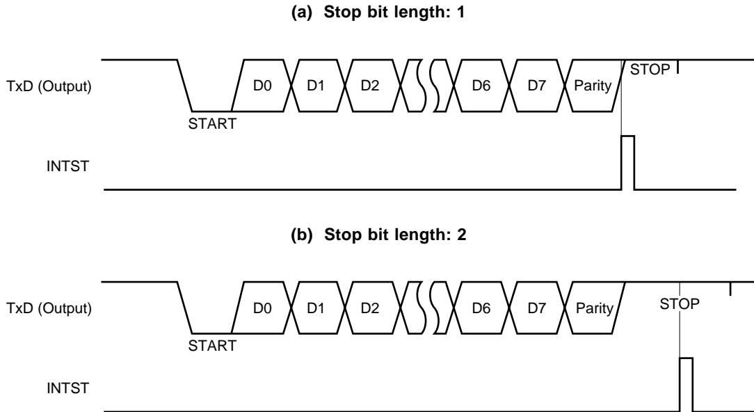
Figure 14-6. Interrupt Timing of Asynchronous Serial Interface Transmission Completion
