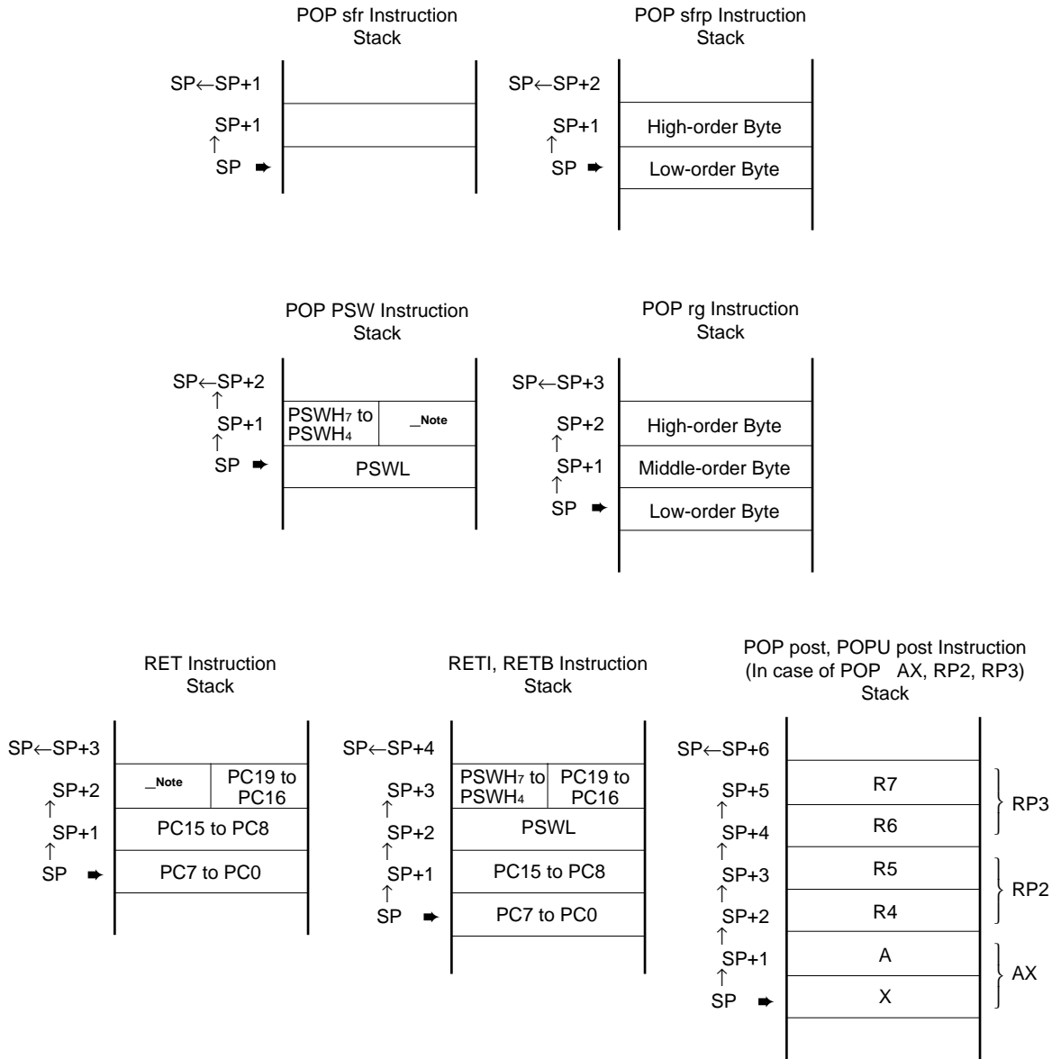
Figure 3-9. Data Restored from Stack Area
