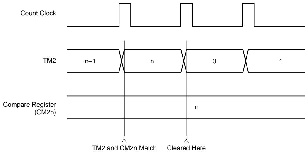
Figure 10-7. TM2 Clear Operation by Match With Compare Register (CM20/CM21)
