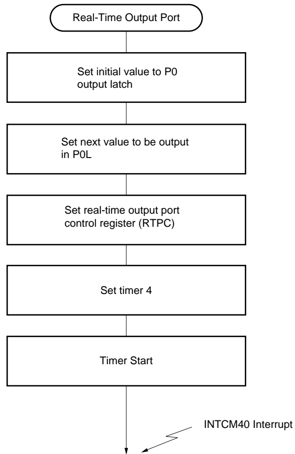
Figure 6-6. Setting Procedure of Real-Time Output Function
