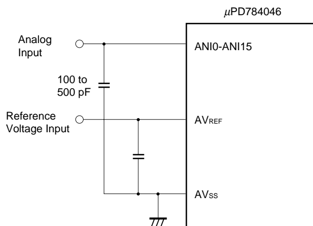
Figure 13-17. Example of Capacitor Connection on A/D Converter Pins
