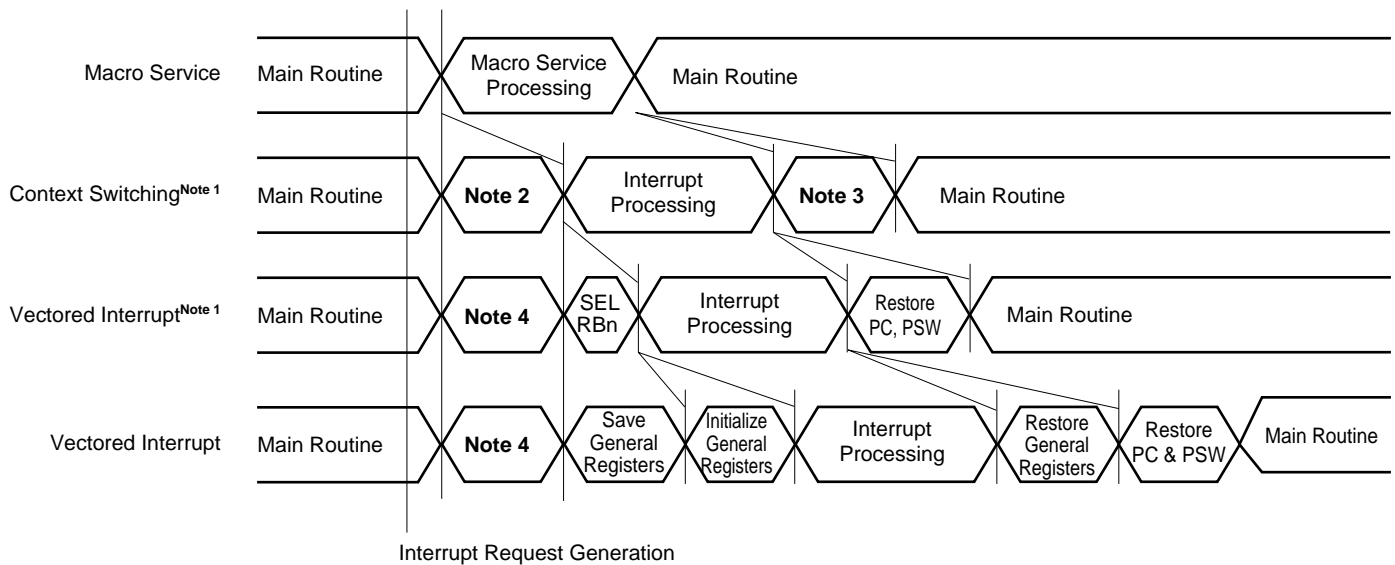
Figure 16-16. Differences between Vectored Interrupt and Macro Service Processing
