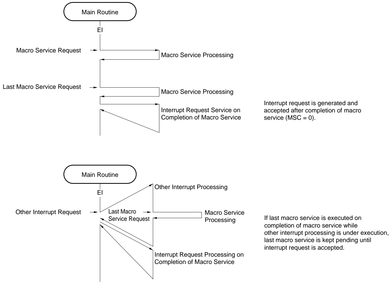
Figure 16-18. Operation on Completion of Macro Service
