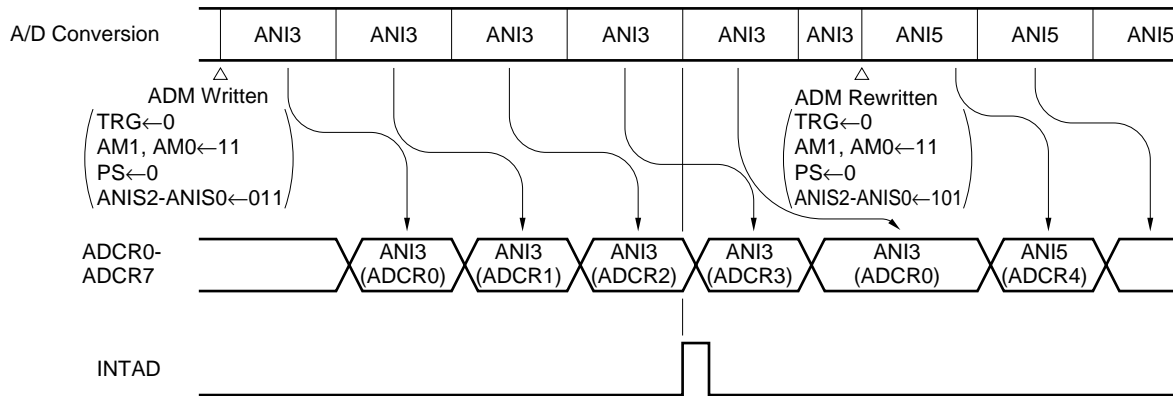
Figure 13-12. A/D Conversion in Select Mode (4-buffer mode) Started by Software
