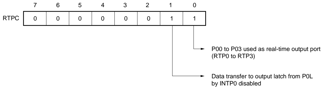
Figure 6-5. Settings for Real-Time Output Function Control Register
