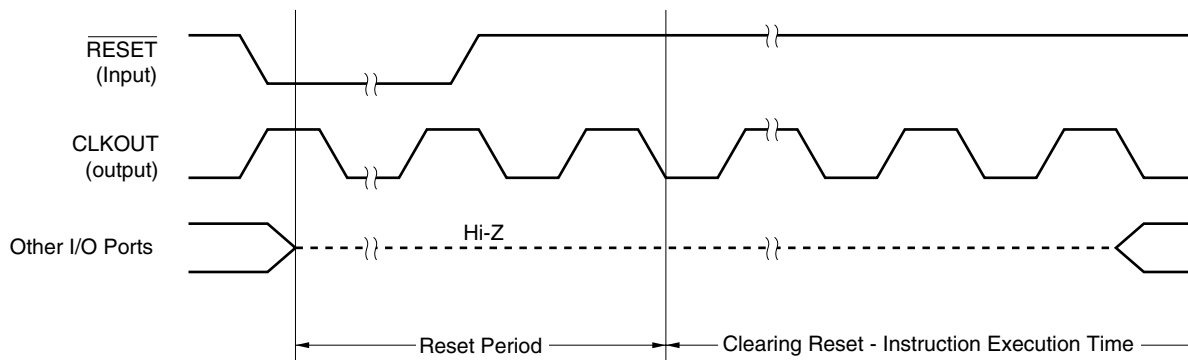
Figure 19-3. Timing on Reset Input
