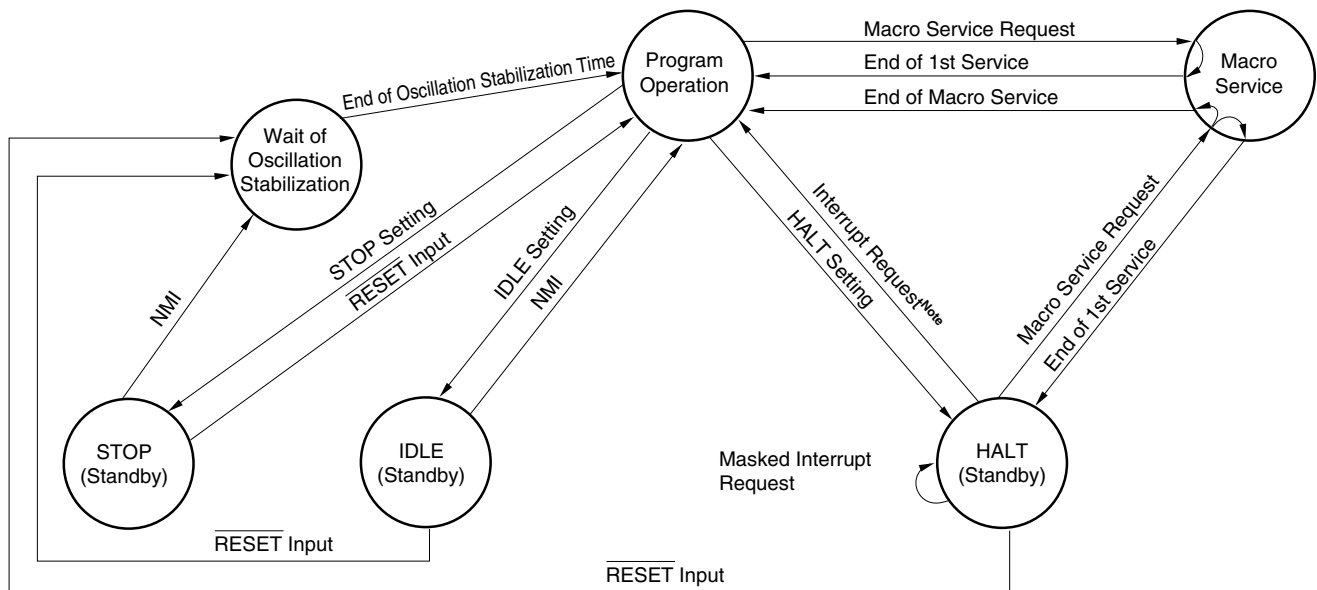
★ Figure 18-1. Diagram of Standby Mode Transition
