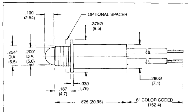
5mm Panel Mount LED Assemblies
