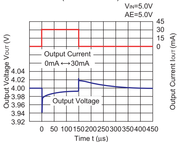
RP200x40xx (Fixed Fast Mode)
