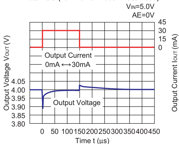
RP200x40xx Auto ECO (Low Power Mode \leftrightarrow Fast Mode)
