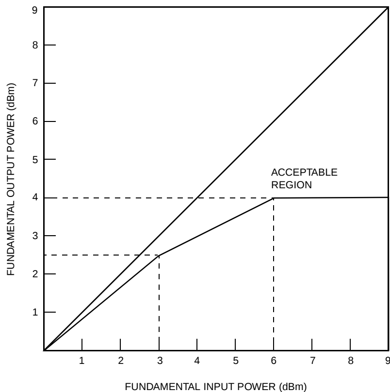
Figure 4. Overload Compression
