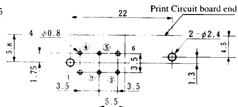
PCB mounting hole layout (Connector mounting side)
