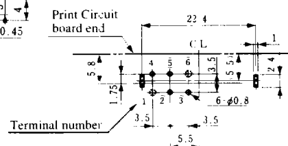
PCB mounting hole layout (Connector mounting side)
