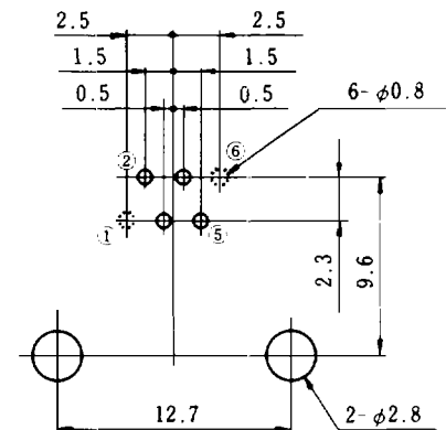
PCB mounting hole layout (Connector mounting side)
