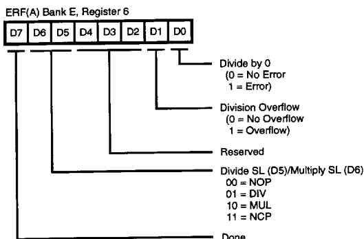
Figure 22. Multiply/Divide Control Register (MDCON)
