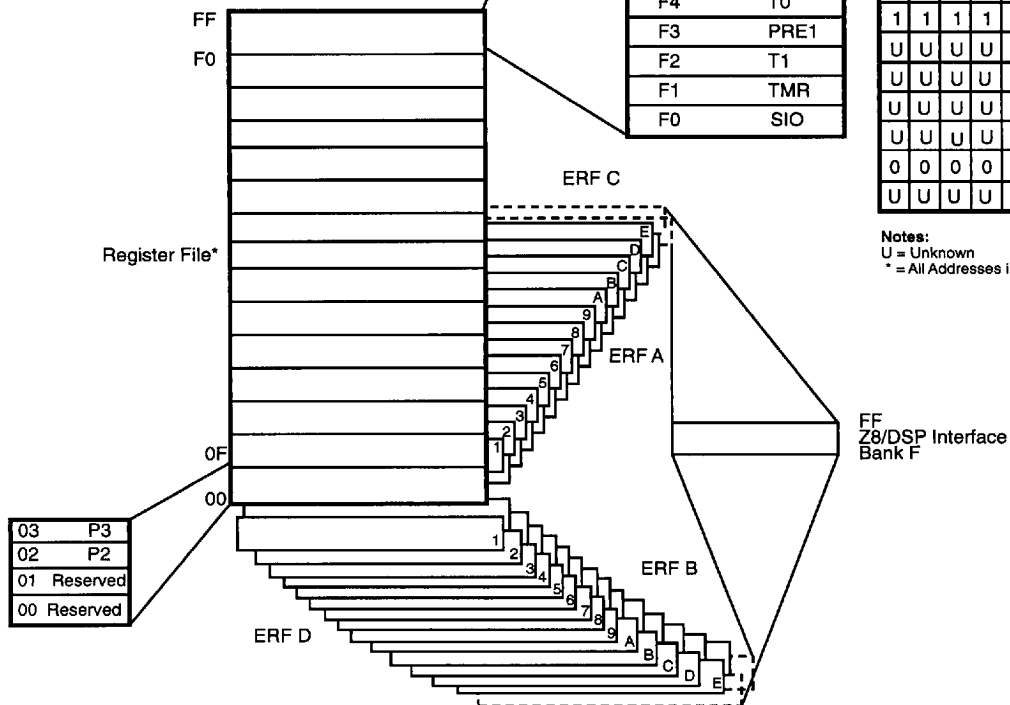
Figure 10. Register File
