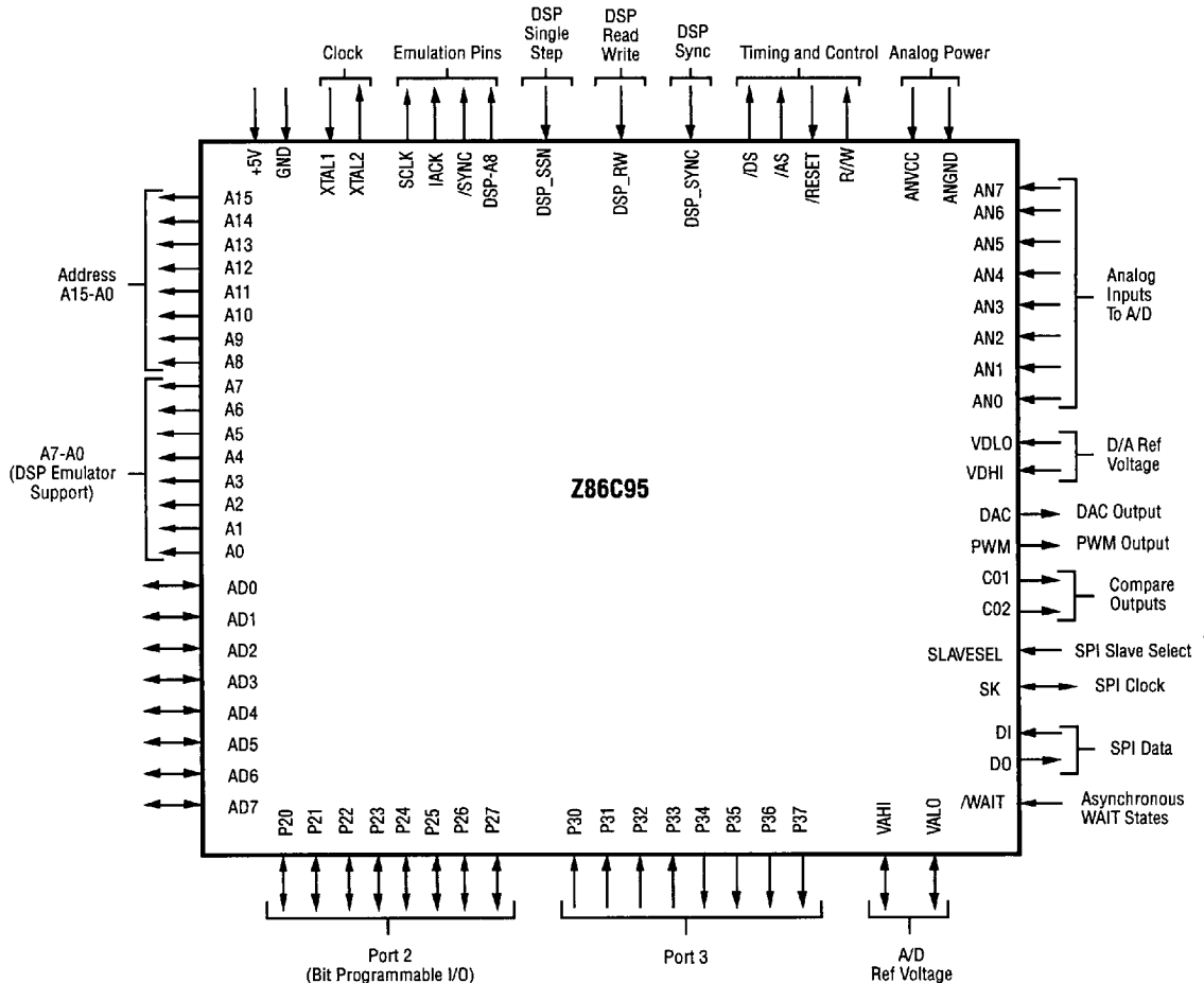
Figure 5. Pin Functions
