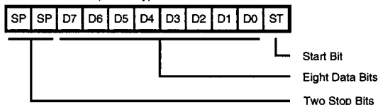
Transmitted Data (No Parity)
