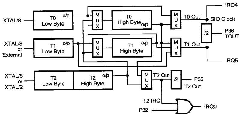
Figure 24. Counter/Timer Block Diagram
