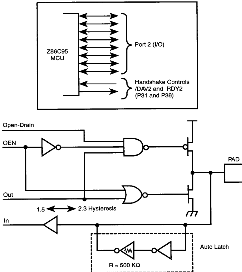
Figure 6. Port 2 Configuration
