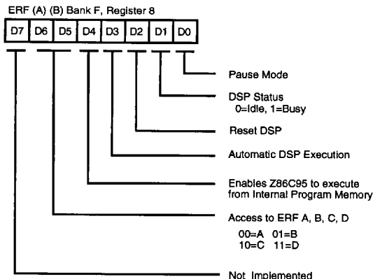
Figure 20. Z8/DSP Control Register
