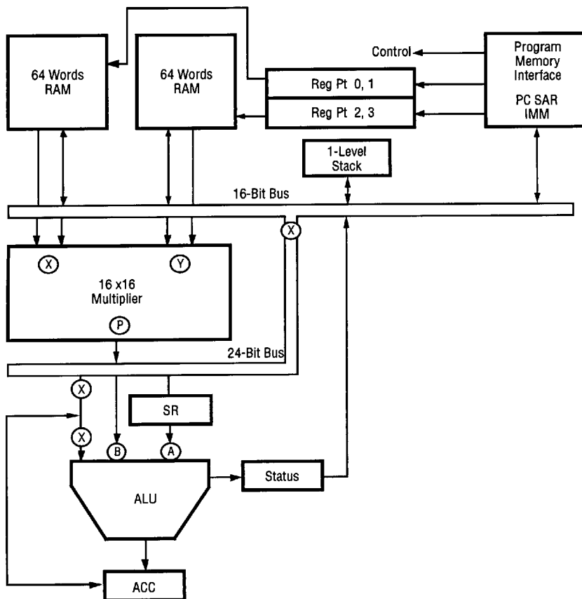
Figure 19. DSP Core
