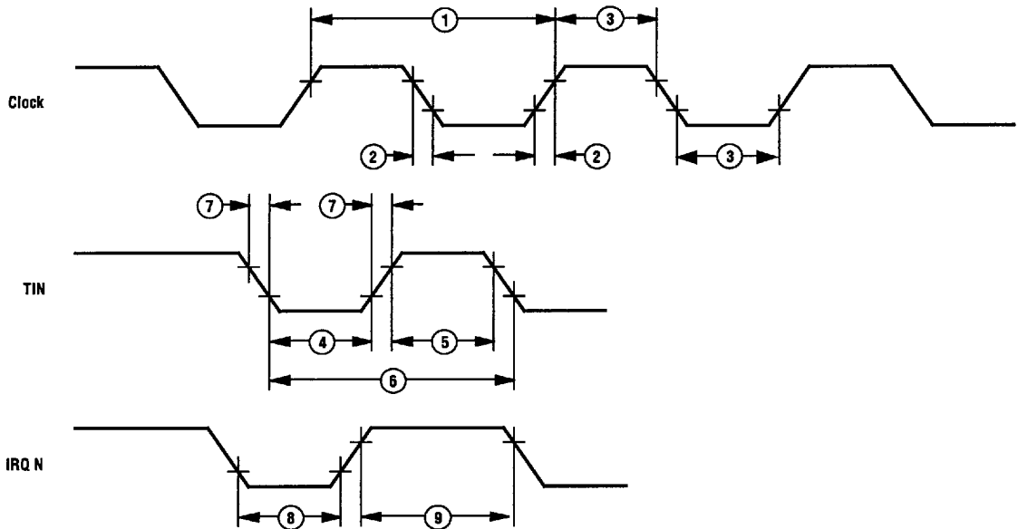
Figure 55. Additional Timing
