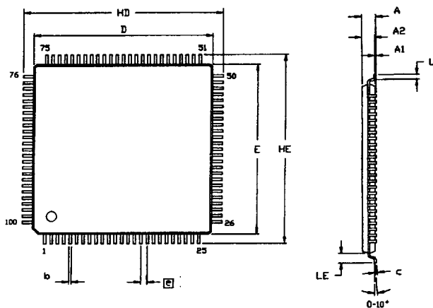
100-Pin VQFP Package Diagram
