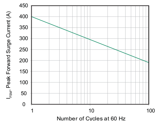
Figure 6 - Maximum Non-Repetitive Forward Surge Current
