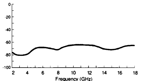
Isolation (dB)
