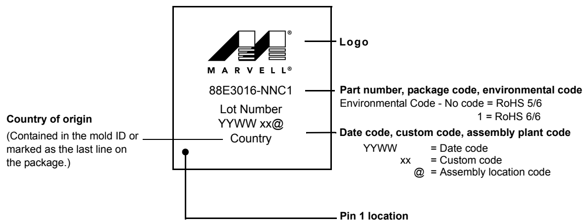
Figure 32: 88E3016 64-pin QFN Commercial RoHS 6/6 Compliant Package Marking and Pin 1 Location
