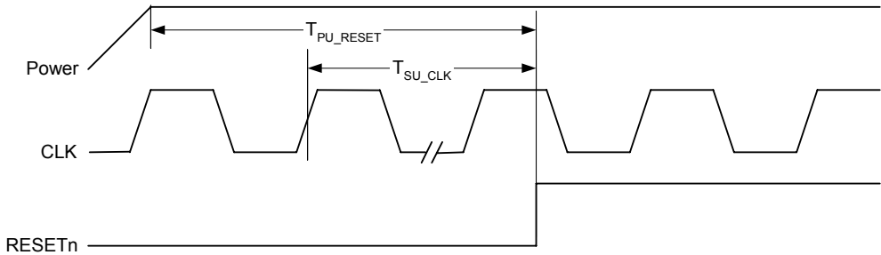
Figure 14: Reset Timing
