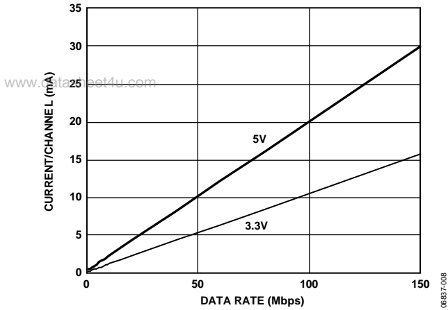
Figure 8. Typical Input Supply Current per Channel vs. Data Rate for 5 V and 3.3 V Operation
